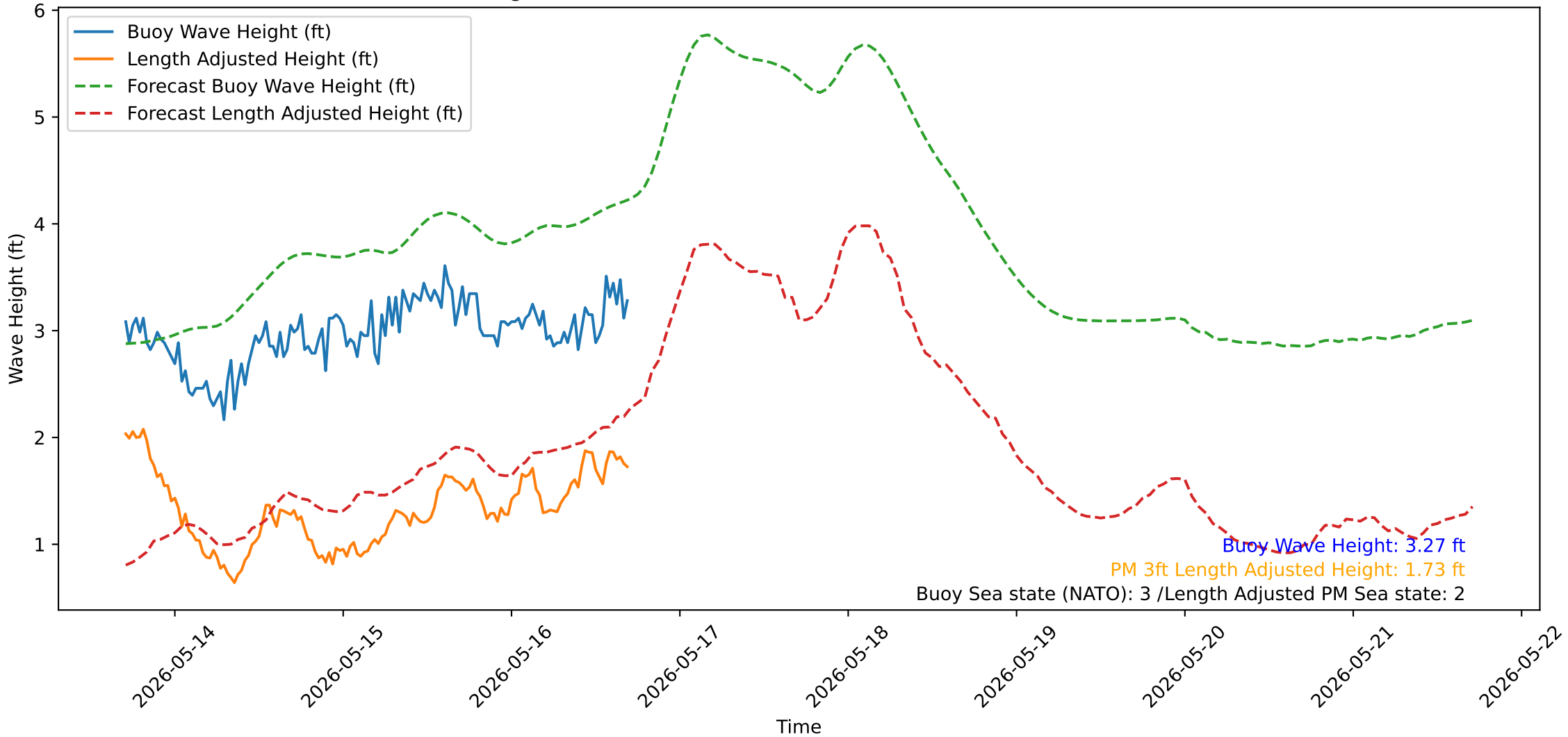
Wave Heights over Time for Oceanside Harbor at 2026-05-16 17:10:31
