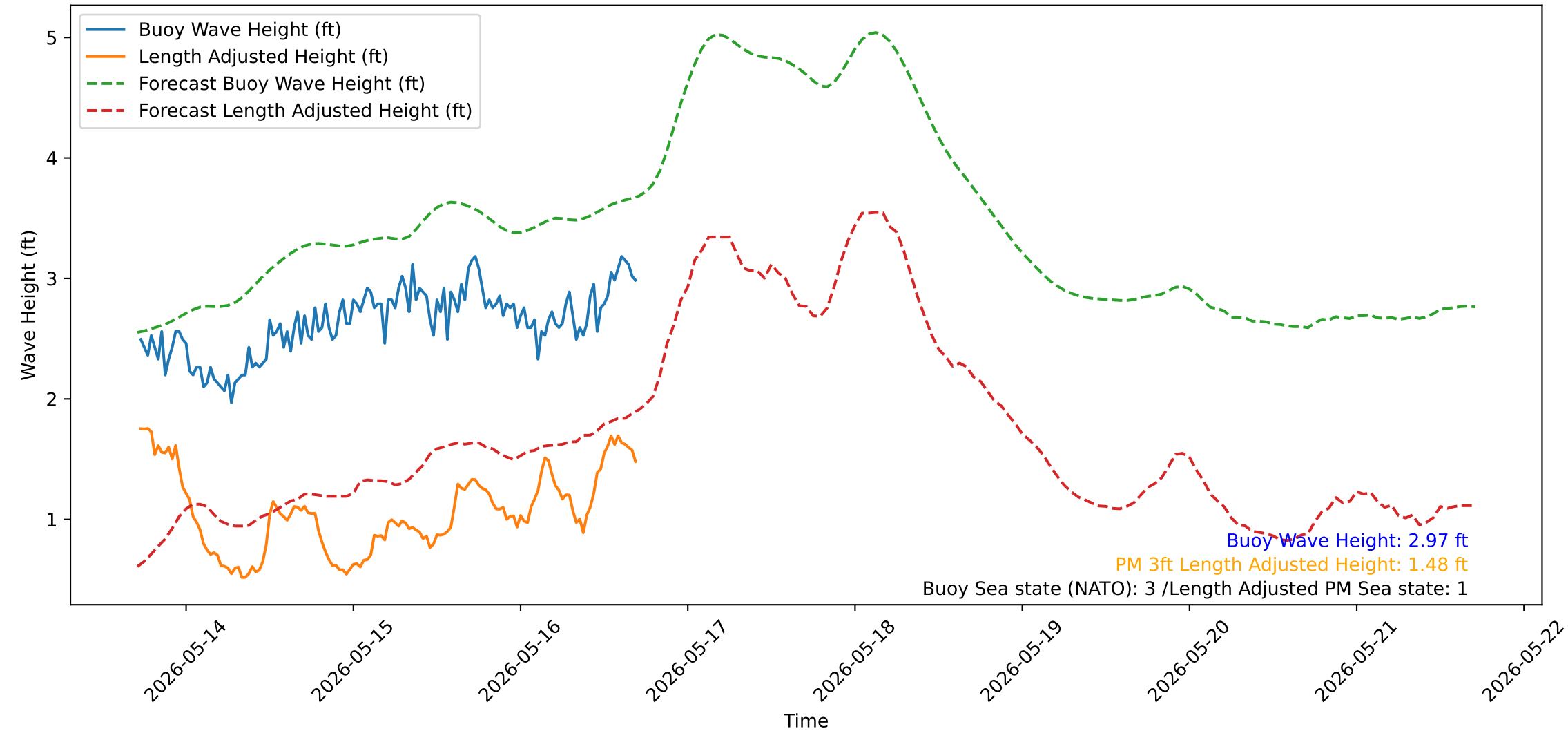
Wave Heights over Time for Red Beach at 2026-05-16 17:10:51
