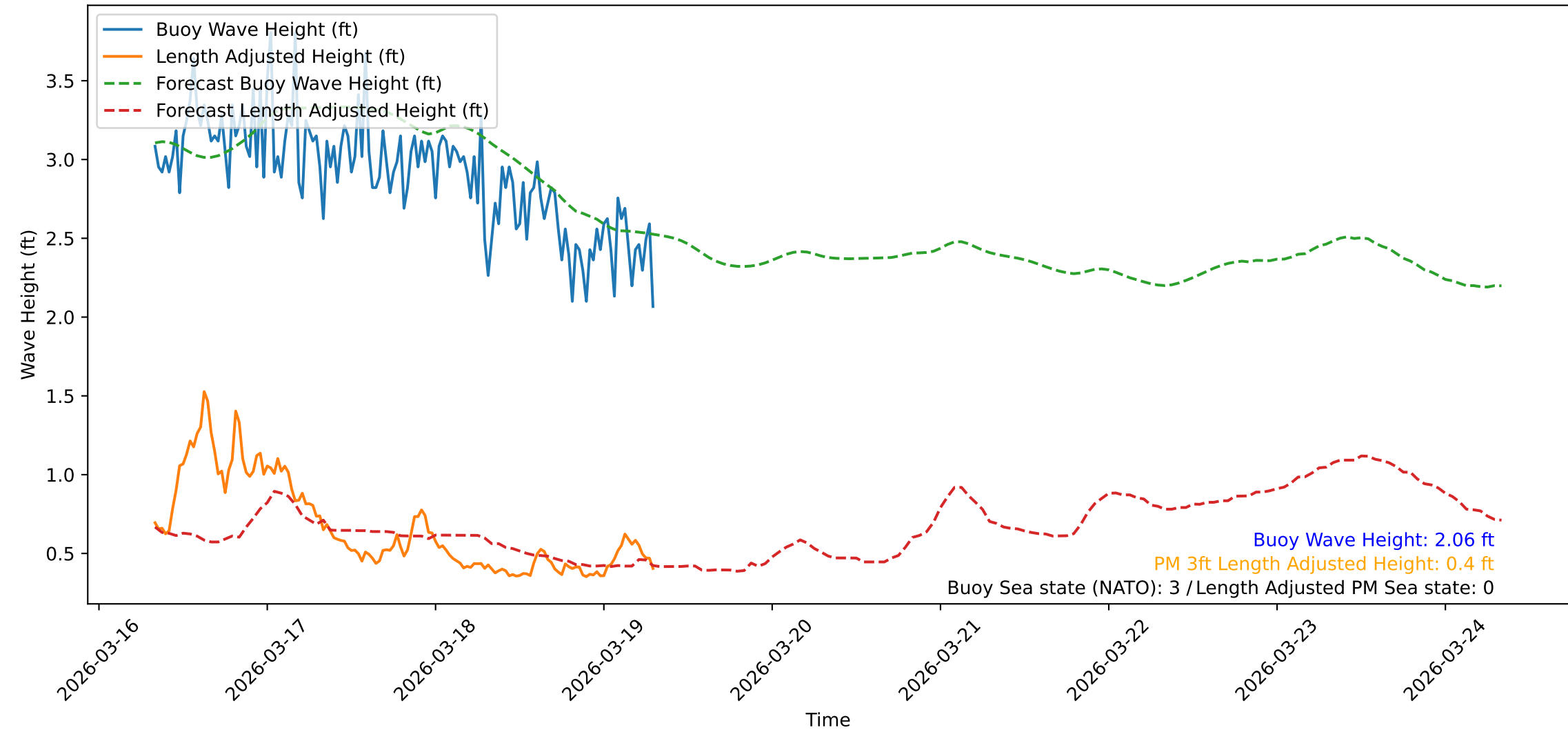
Wave Heights over Time for Red Beach at 2026-03-19 07:40:48
