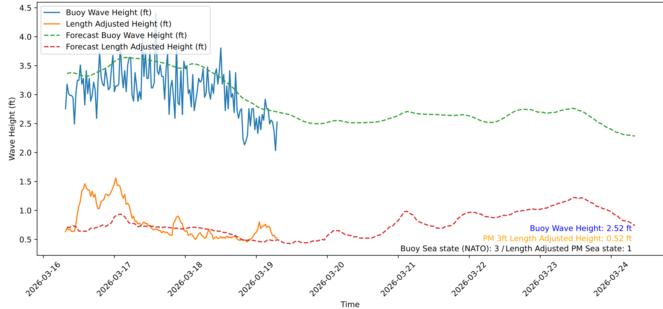
Wave Heights over Time for Oceanside Harbor at 2026-03-19 07:40:32
