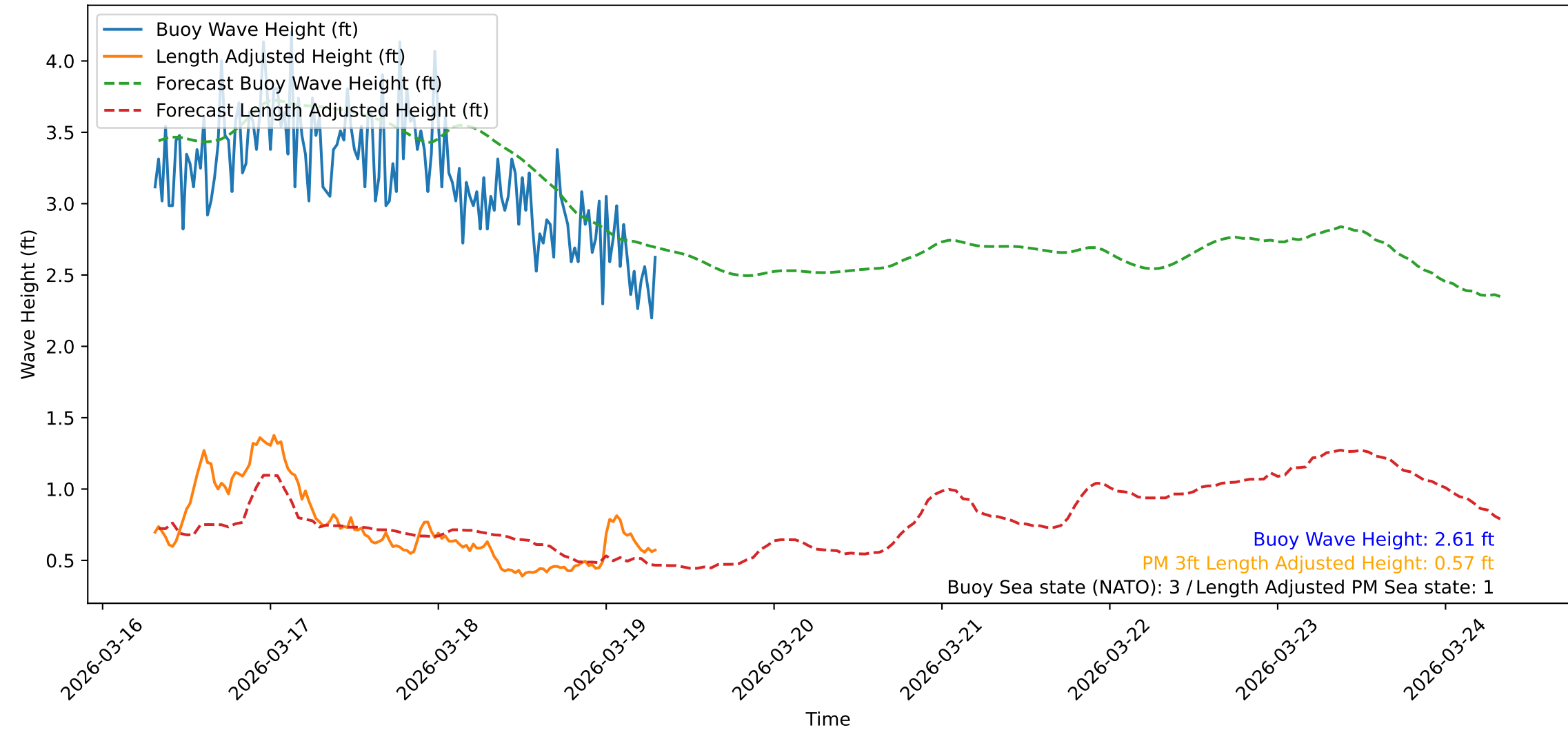
Wave Heights over Time for Green Beach at 2026-03-19 07:41:11
