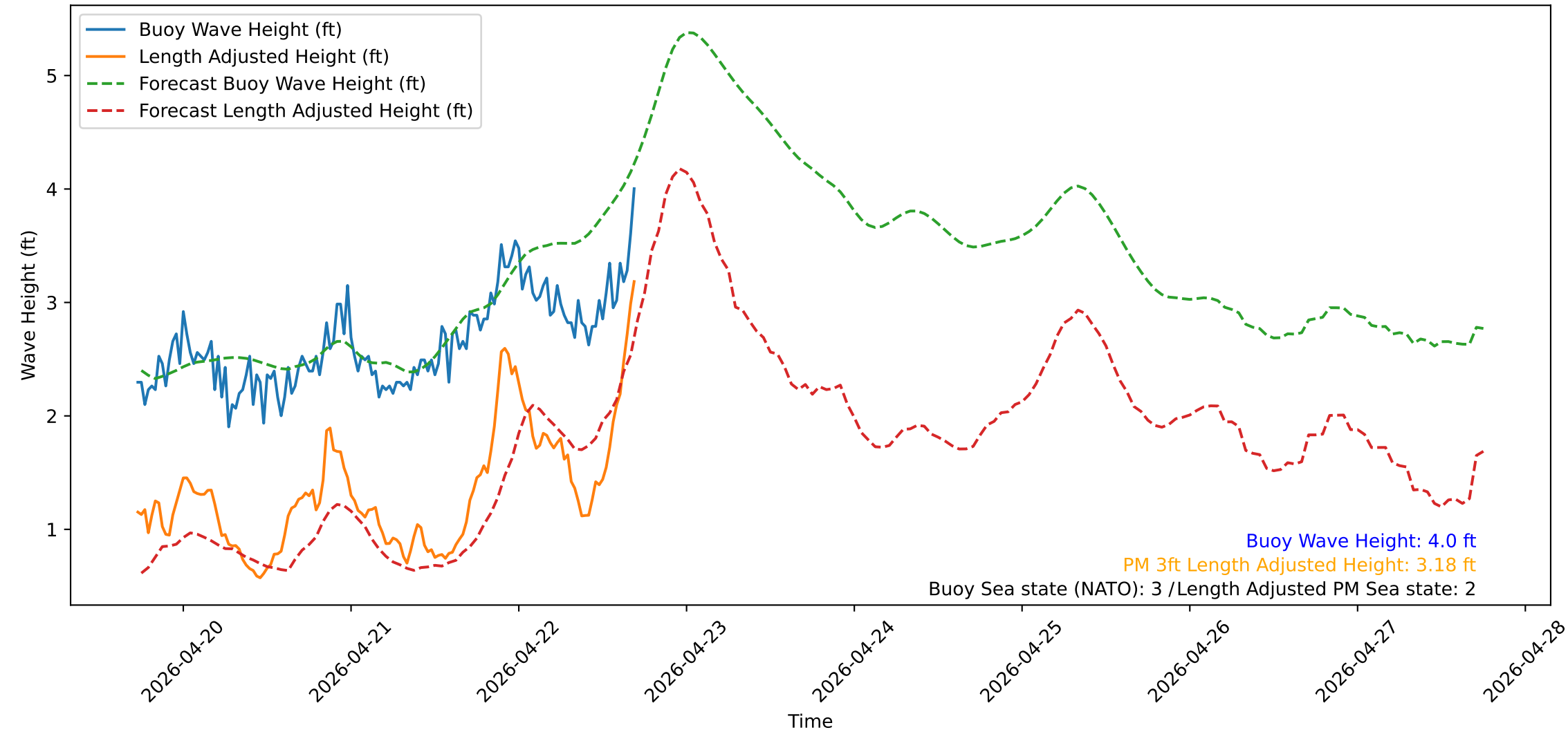
Wave Heights over Time for Green Beach at 2026-04-22 17:31:13
