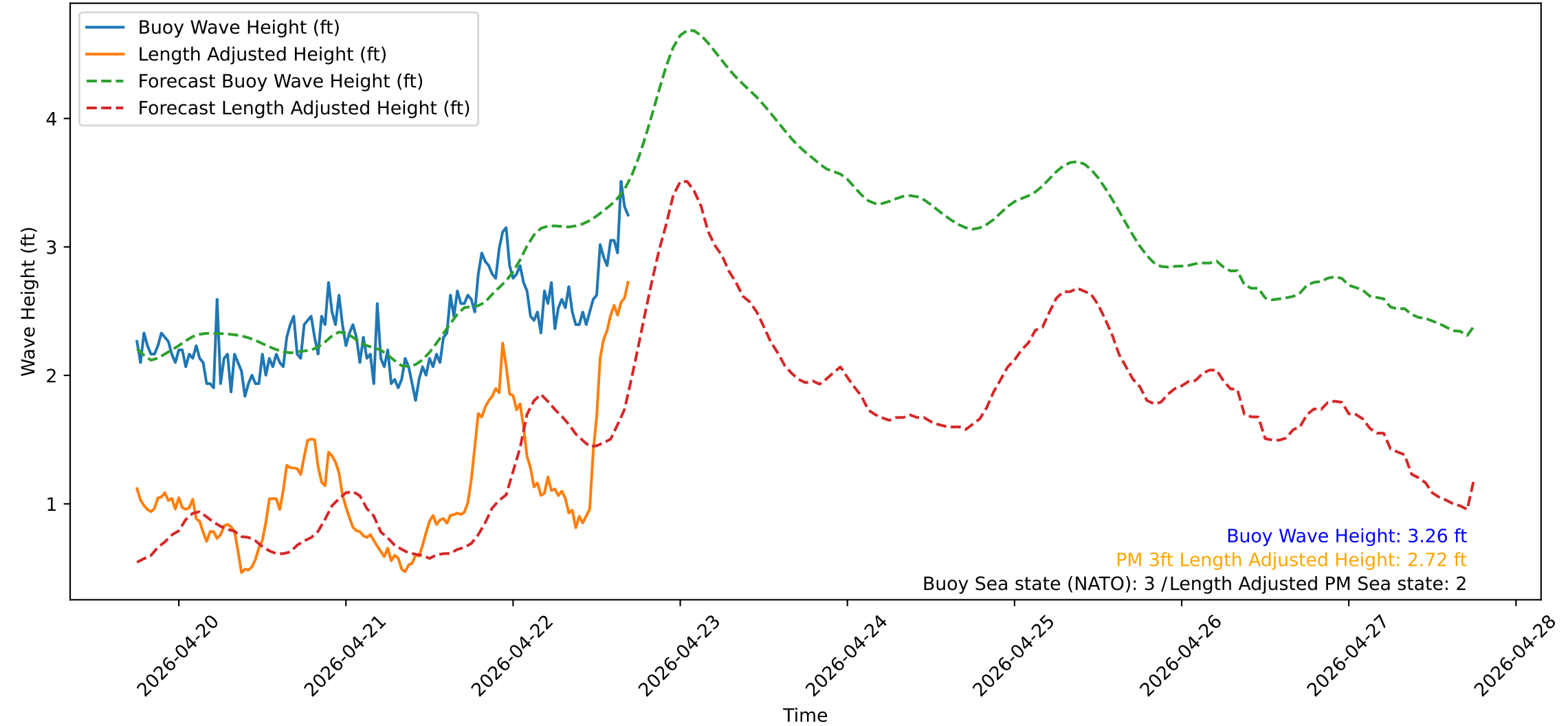
Wave Heights over Time for Red Beach at 2026-04-22 17:30:51
