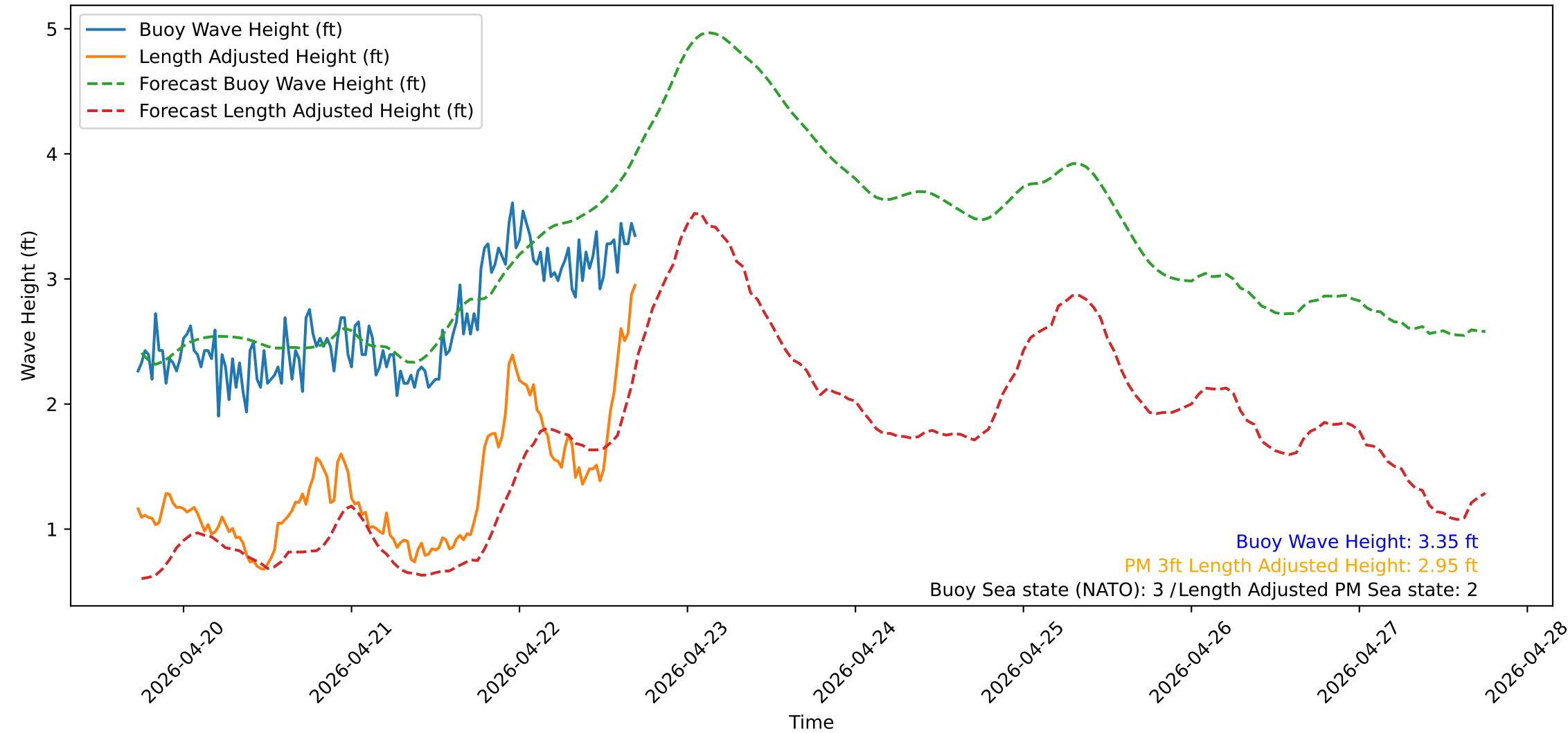
Wave Heights over Time for Oceanside Harbor at 2026-04-22 17:30:32
