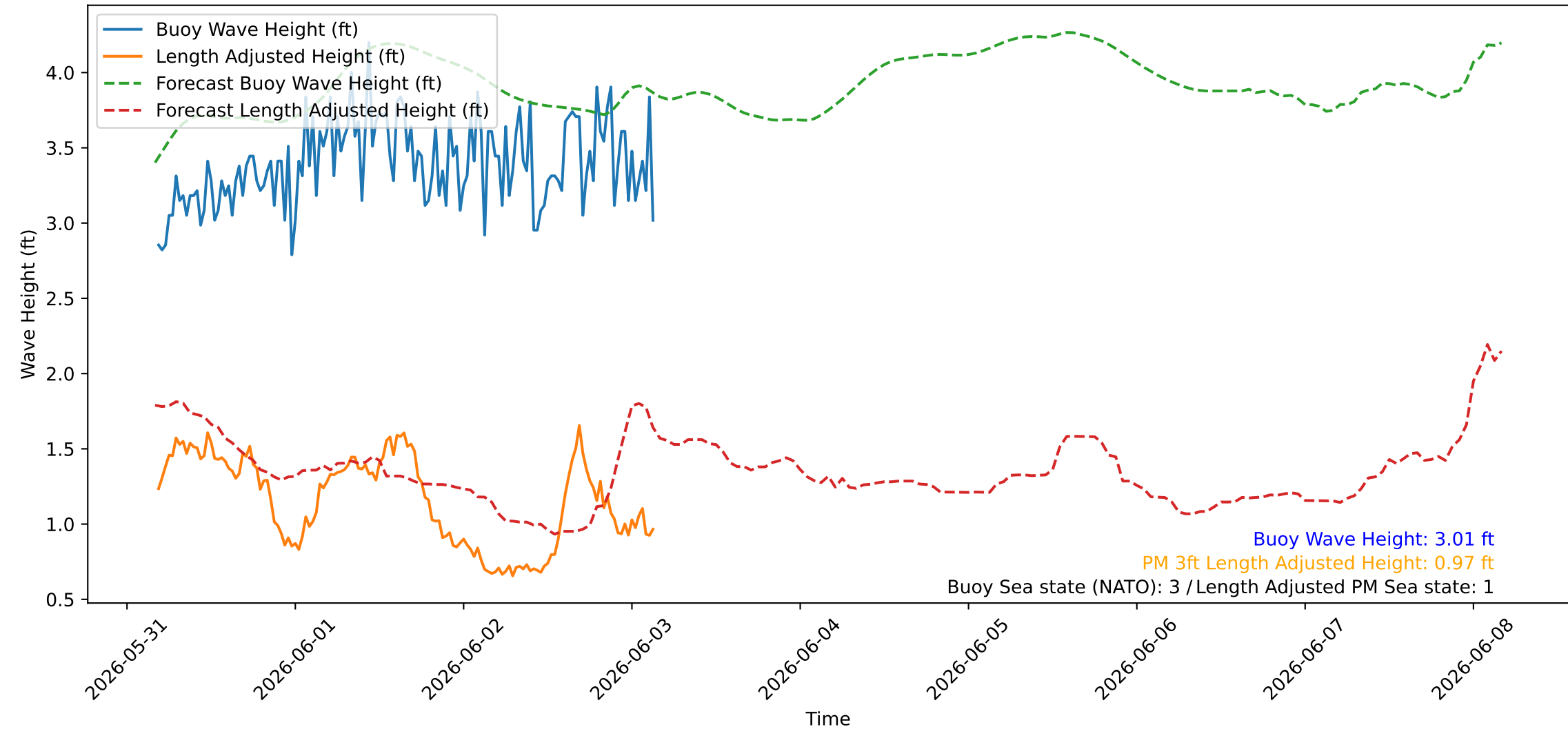
Wave Heights over Time for Red Beach at 2026-06-03 04:00:45
