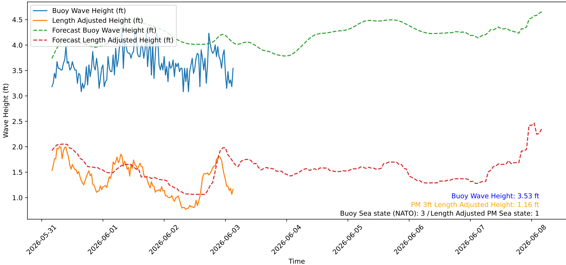
Wave Heights over Time for Green Beach at 2026-06-03 04:01:07
