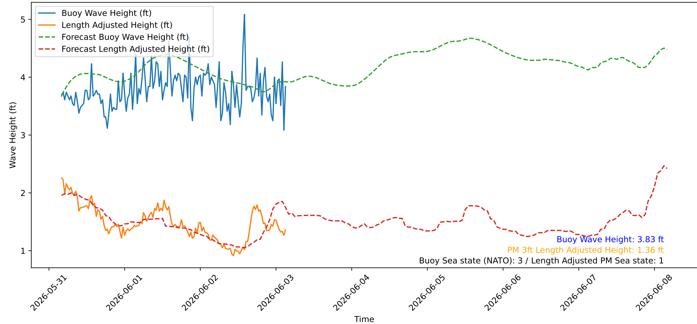
Wave Heights over Time for Oceanside Harbor at 2026-06-03 04:00:26
