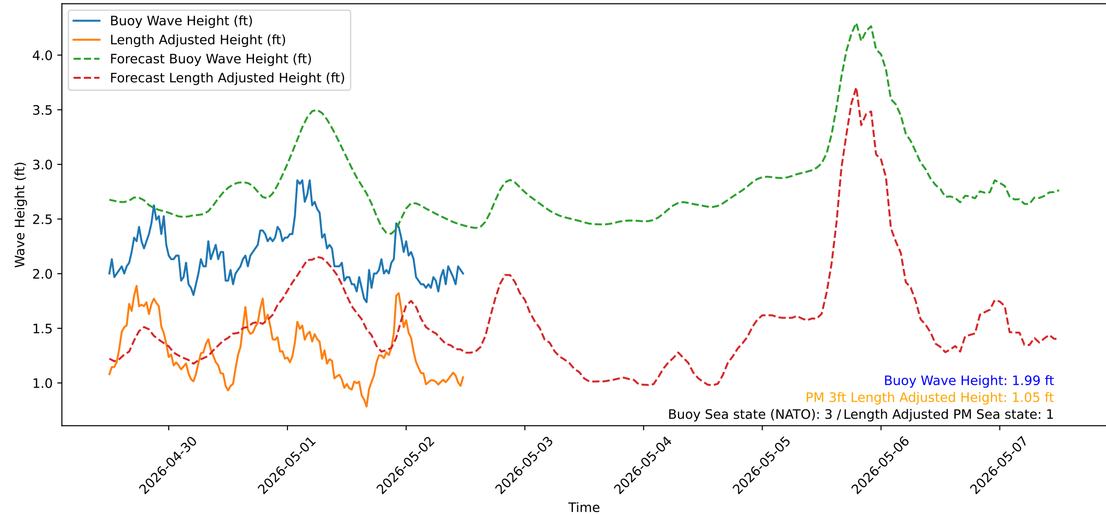
Wave Heights over Time for Green Beach at 2026-05-02 12:11:12
