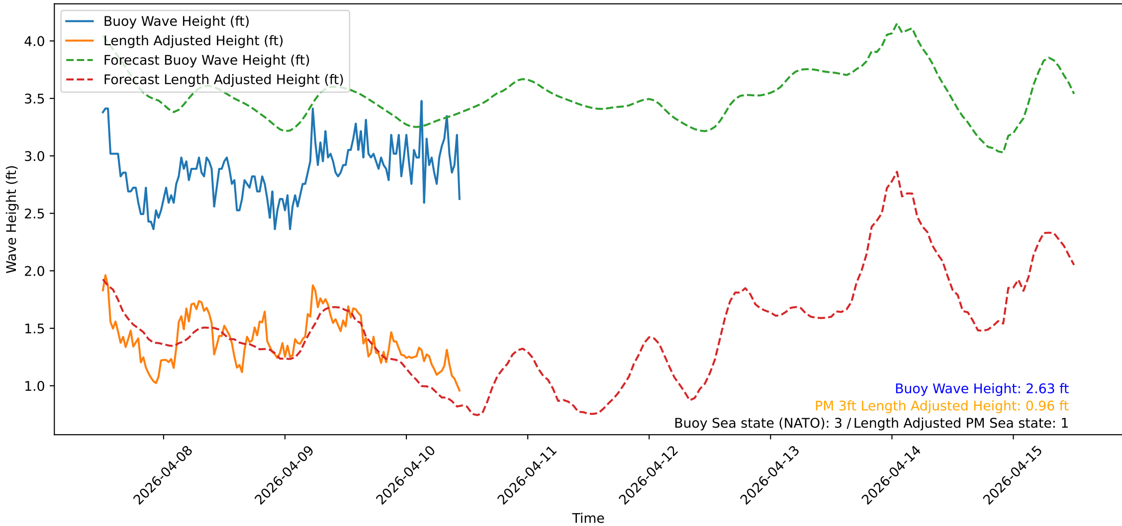
Wave Heights over Time for Green Beach at 2026-04-10 11:51:14
