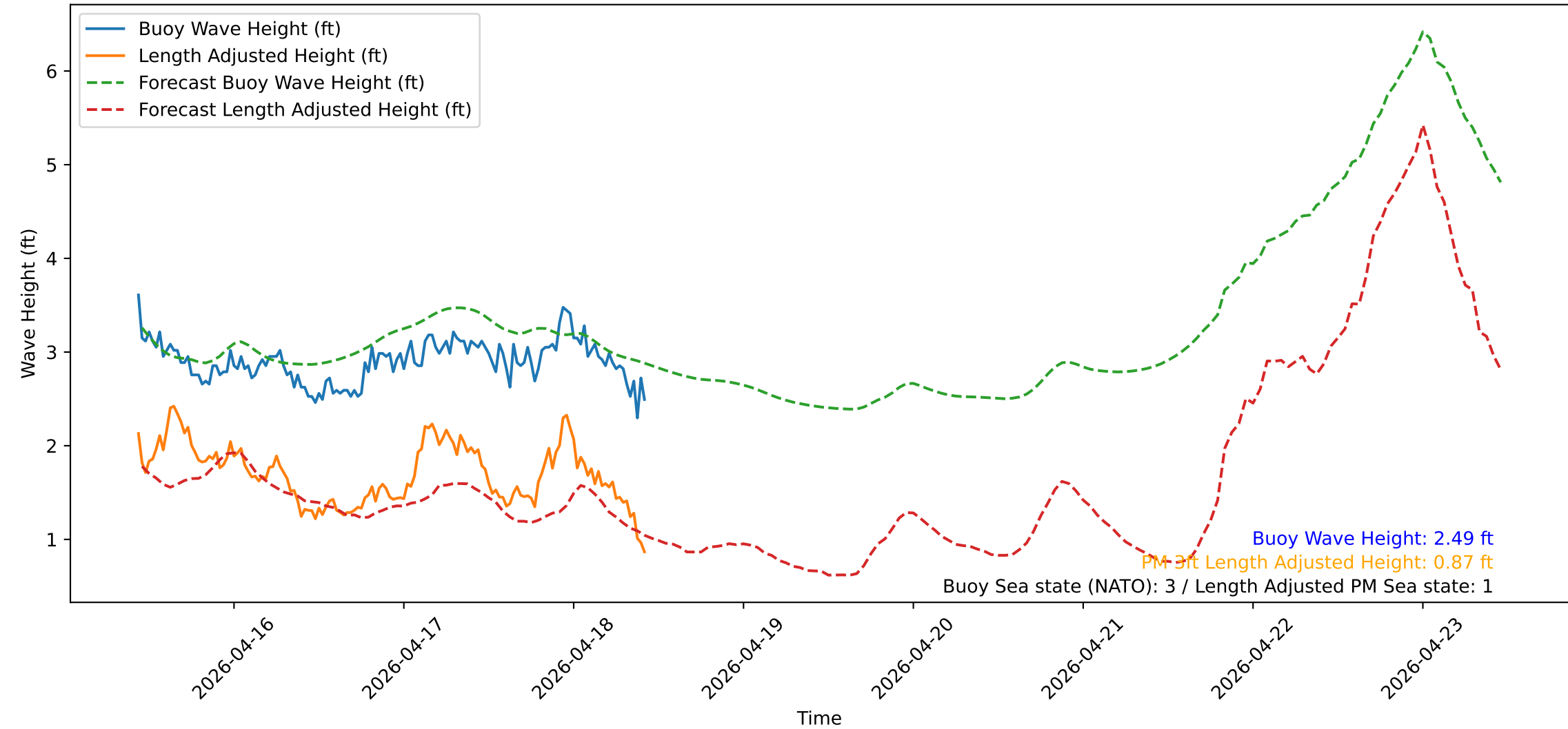
Wave Heights over Time for Green Beach at 2026-04-18 10:41:13
