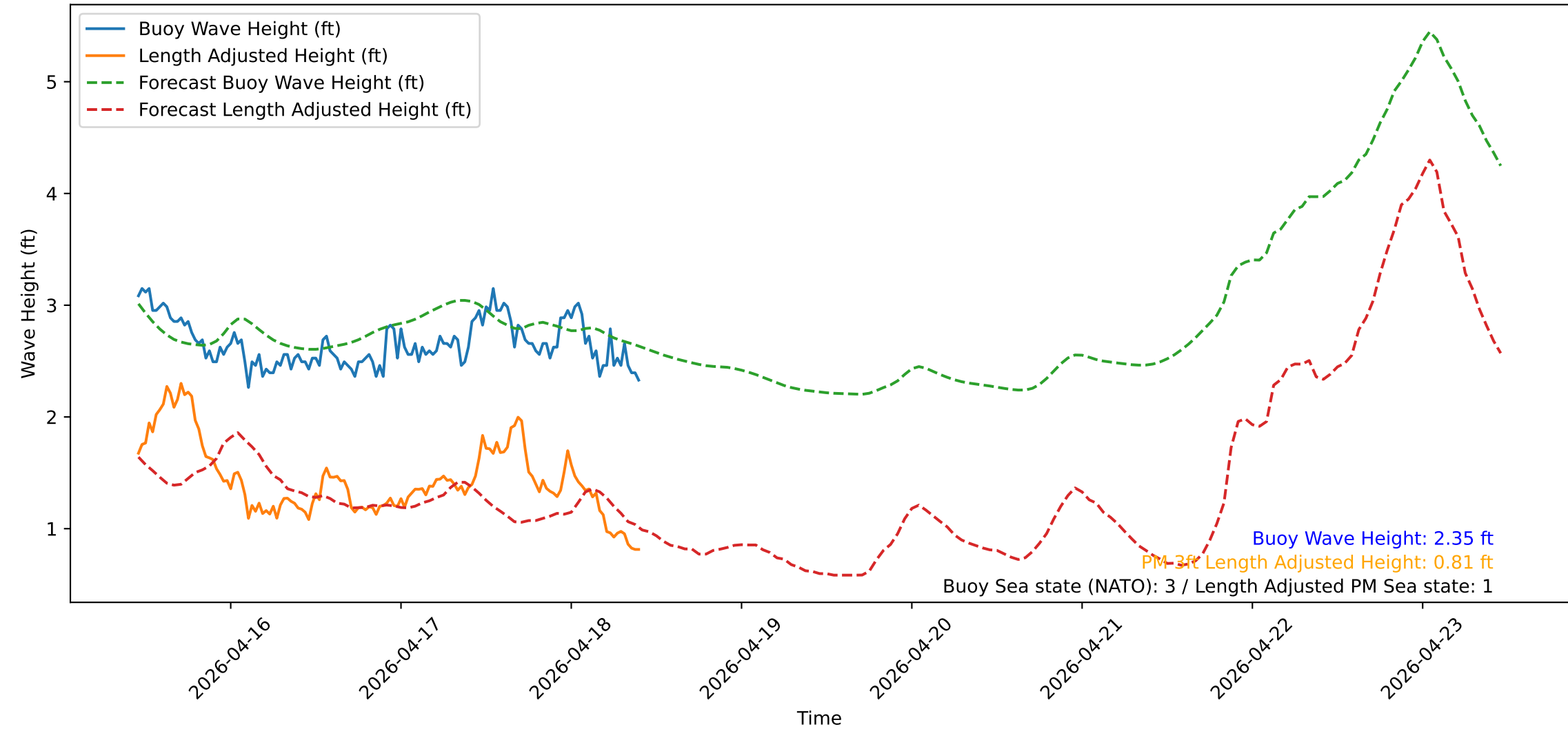
Wave Heights over Time for Red Beach at 2026-04-18 10:40:50
