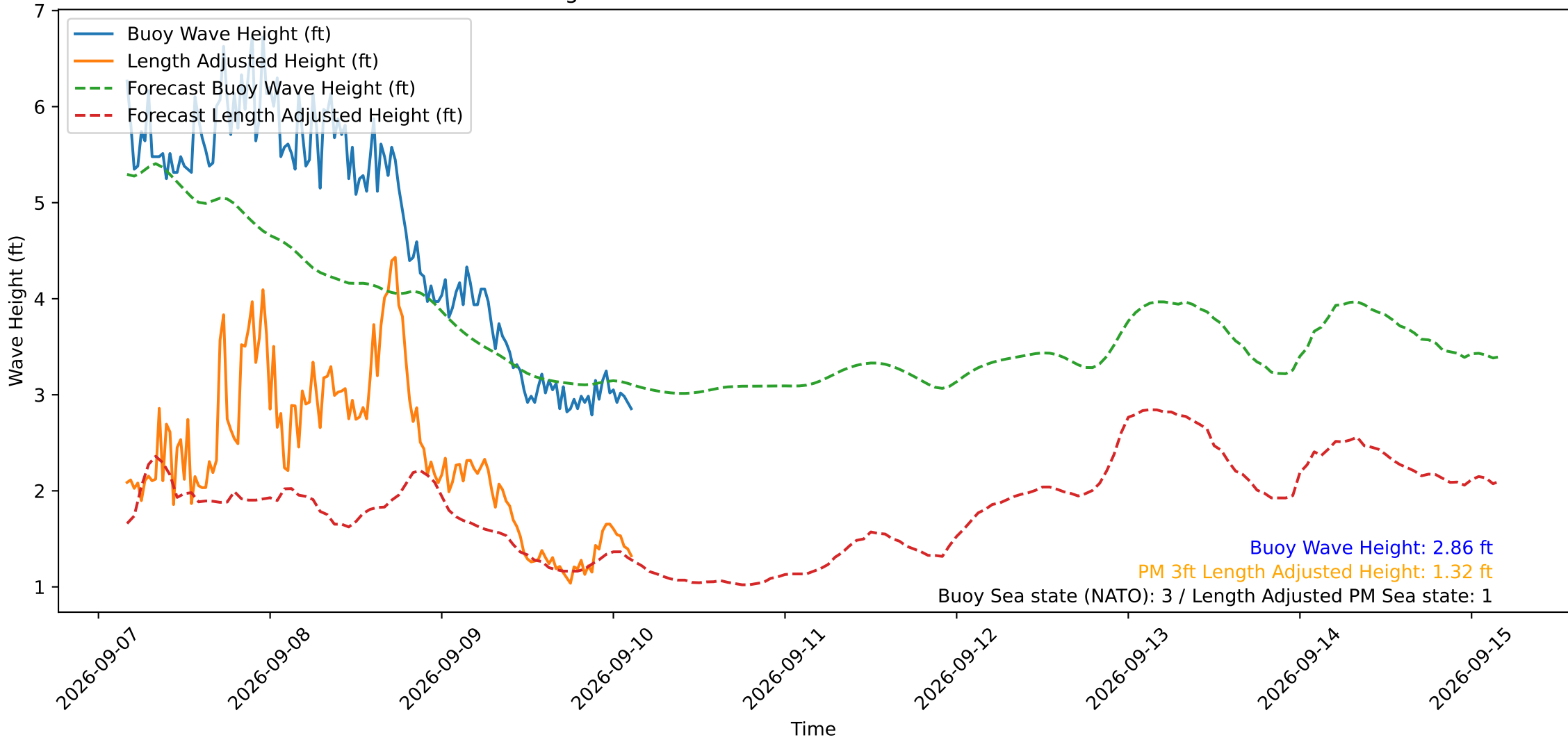
Wave Heights over Time for Red Beach at 2026-09-10 03:30:50
