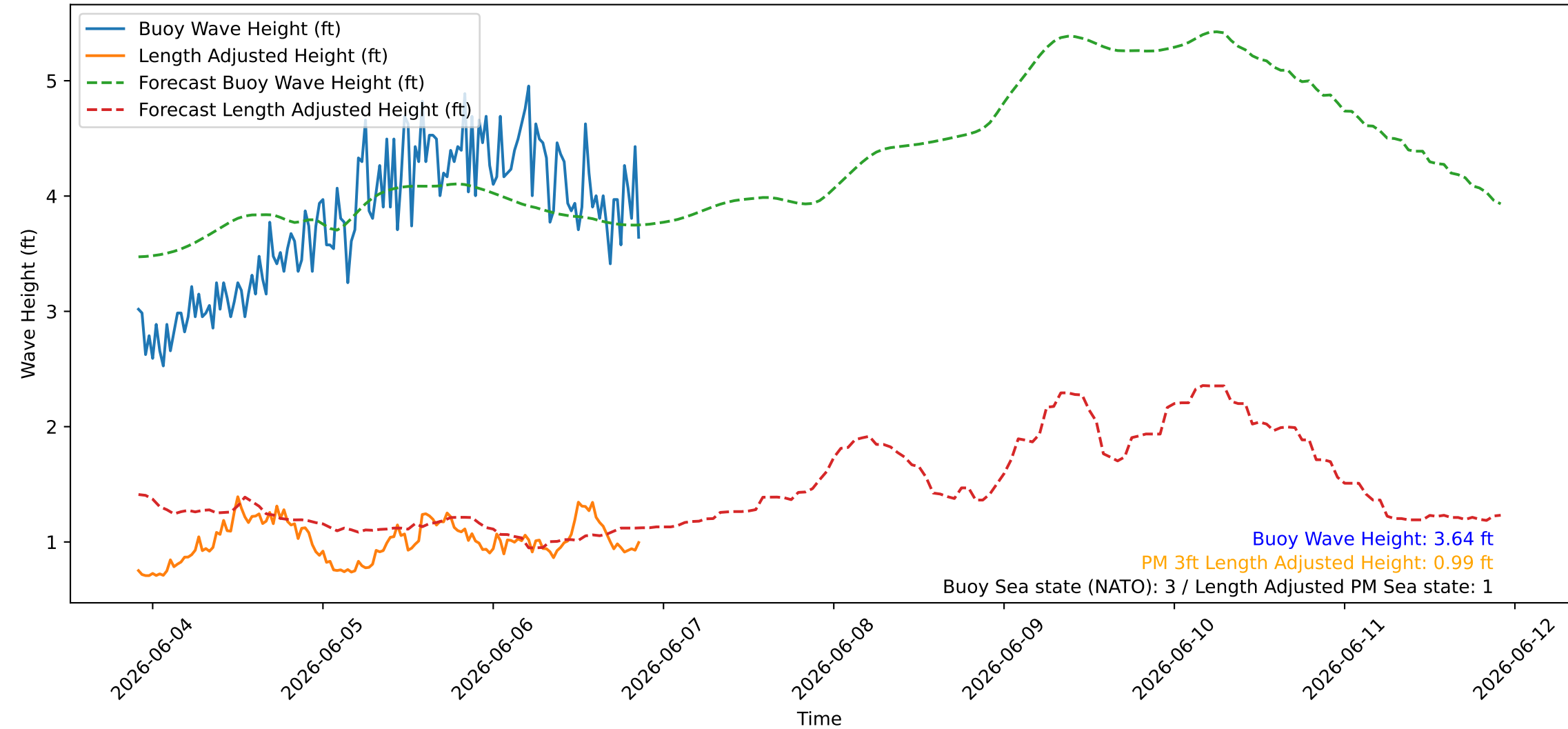
Wave Heights over Time for Red Beach at 2026-06-06 21:30:45
