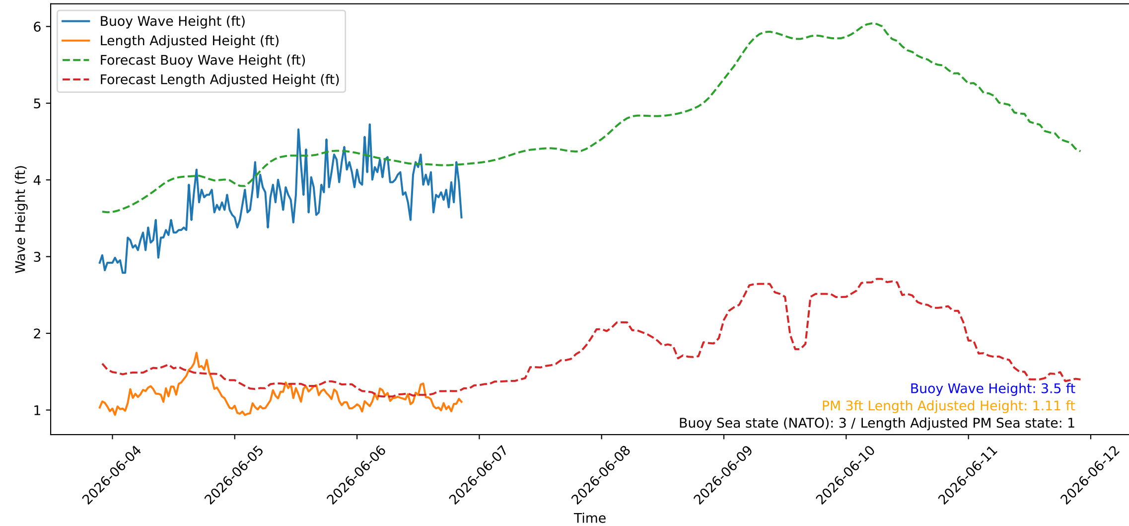
Wave Heights over Time for Green Beach at 2026-06-06 21:31:07
