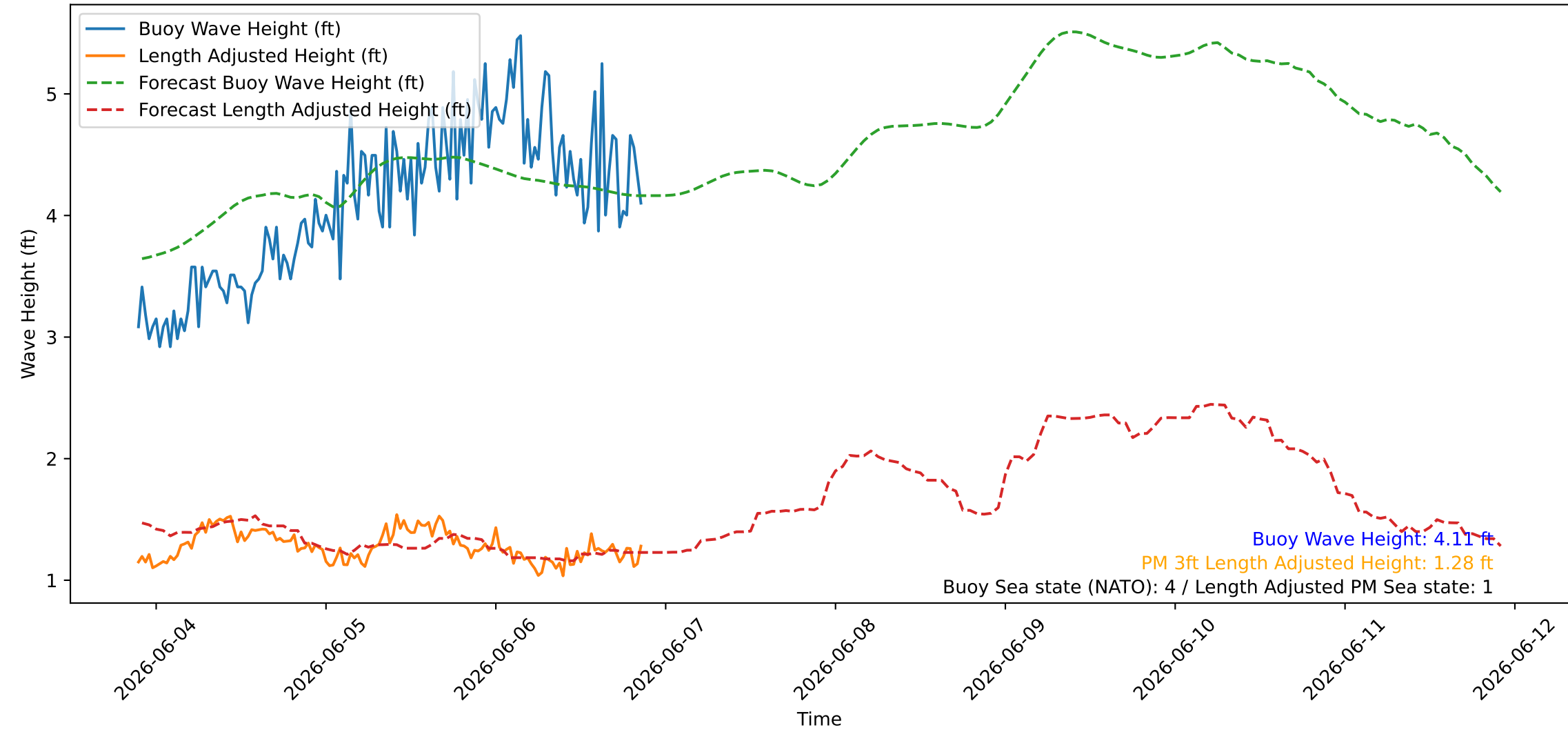
Wave Heights over Time for Oceanside Harbor at 2026-06-06 21:30:26
