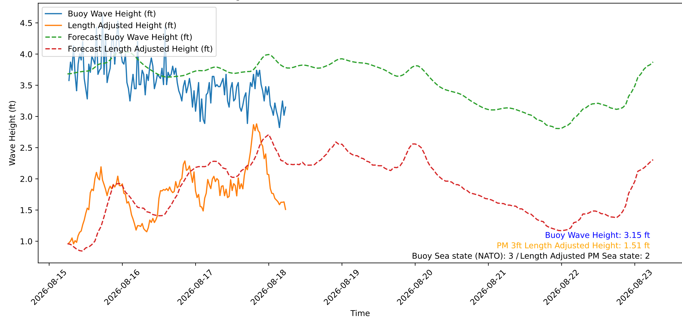
Wave Heights over Time for Oceanside Harbor at 2026-08-18 06:20:27
