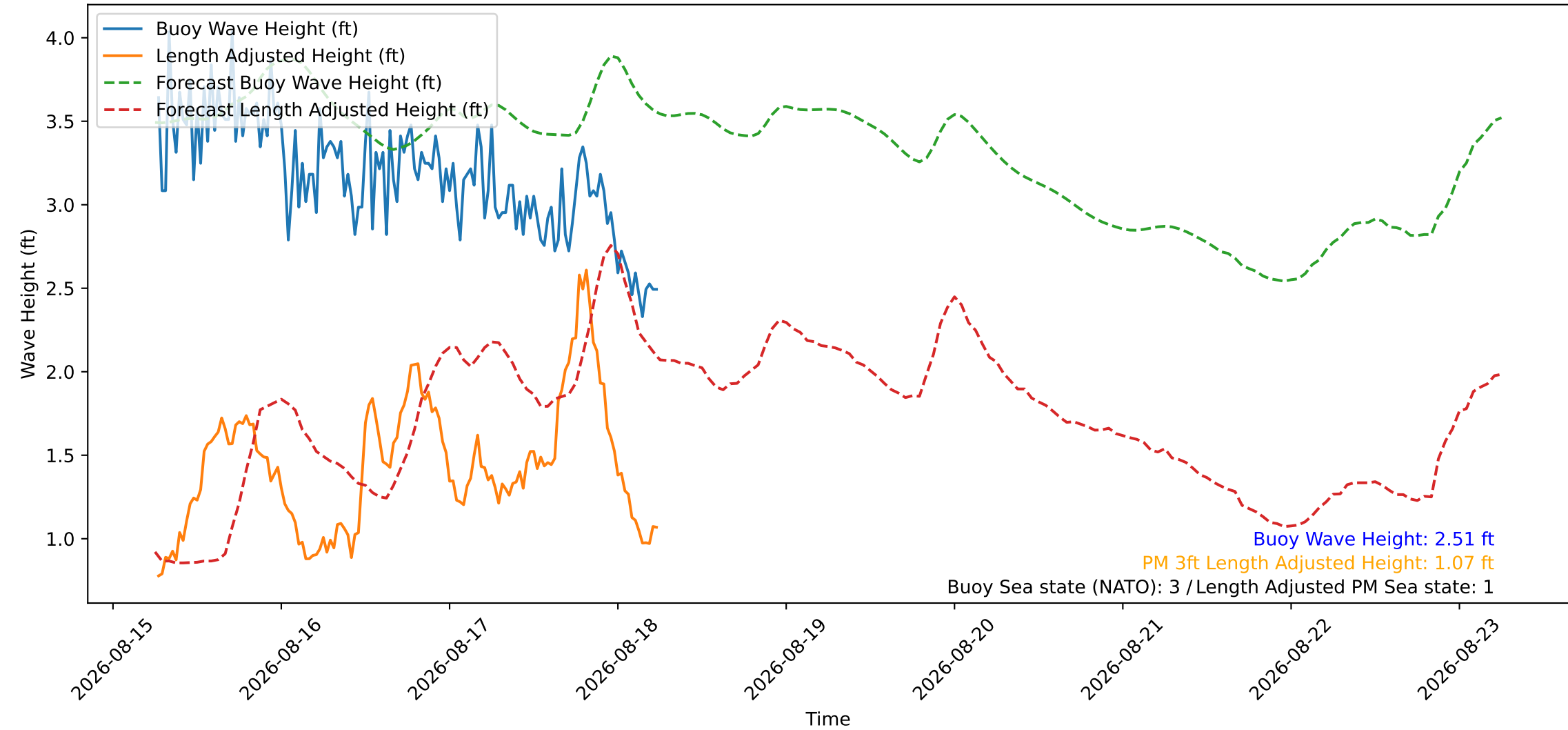
Wave Heights over Time for Red Beach at 2026-08-18 06:20:49
