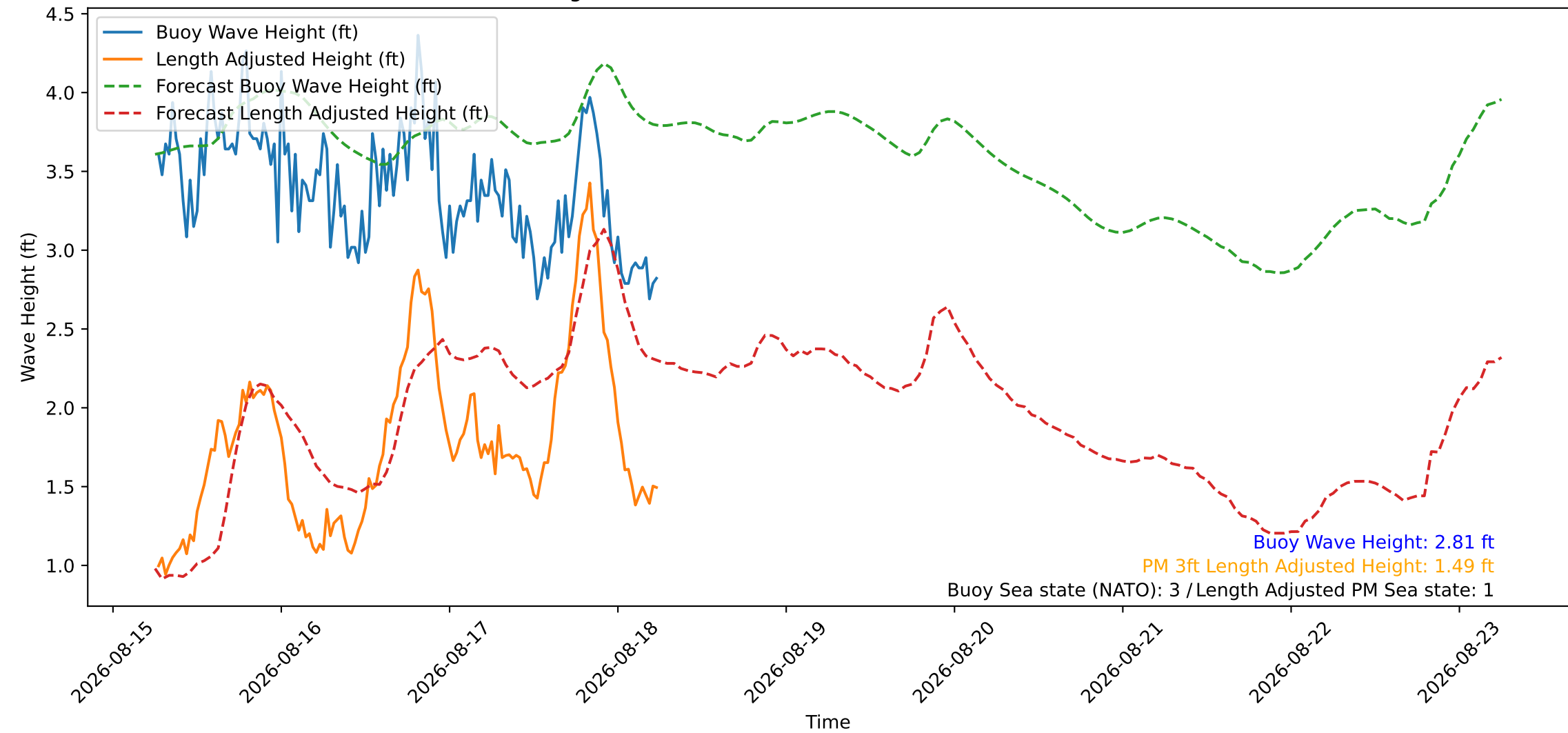
Wave Heights over Time for Green Beach at 2026-08-18 06:21:13
