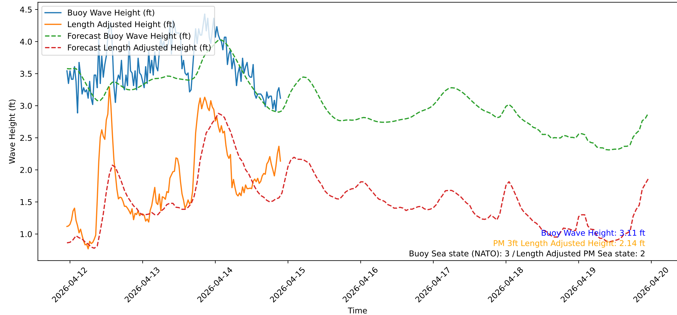
Wave Heights over Time for Red Beach at 2026-04-14 22:30:50
