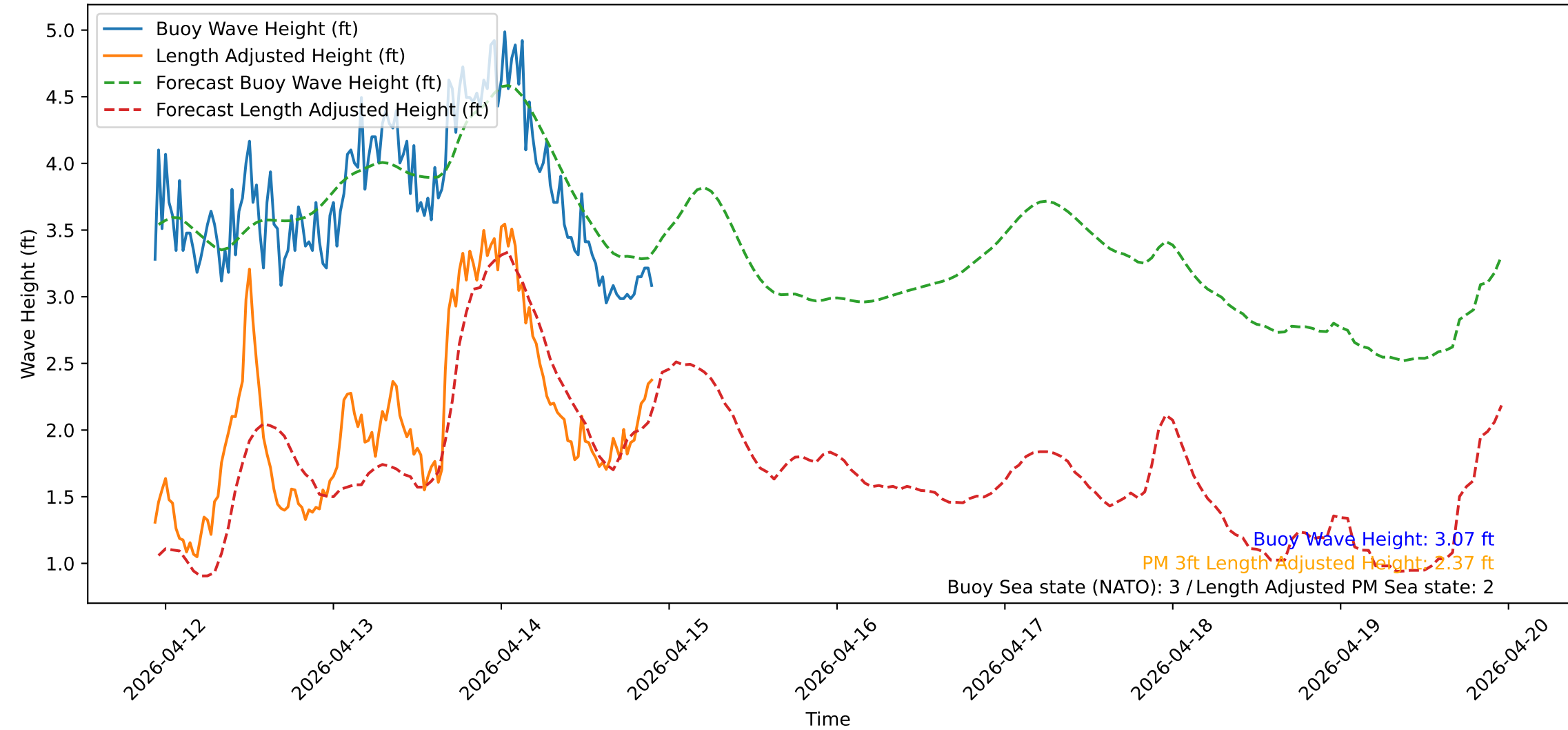
Wave Heights over Time for Green Beach at 2026-04-14 22:31:12
