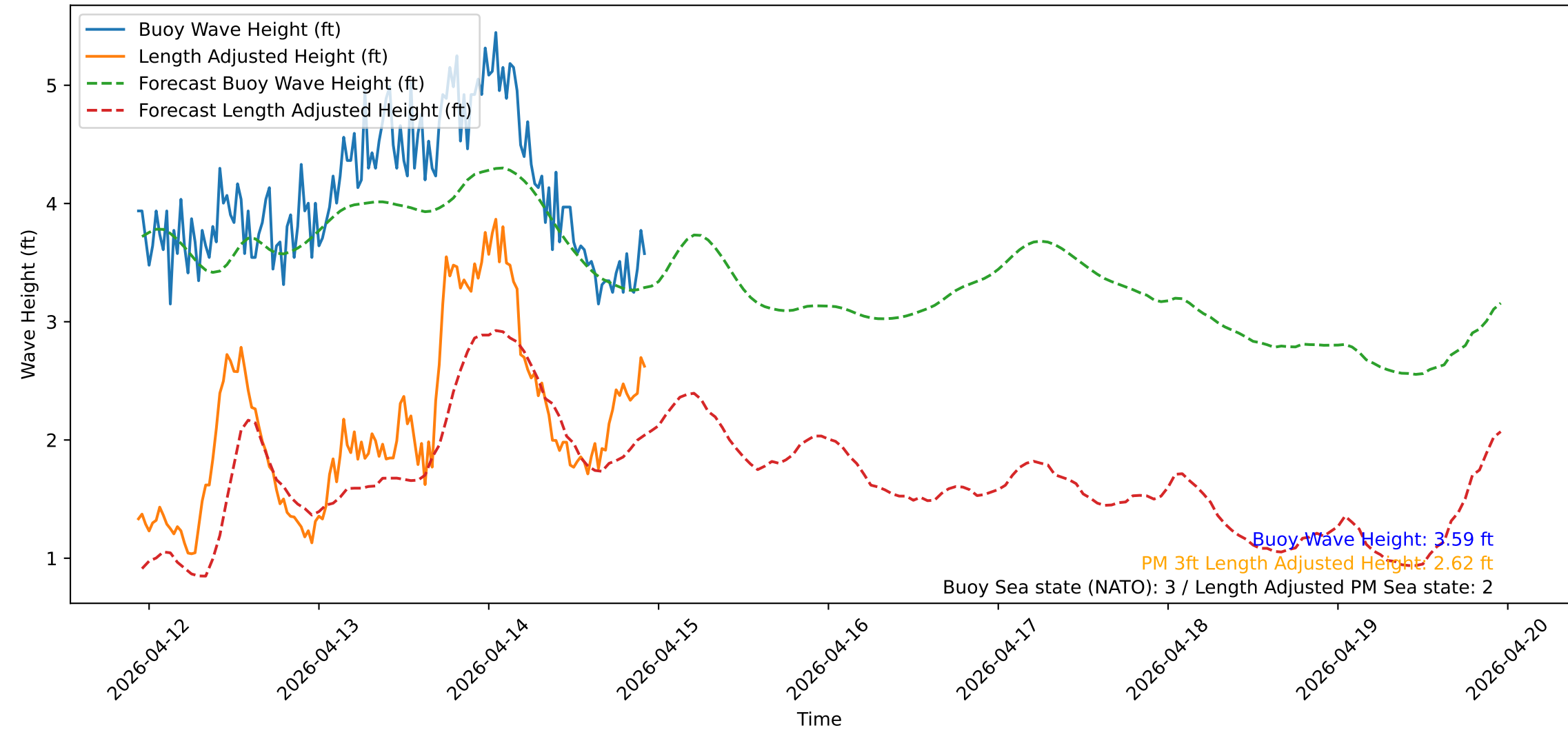
Wave Heights over Time for Oceanside Harbor at 2026-04-14 22:30:31
