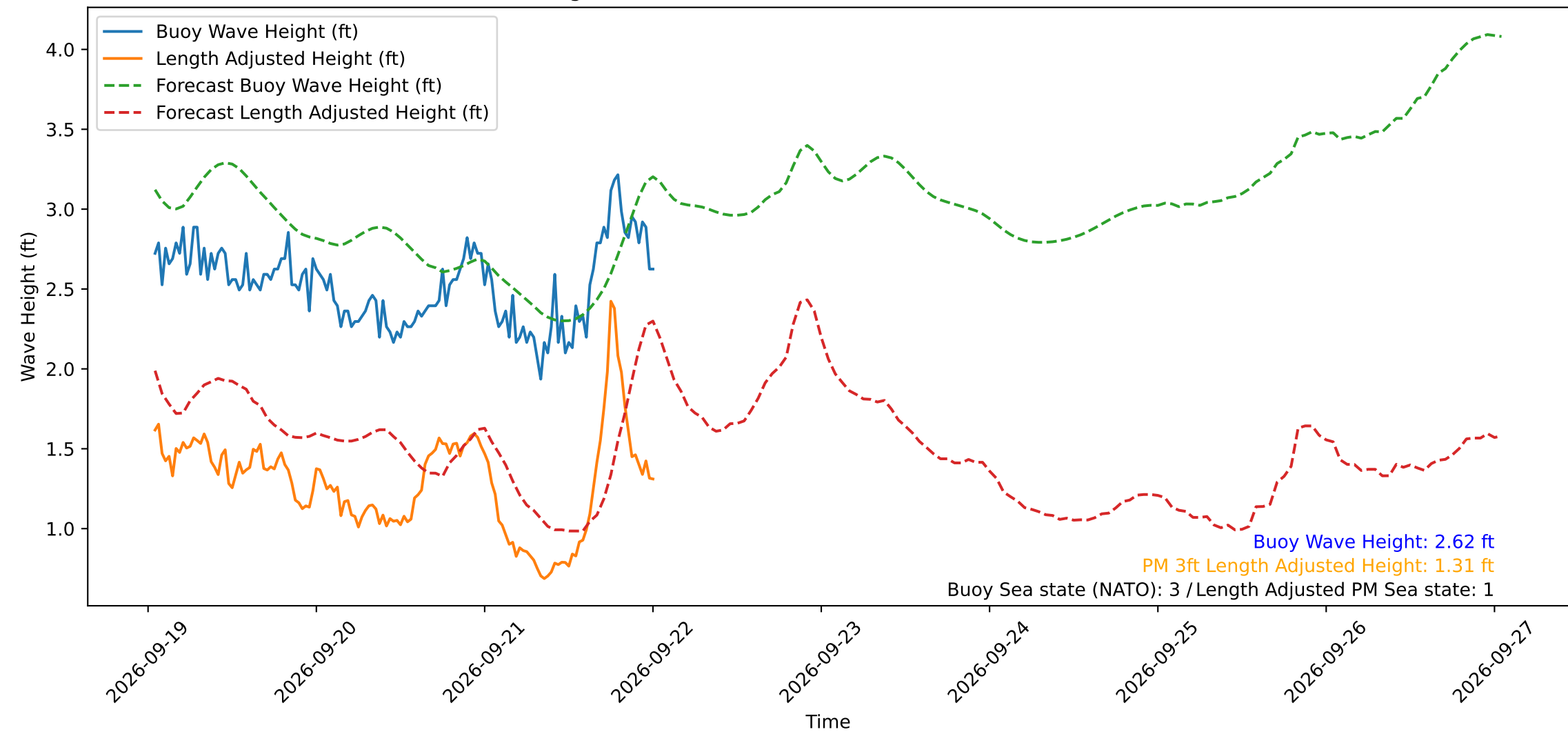
Wave Heights over Time for Green Beach at 2026-09-22 00:41:11
