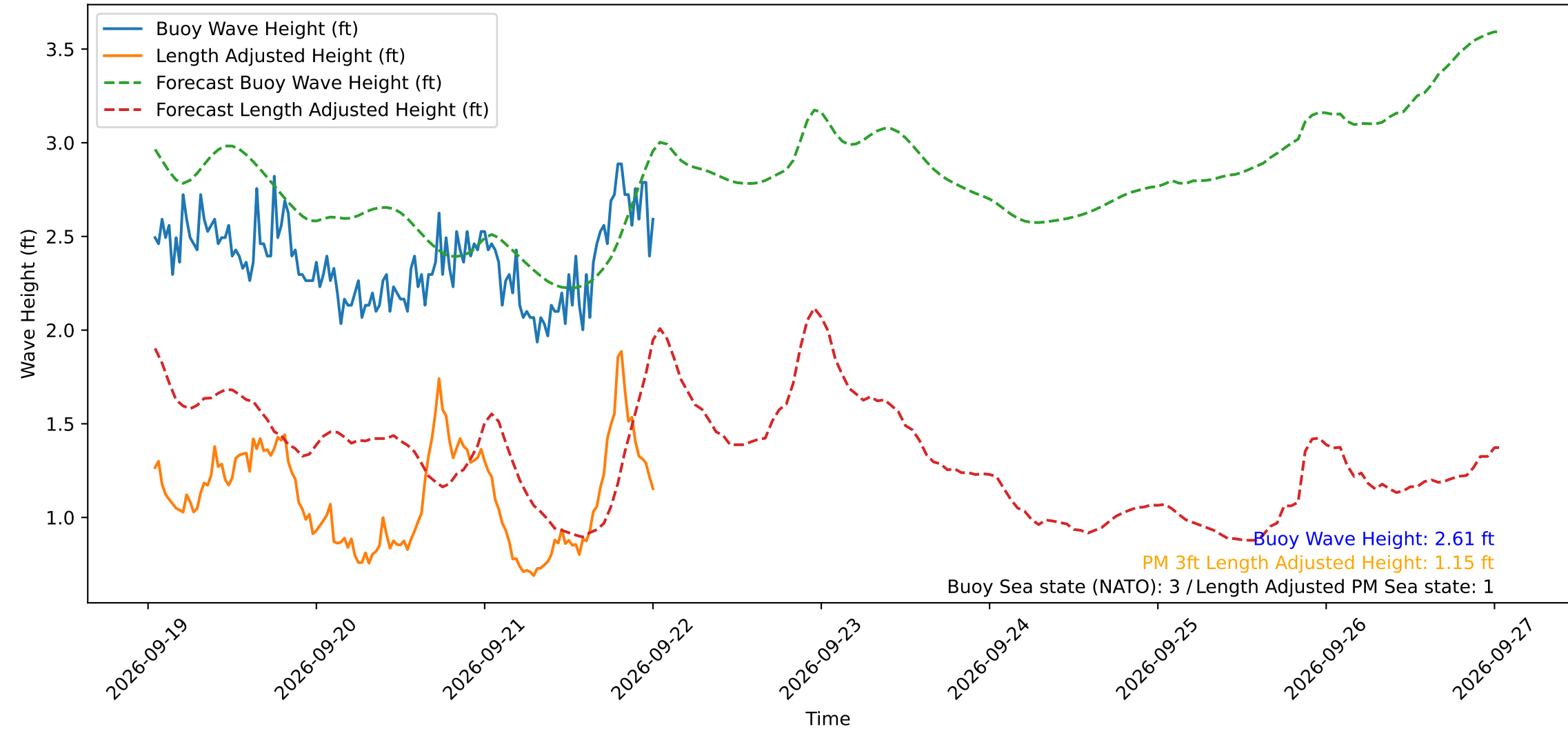
Wave Heights over Time for Red Beach at 2026-09-22 00:40:49
