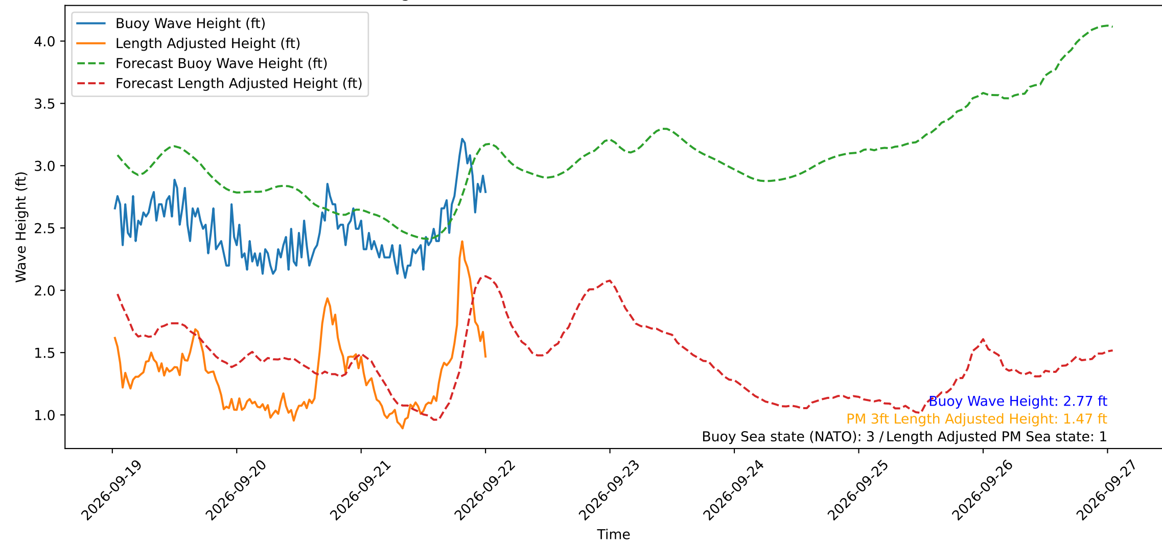
Wave Heights over Time for Oceanside Harbor at 2026-09-22 00:40:29
