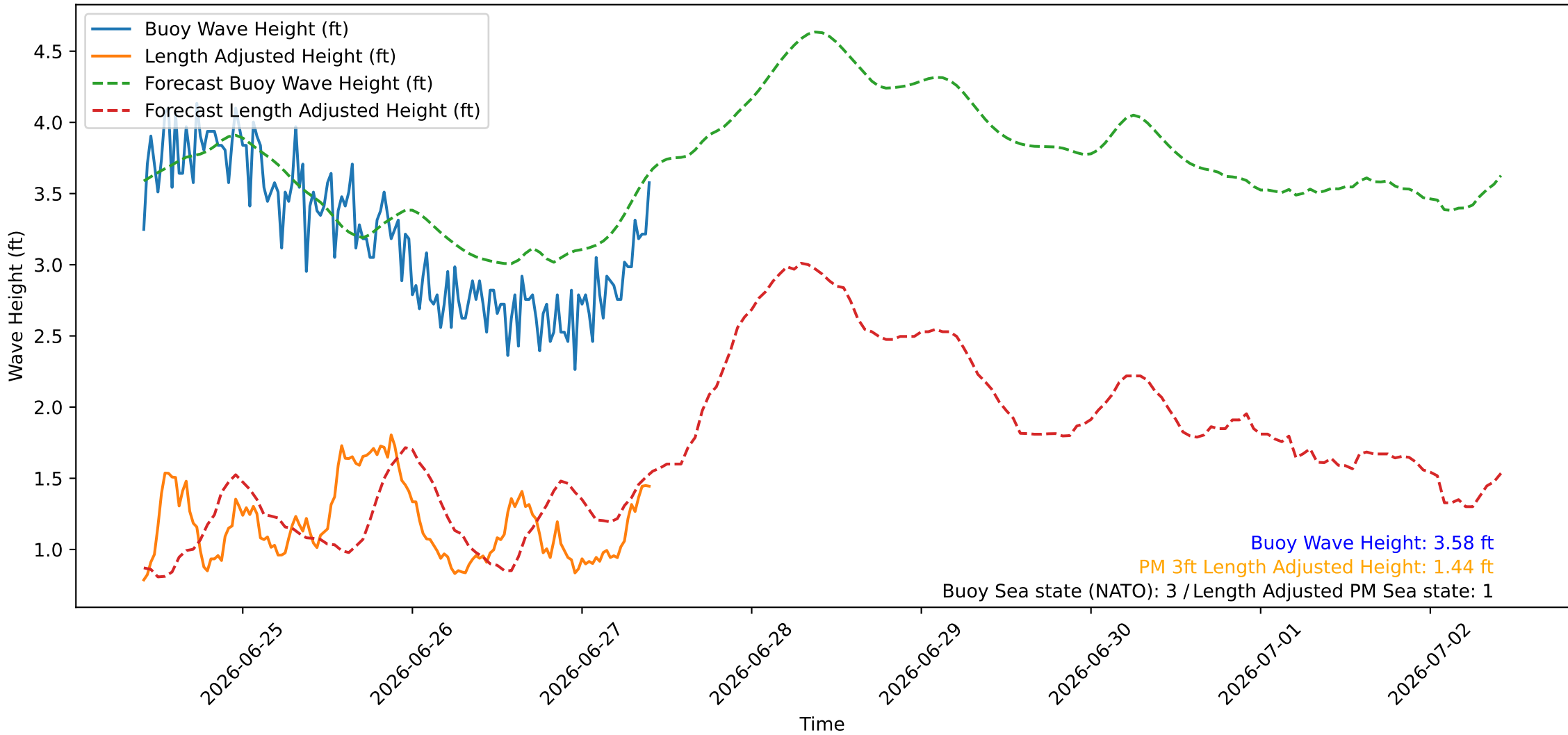
Wave Heights over Time for Green Beach at 2026-06-27 10:11:08
