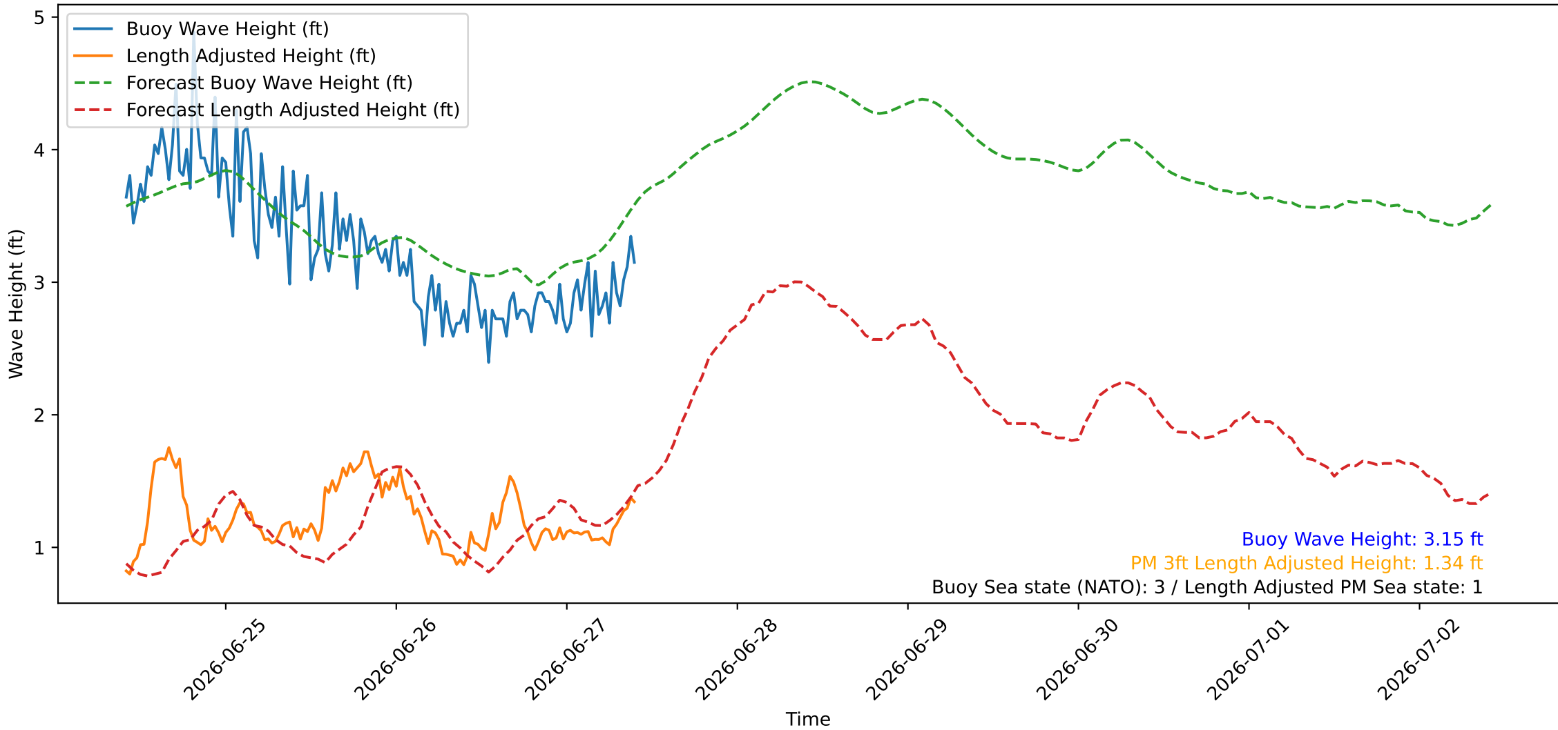
Wave Heights over Time for Oceanside Harbor at 2026-06-27 10:10:26
