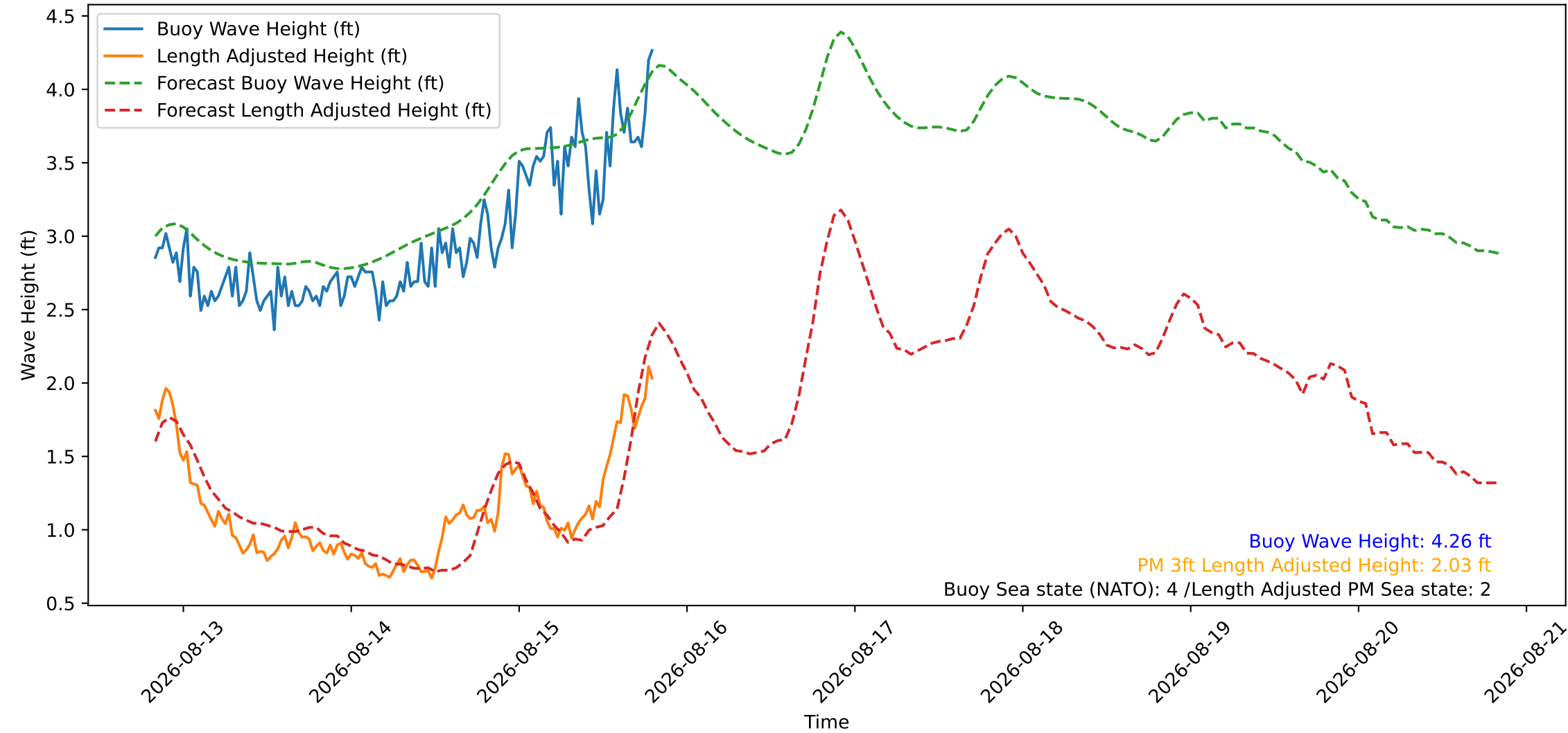
Wave Heights over Time for Green Beach at 2026-08-15 19:51:12
