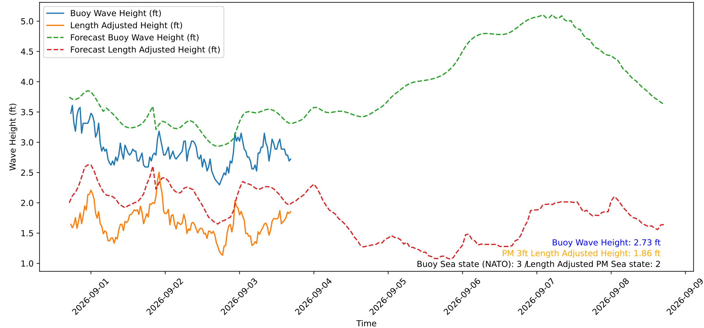
Wave Heights over Time for Red Beach at 2026-09-03 17:10:50
