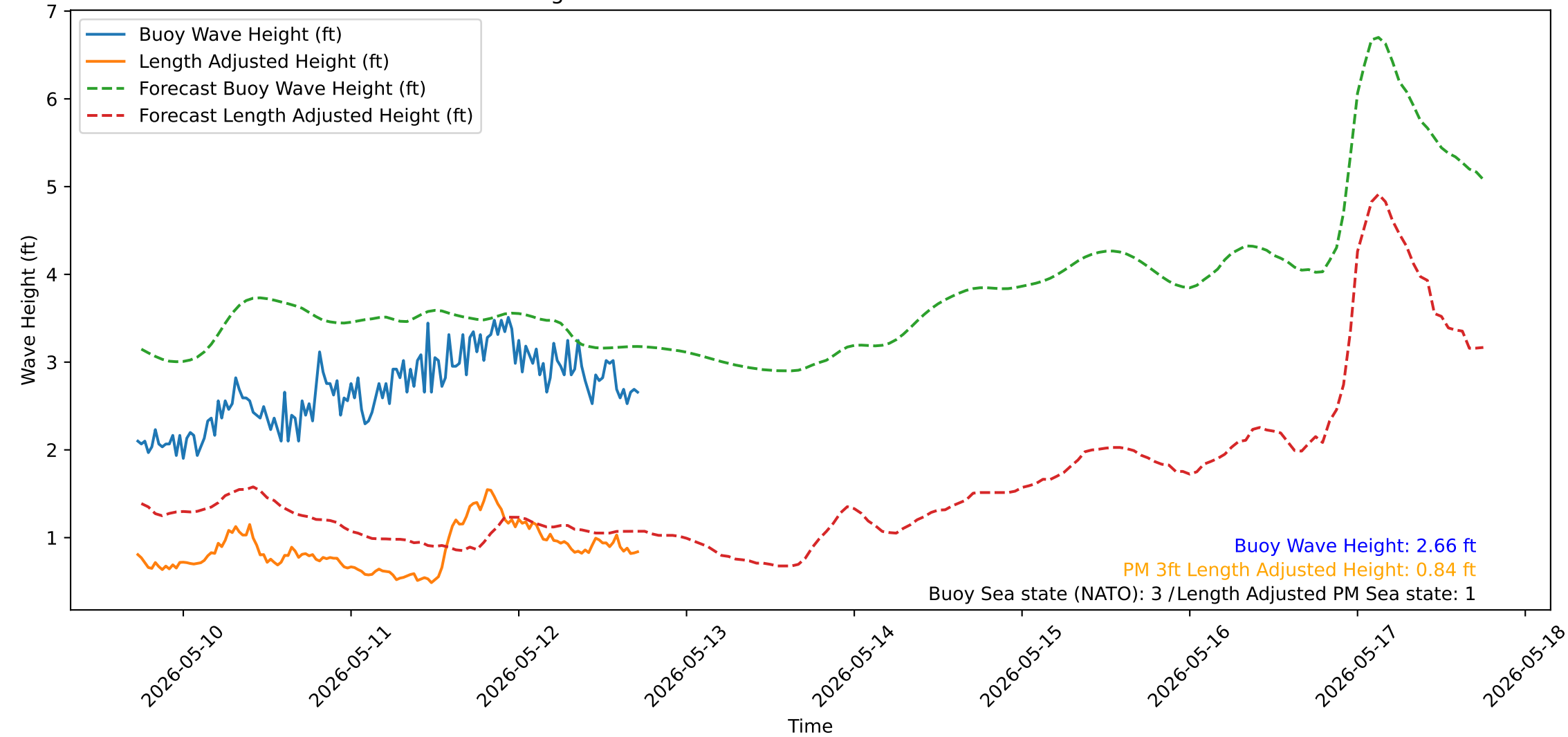
Wave Heights over Time for Green Beach at 2026-05-12 17:41:13
