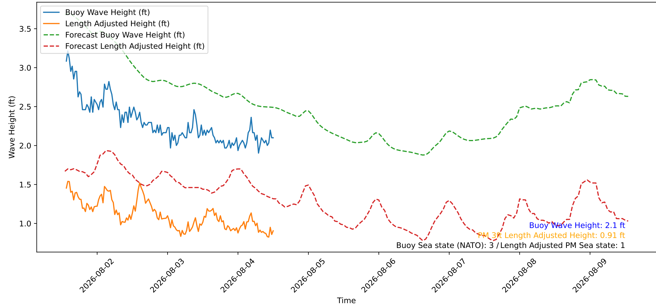
Wave Heights over Time for Red Beach at 2026-08-04 13:00:46
