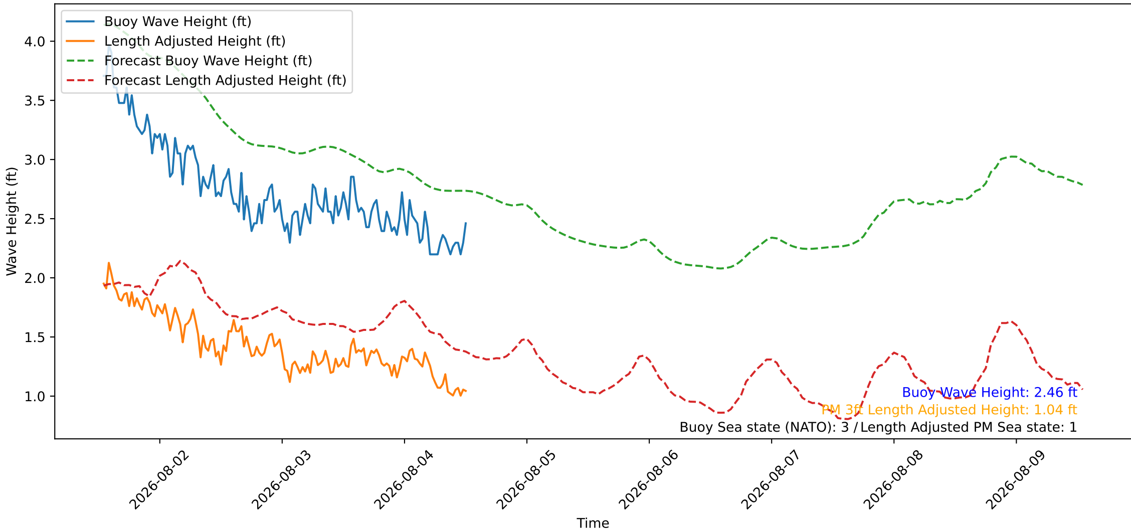
Wave Heights over Time for Oceanside Harbor at 2026-08-04 13:00:27
