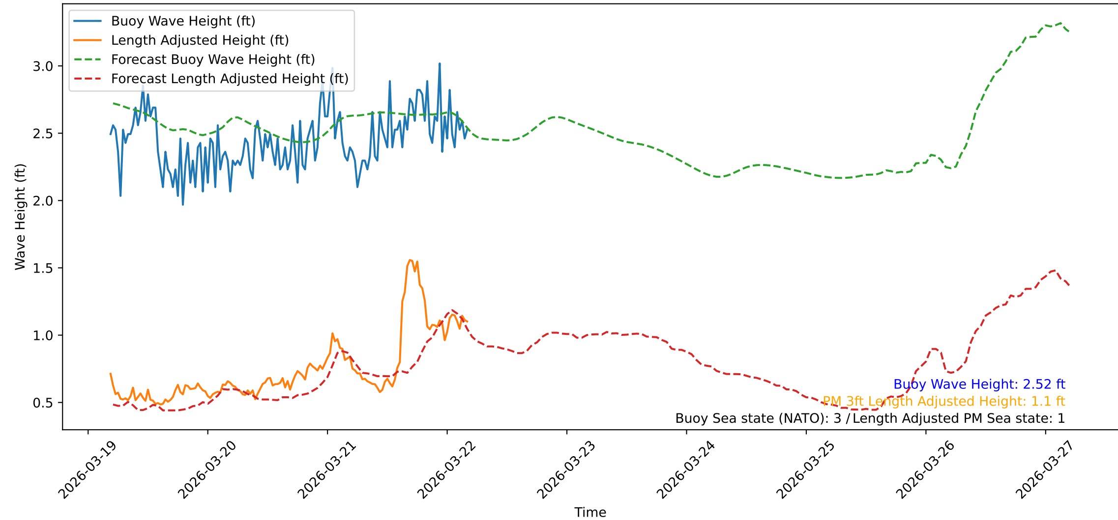
Wave Heights over Time for Oceanside Harbor at 2026-03-22 04:30:32
