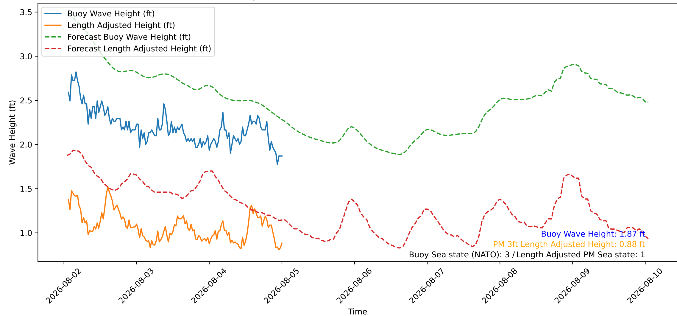
Wave Heights over Time for Red Beach at 2026-08-05 01:10:46
