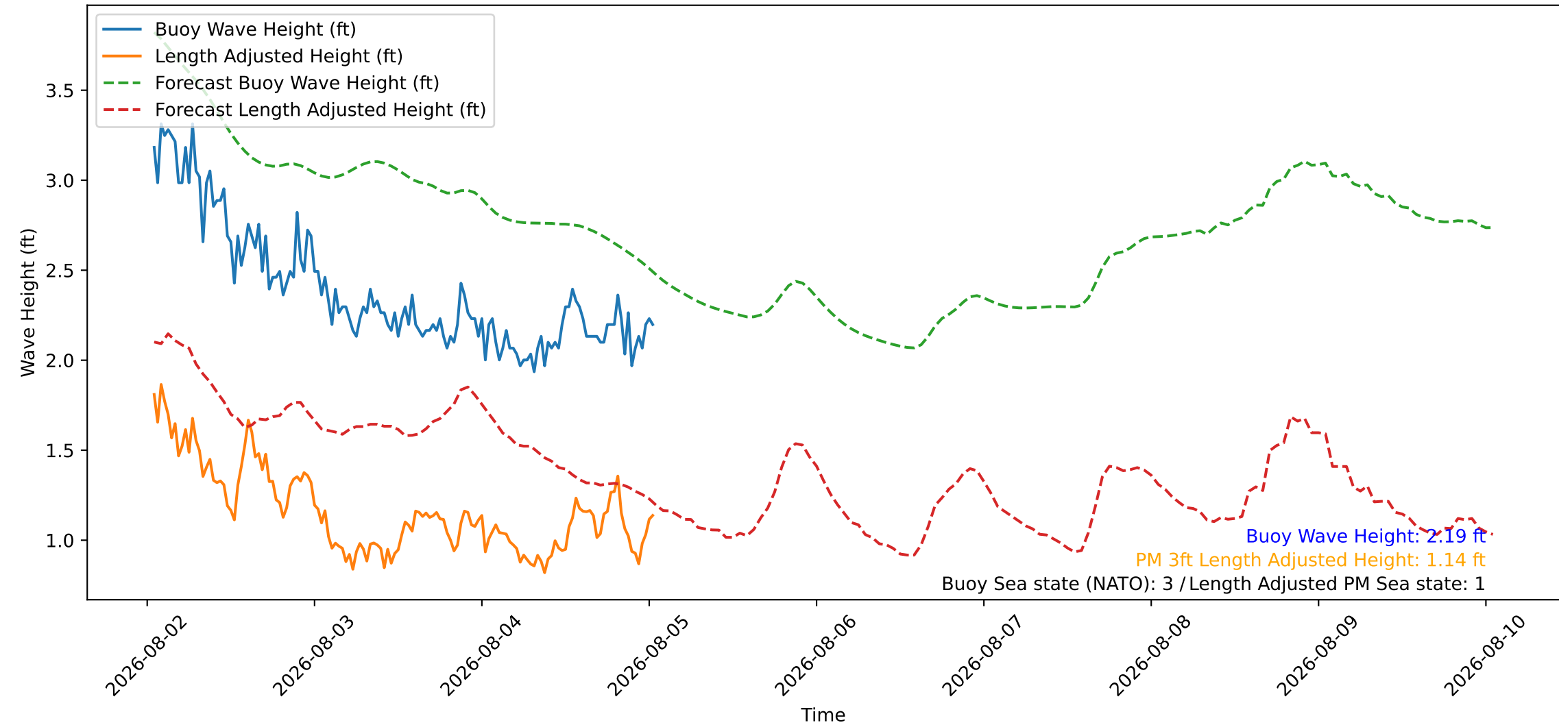
Wave Heights over Time for Green Beach at 2026-08-05 01:11:08
