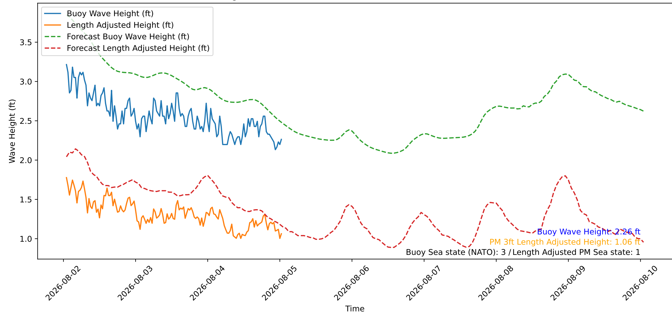
Wave Heights over Time for Oceanside Harbor at 2026-08-05 01:10:26
