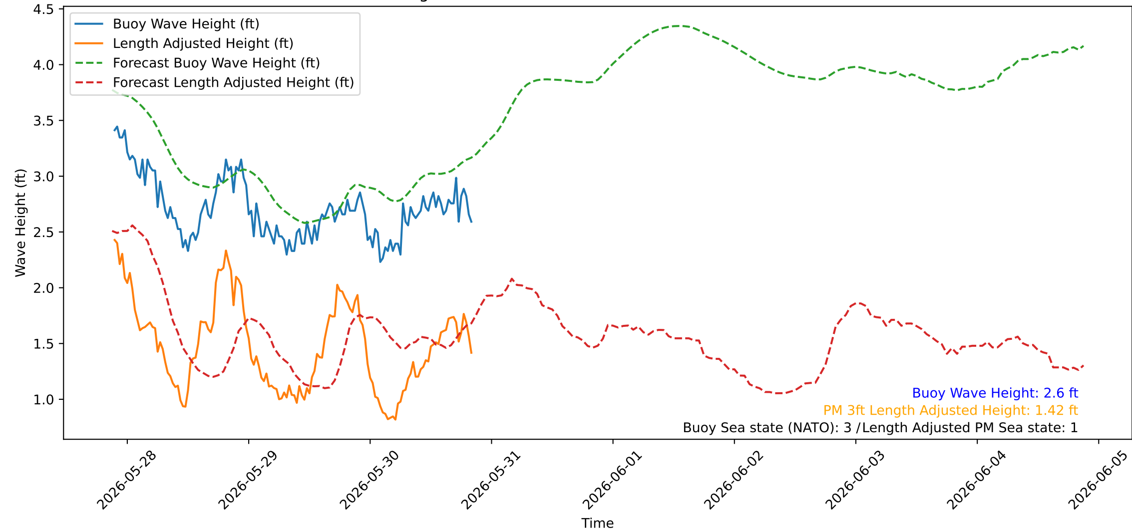
Wave Heights over Time for Red Beach at 2026-05-30 21:10:44
