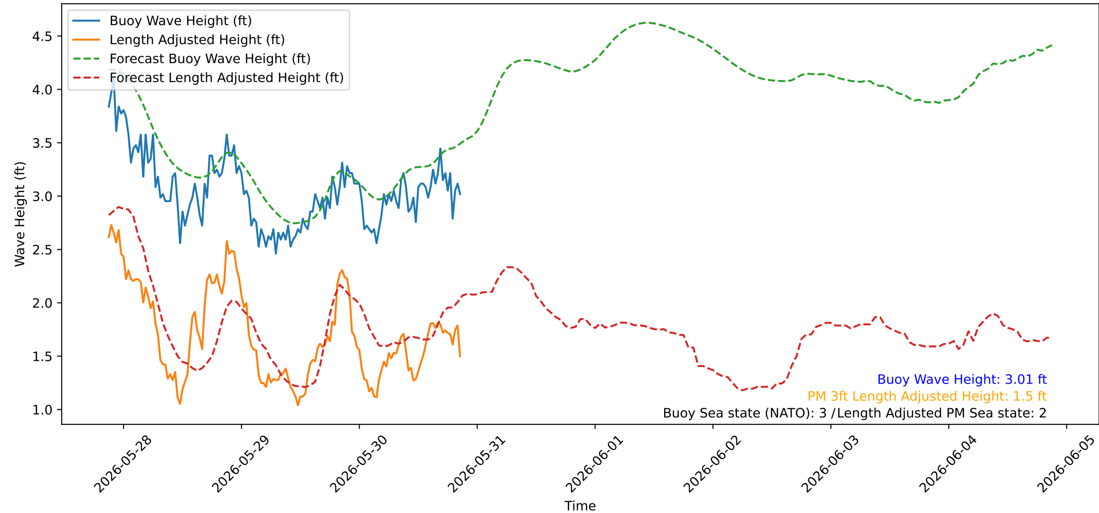
Wave Heights over Time for Green Beach at 2026-05-30 21:11:06
