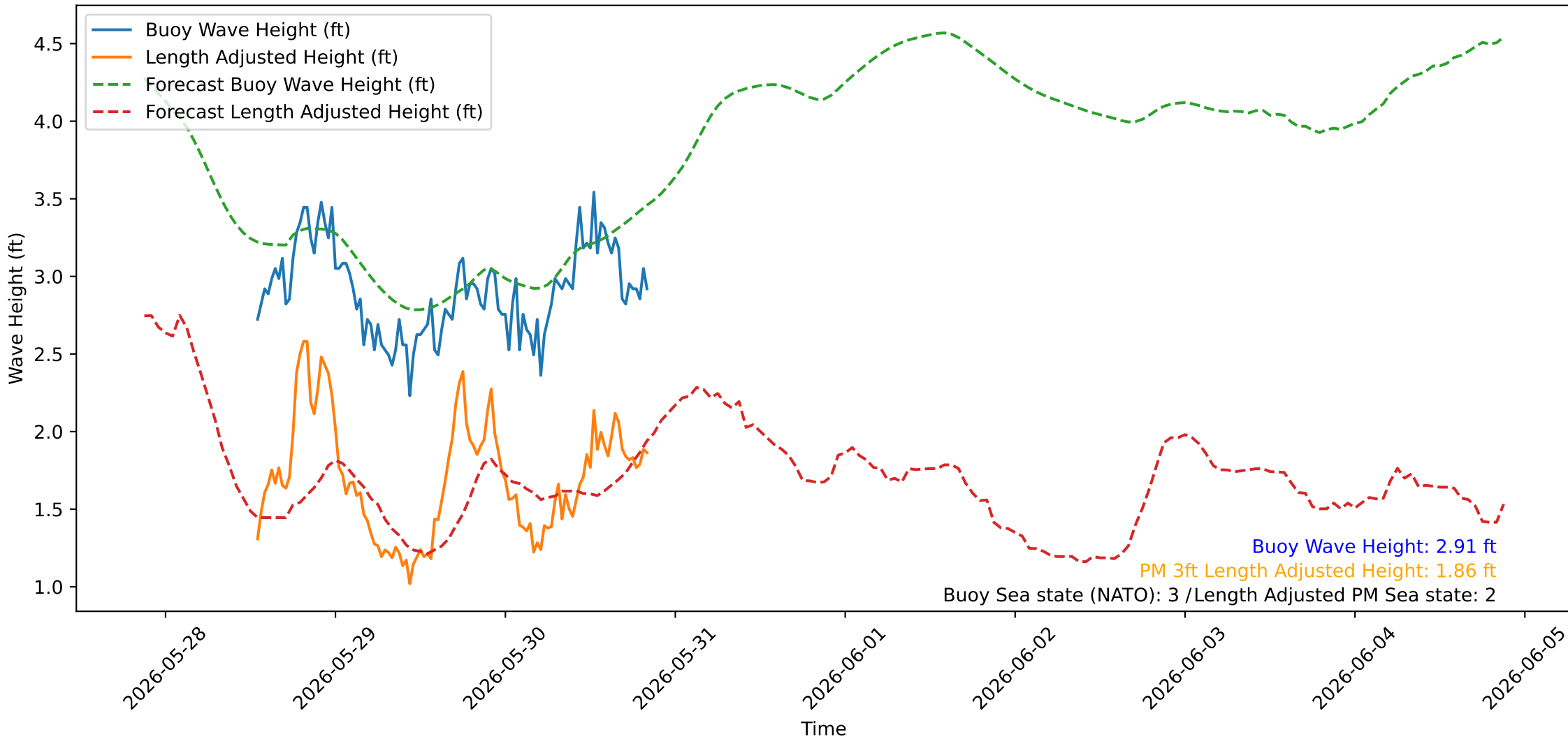
Wave Heights over Time for Oceanside Harbor at 2026-05-30 21:10:24
