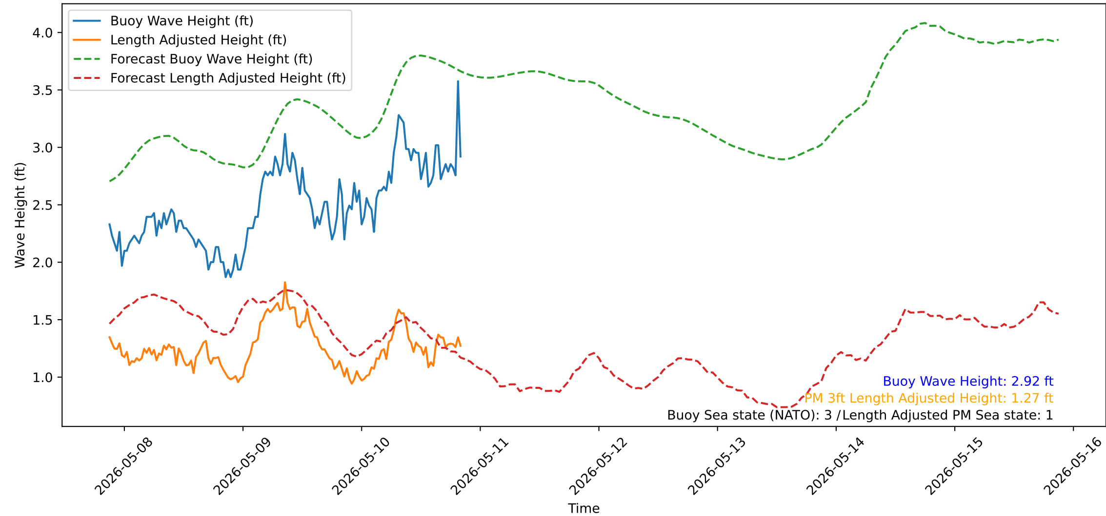
Wave Heights over Time for Oceanside Harbor at 2026-05-10 20:50:31
