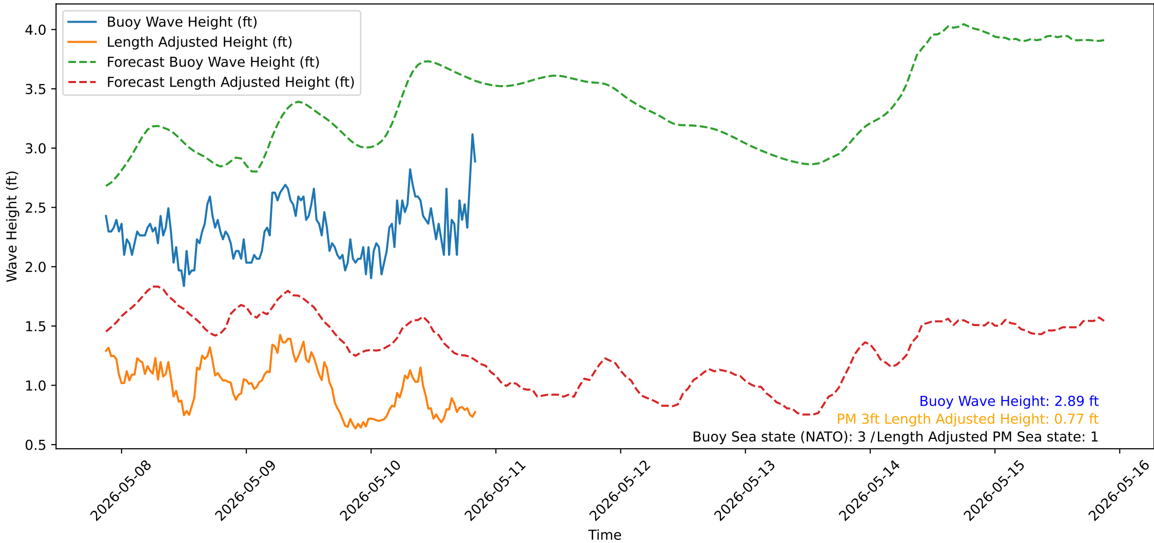
Wave Heights over Time for Green Beach at 2026-05-10 20:51:15
