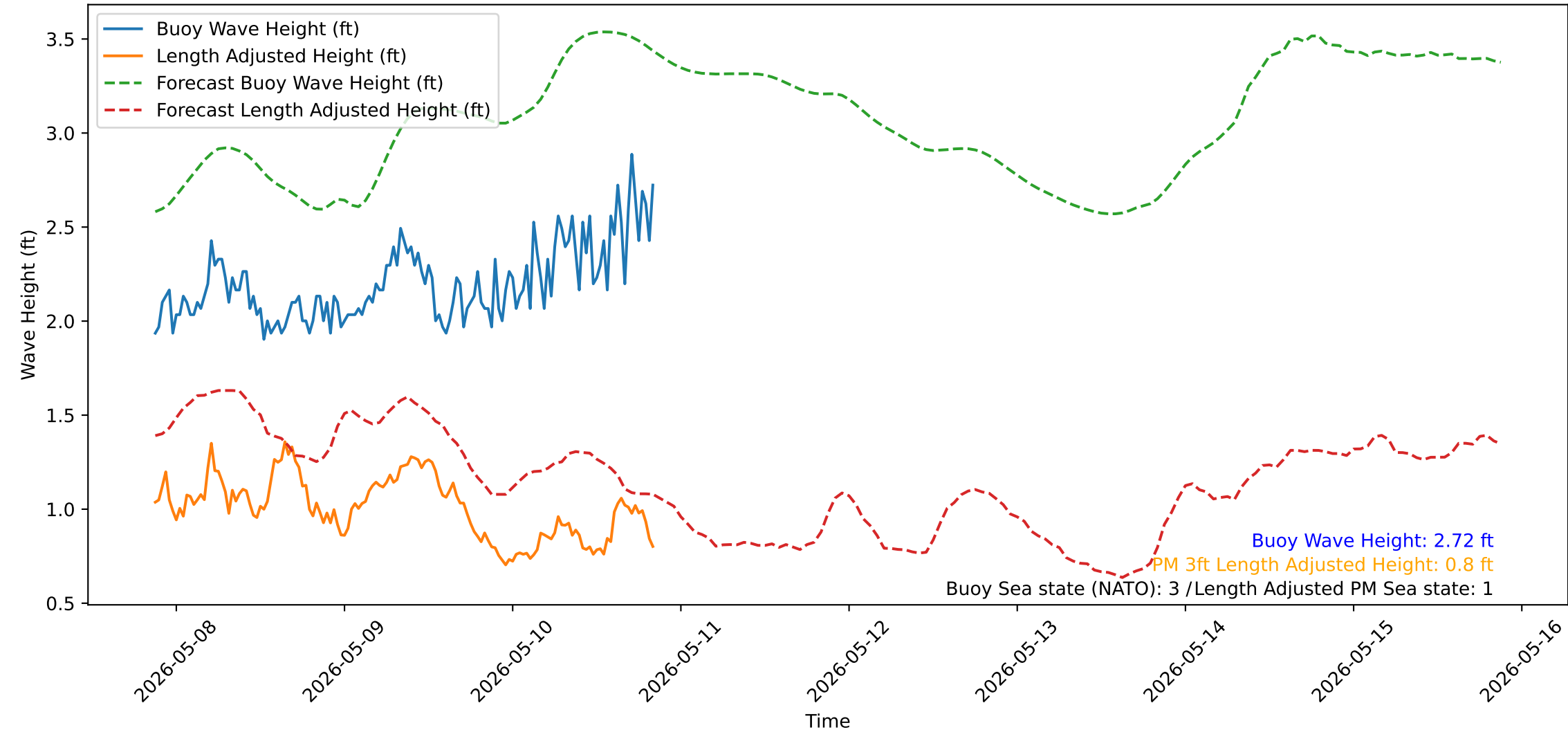
Wave Heights over Time for Red Beach at 2026-05-10 20:50:52
