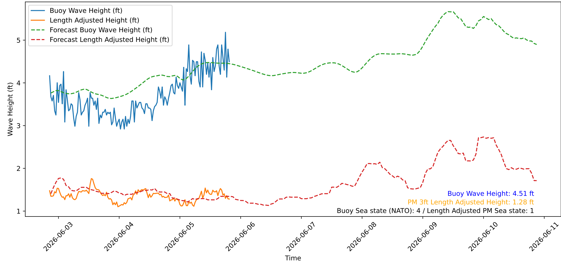
Wave Heights over Time for Oceanside Harbor at 2026-06-05 20:30:26
