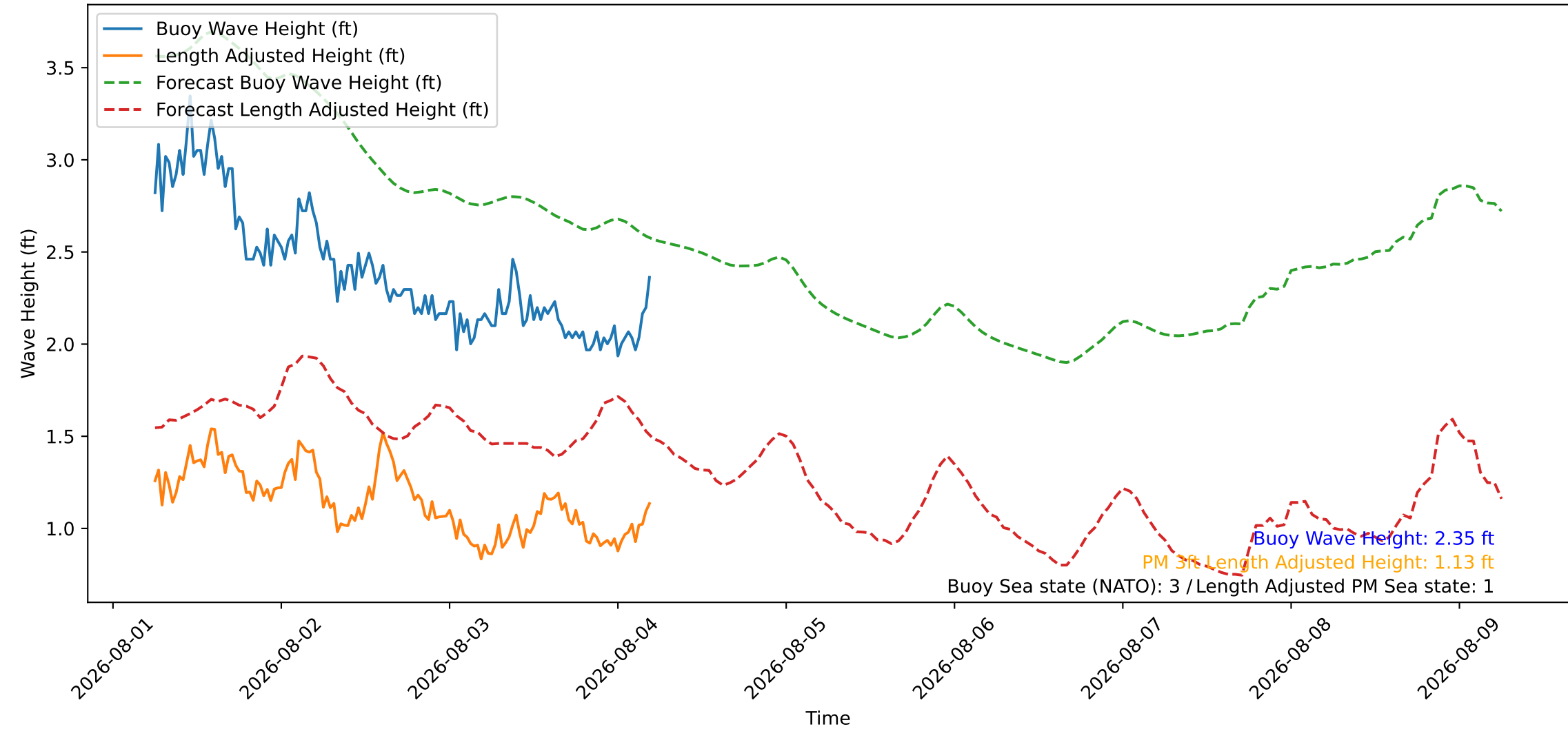
Wave Heights over Time for Red Beach at 2026-08-04 05:30:45
