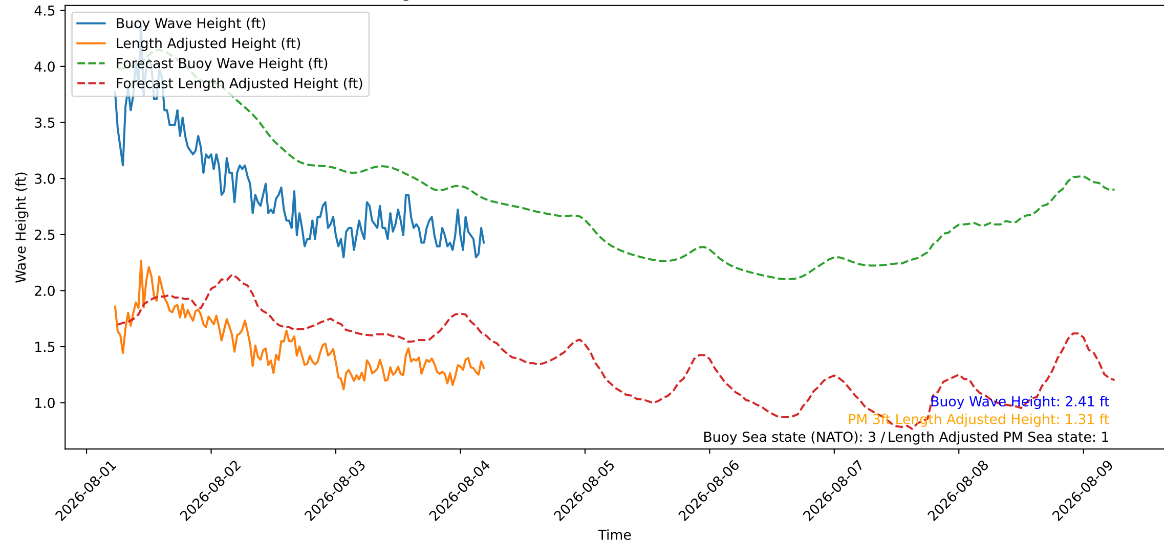
Wave Heights over Time for Oceanside Harbor at 2026-08-04 05:30:26
