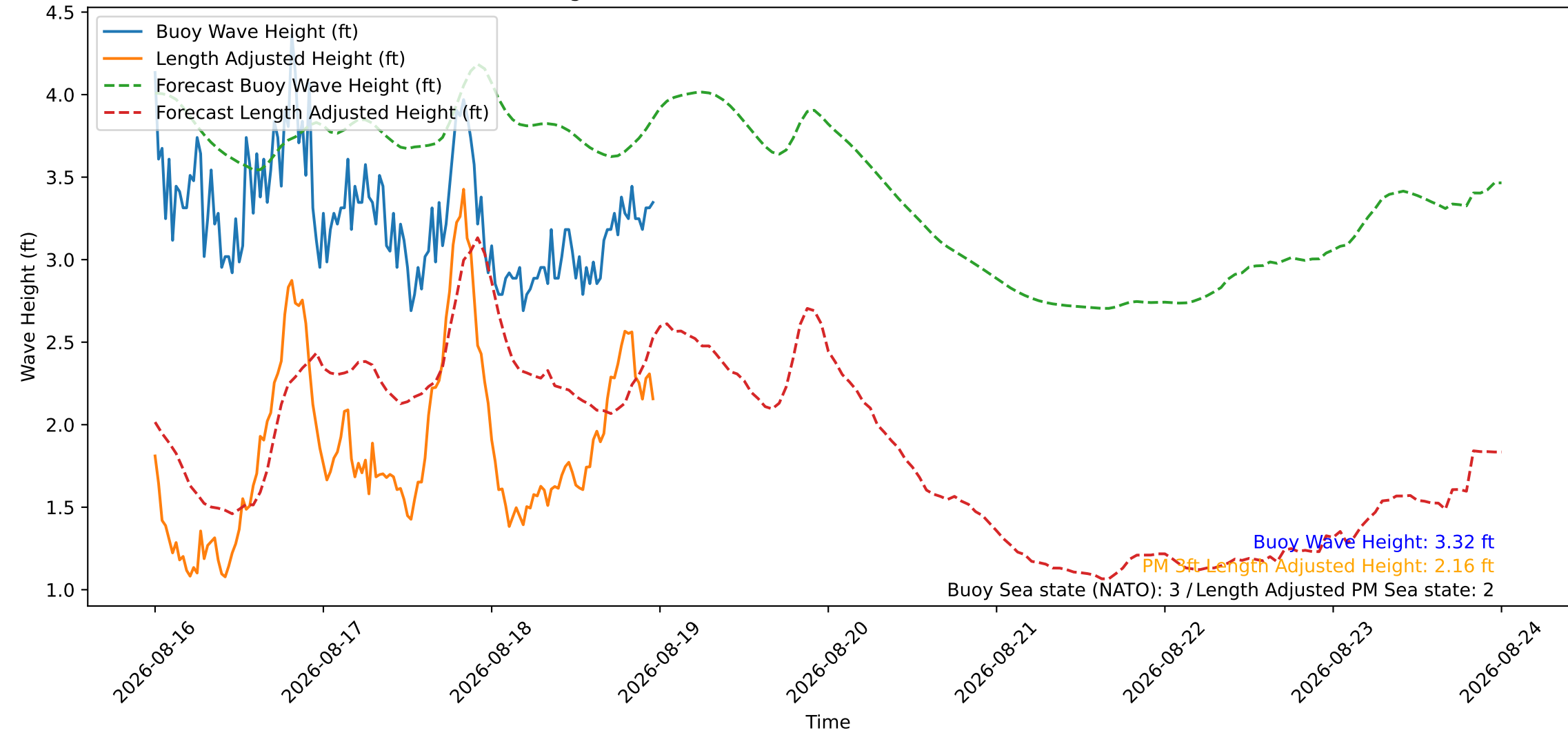
Wave Heights over Time for Green Beach at 2026-08-18 23:41:08
