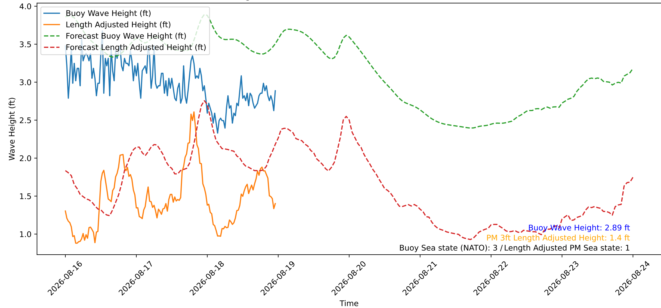
Wave Heights over Time for Red Beach at 2026-08-18 23:40:46
