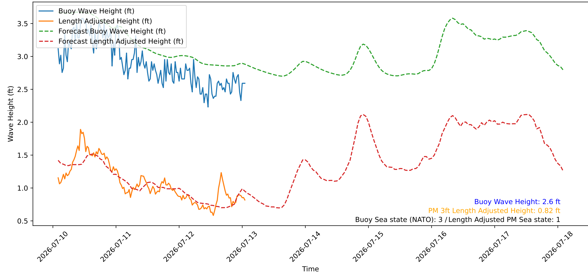
Wave Heights over Time for Green Beach at 2026-07-13 01:51:09
