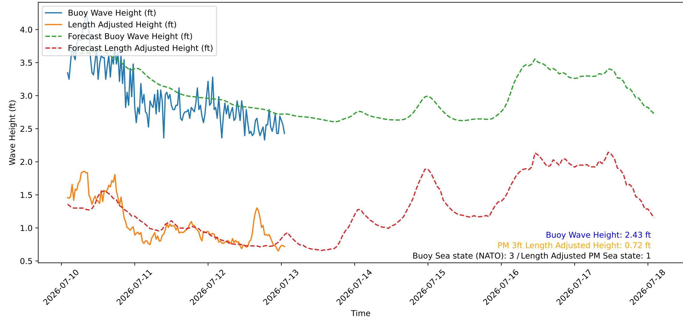
Wave Heights over Time for Oceanside Harbor at 2026-07-13 01:50:26
