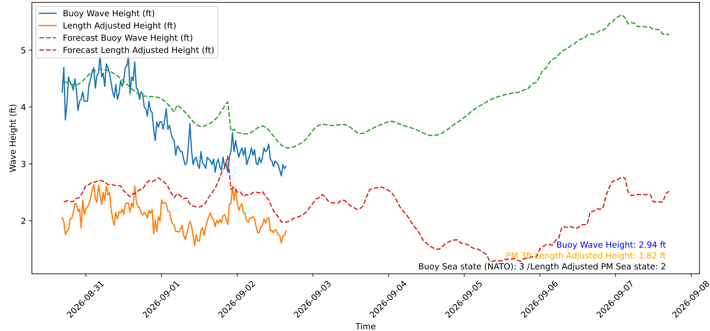
Wave Heights over Time for Oceanside Harbor at 2026-09-02 16:30:30
