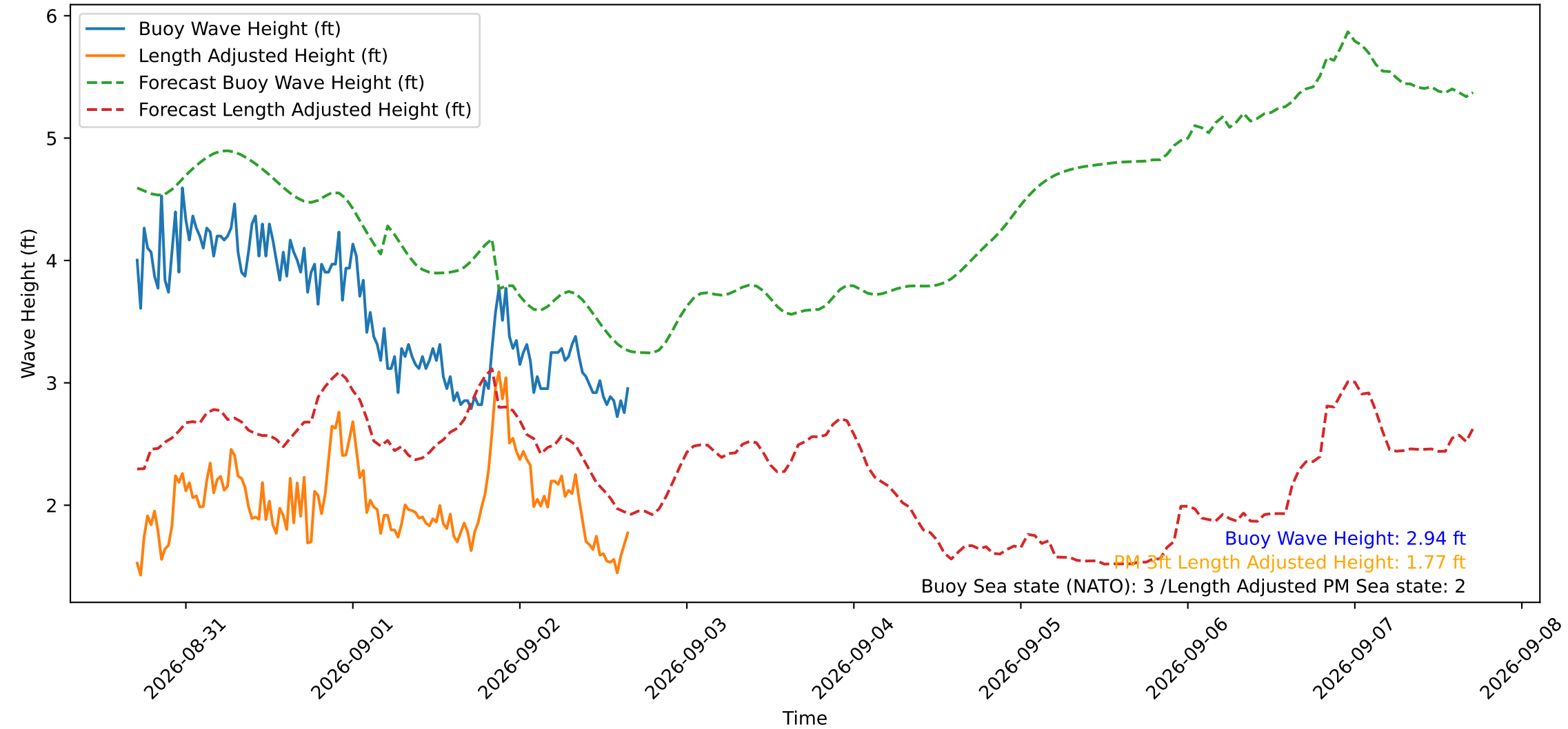
Wave Heights over Time for Green Beach at 2026-09-02 16:31:12
