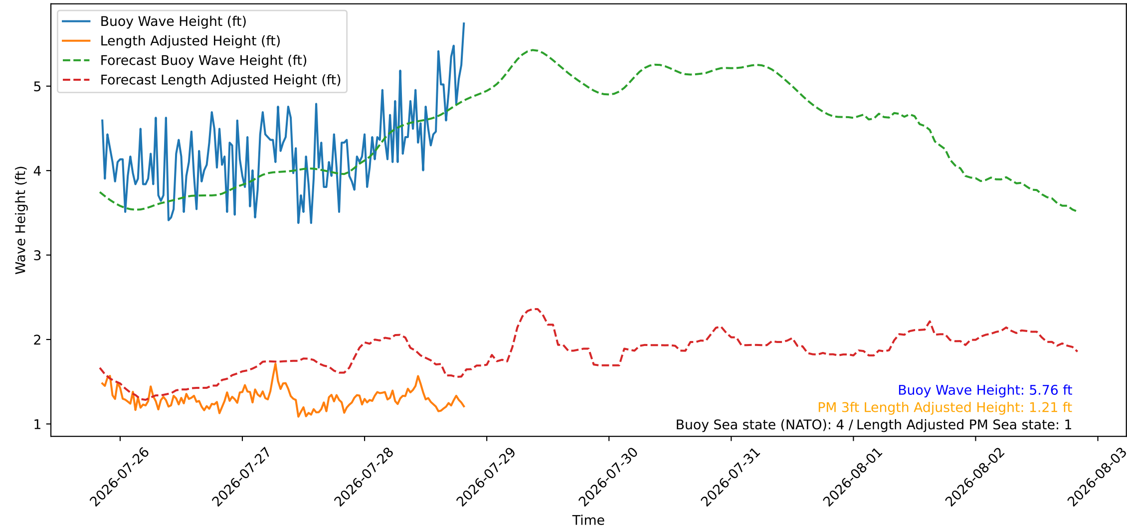
Wave Heights over Time for Green Beach at 2026-07-28 20:21:09
