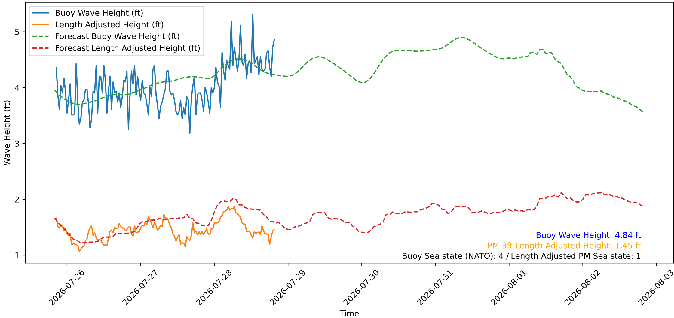
Wave Heights over Time for Oceanside Harbor at 2026-07-28 20:20:26
