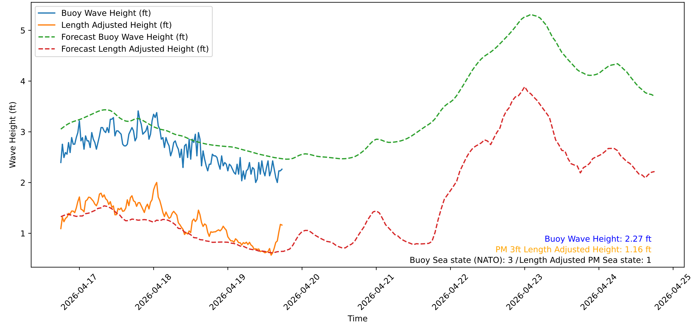
Wave Heights over Time for Oceanside Harbor at 2026-04-19 18:10:31
