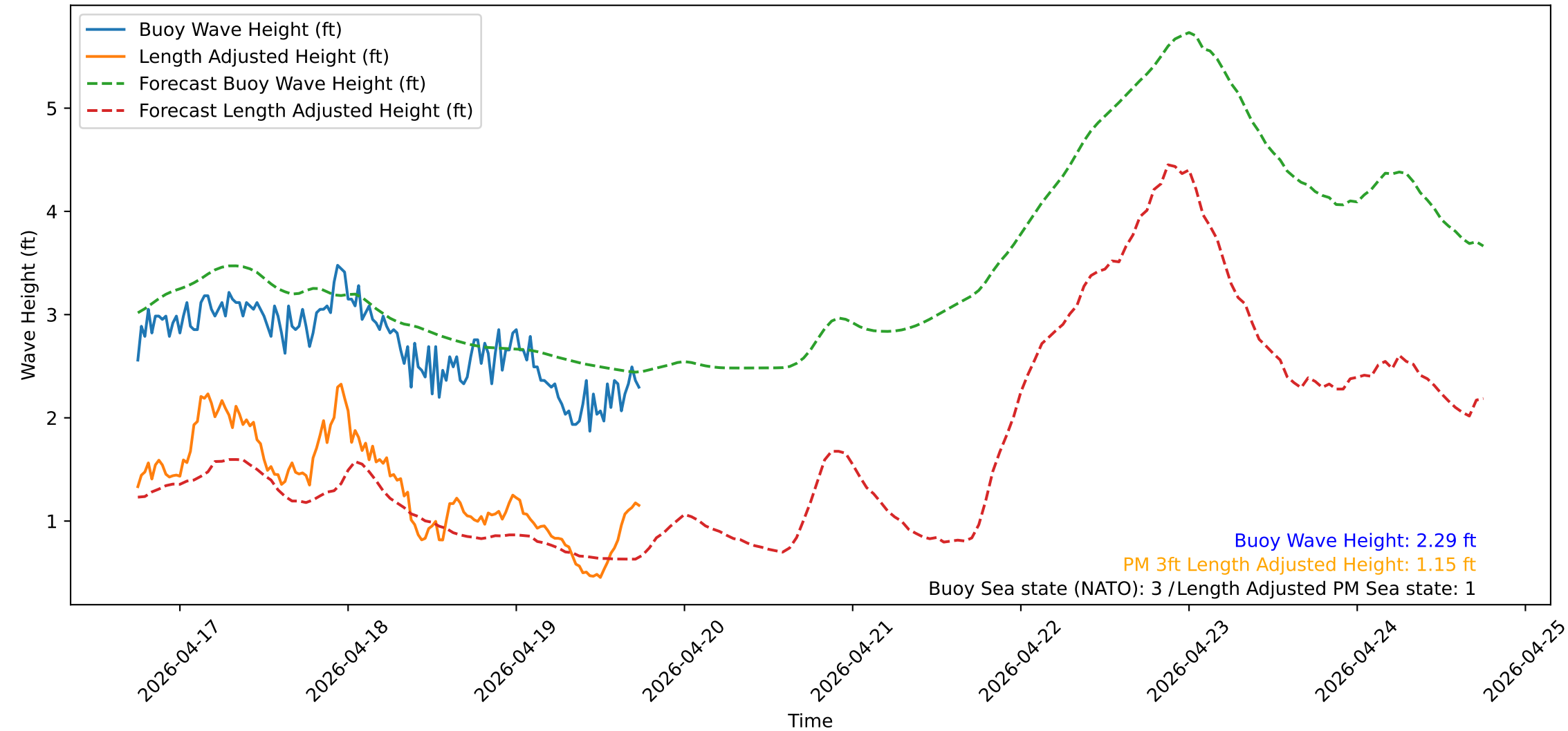
Wave Heights over Time for Green Beach at 2026-04-19 18:11:13
