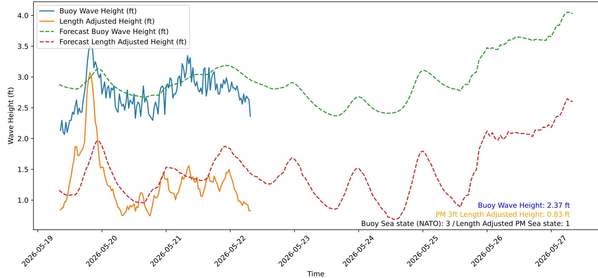
Wave Heights over Time for Red Beach at 2026-05-22 08:20:52
