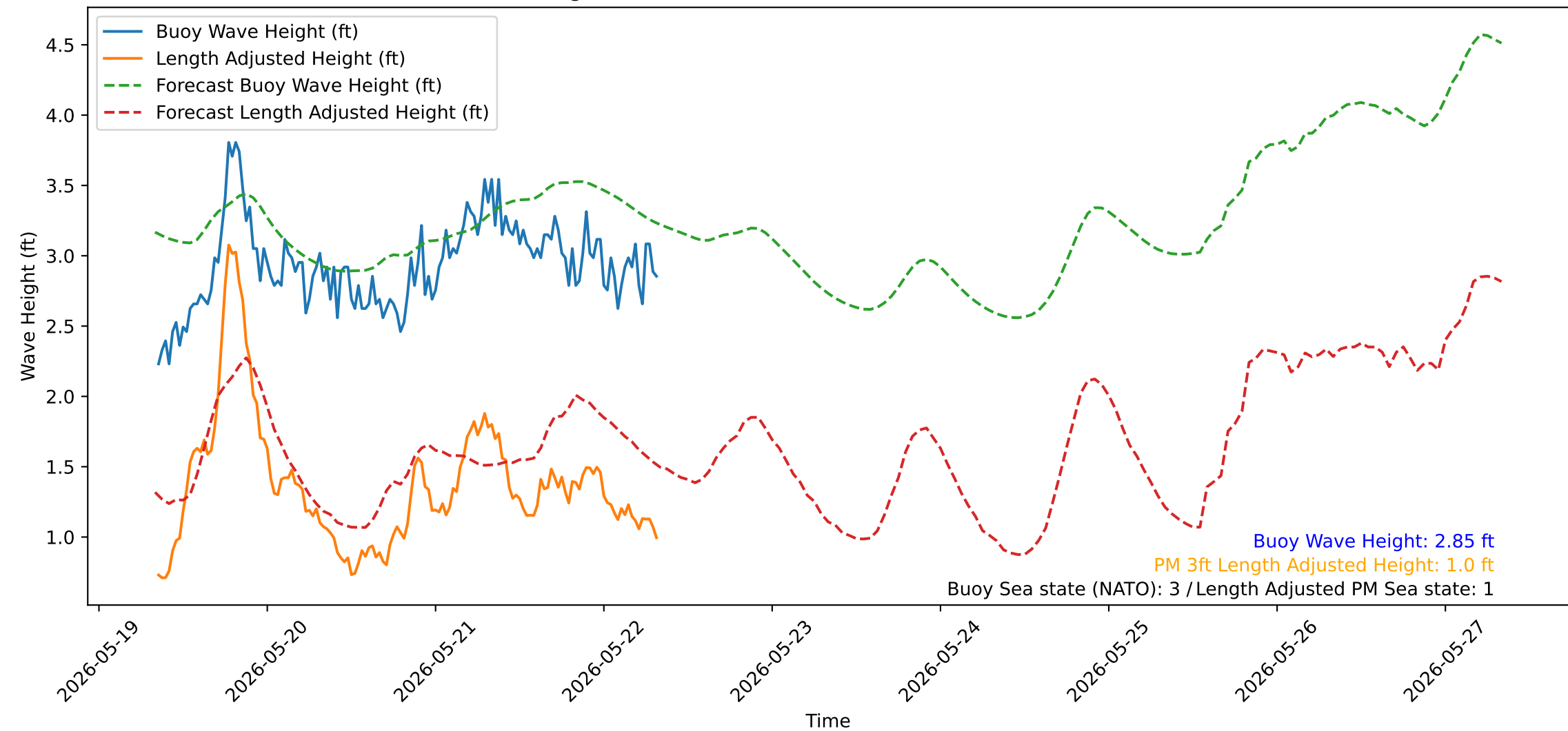
Wave Heights over Time for Green Beach at 2026-05-22 08:21:15
