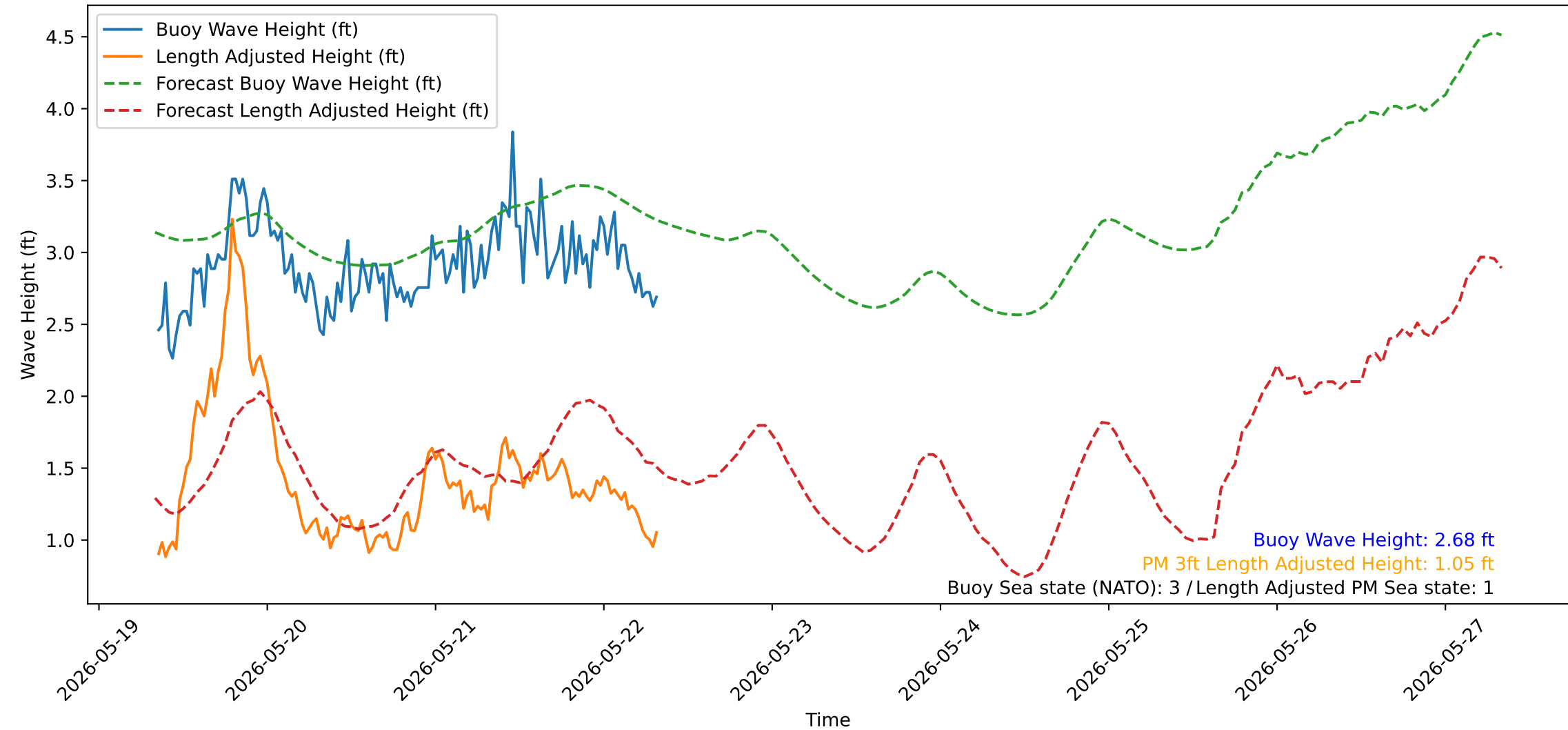
Wave Heights over Time for Oceanside Harbor at 2026-05-22 08:20:31
