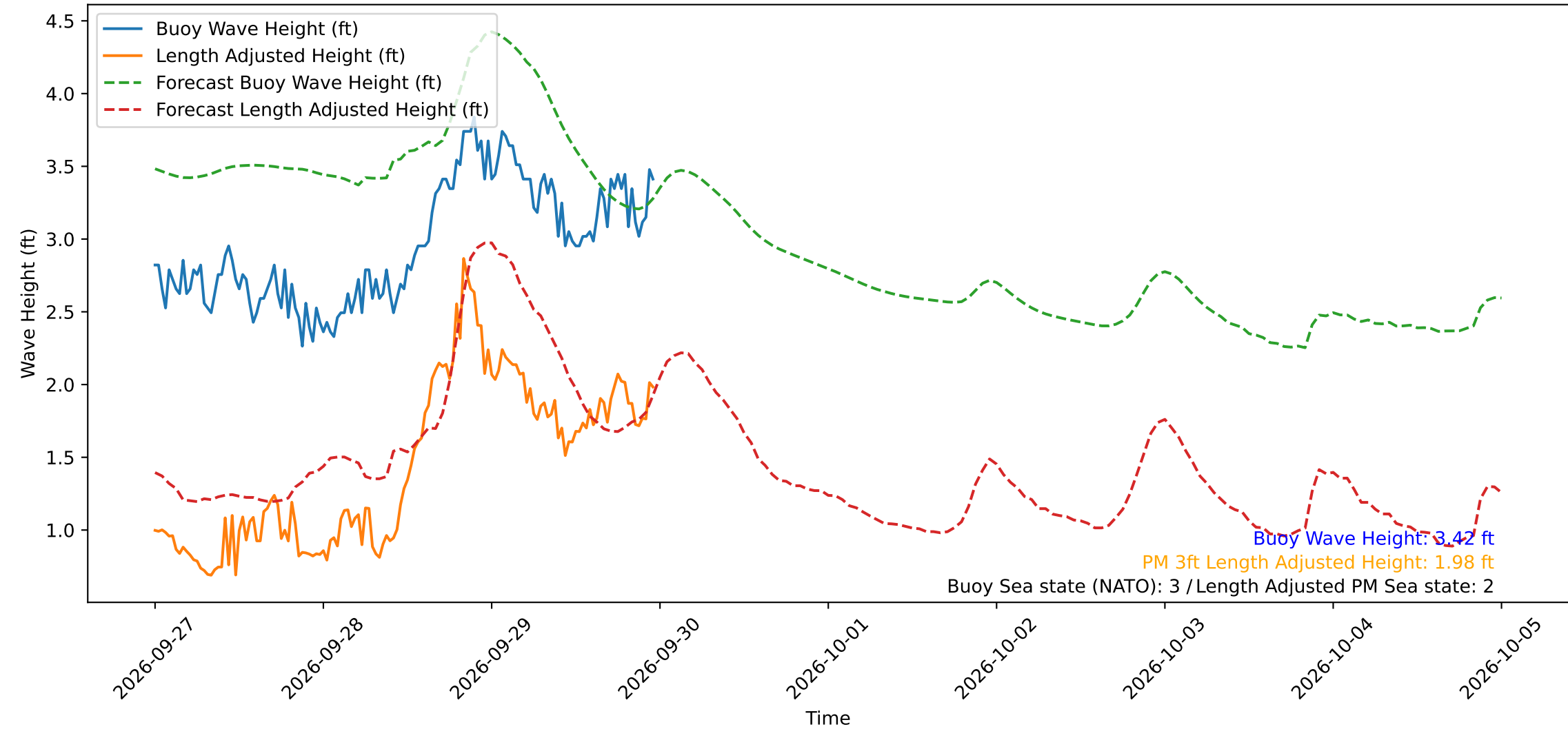
Wave Heights over Time for Red Beach at 2026-09-29 23:50:51
