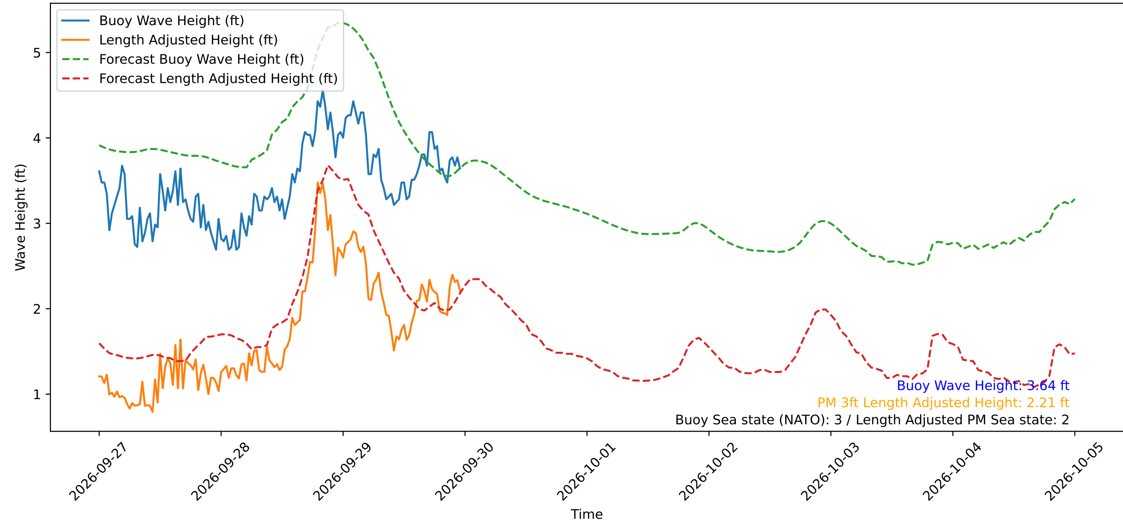
Wave Heights over Time for Green Beach at 2026-09-29 23:51:15
