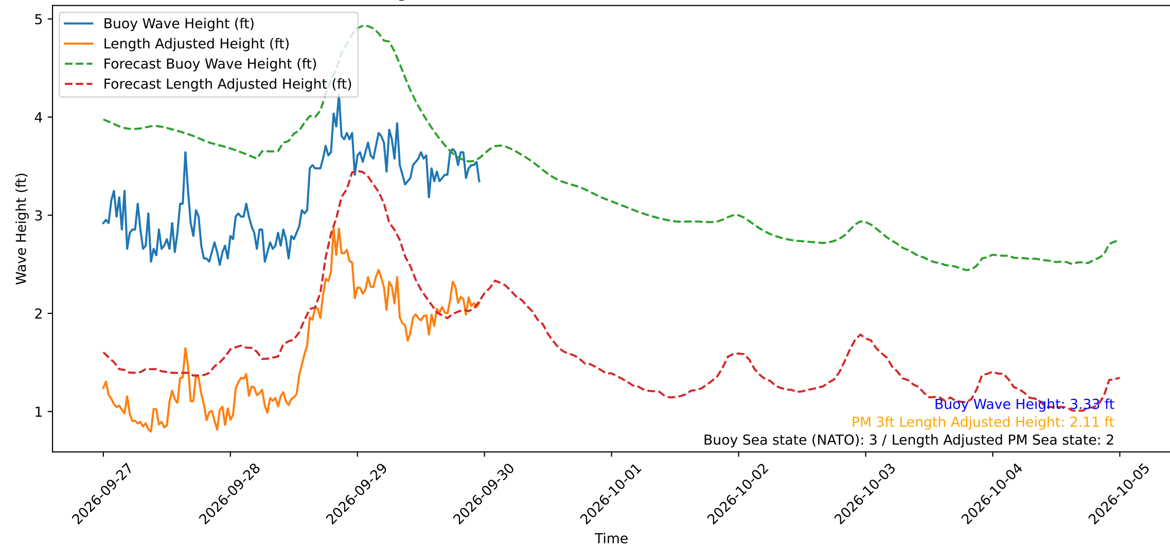
Wave Heights over Time for Oceanside Harbor at 2026-09-29 23:50:30
