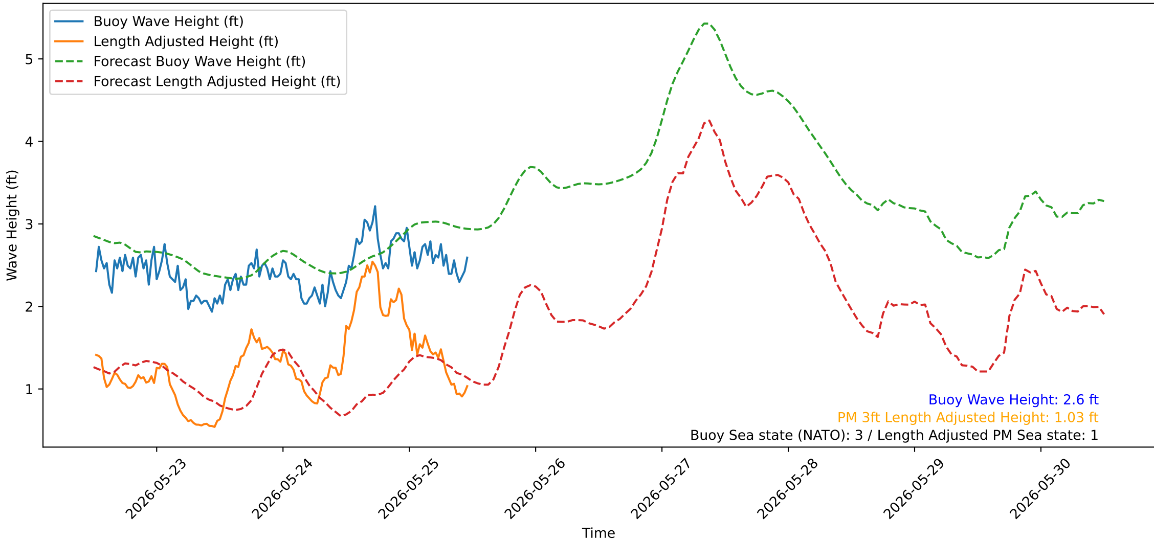
Wave Heights over Time for Red Beach at 2026-05-25 12:00:50
