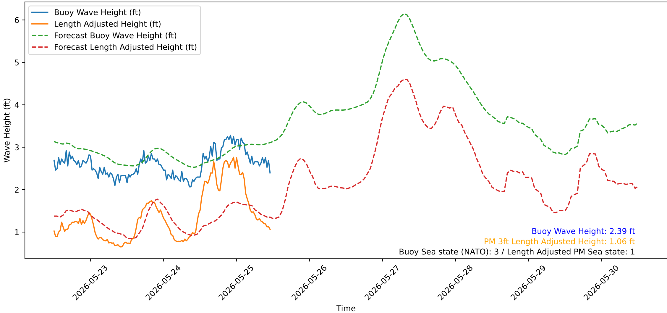
Wave Heights over Time for Green Beach at 2026-05-25 12:01:13
