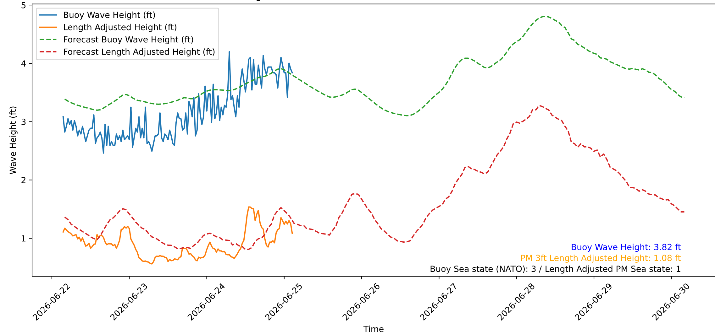
Wave Heights over Time for Green Beach at 2026-06-25 03:31:07
