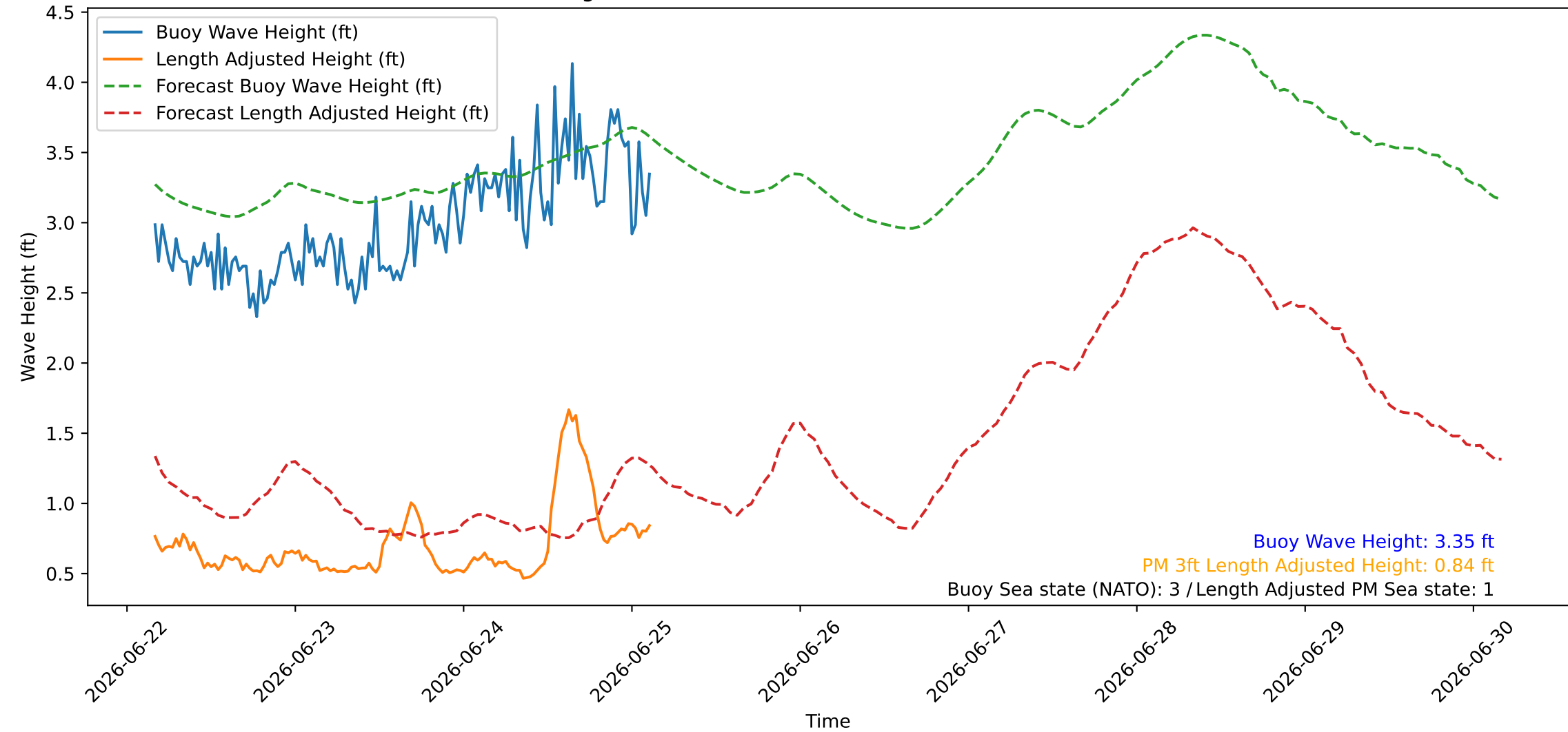
Wave Heights over Time for Red Beach at 2026-06-25 03:30:45
