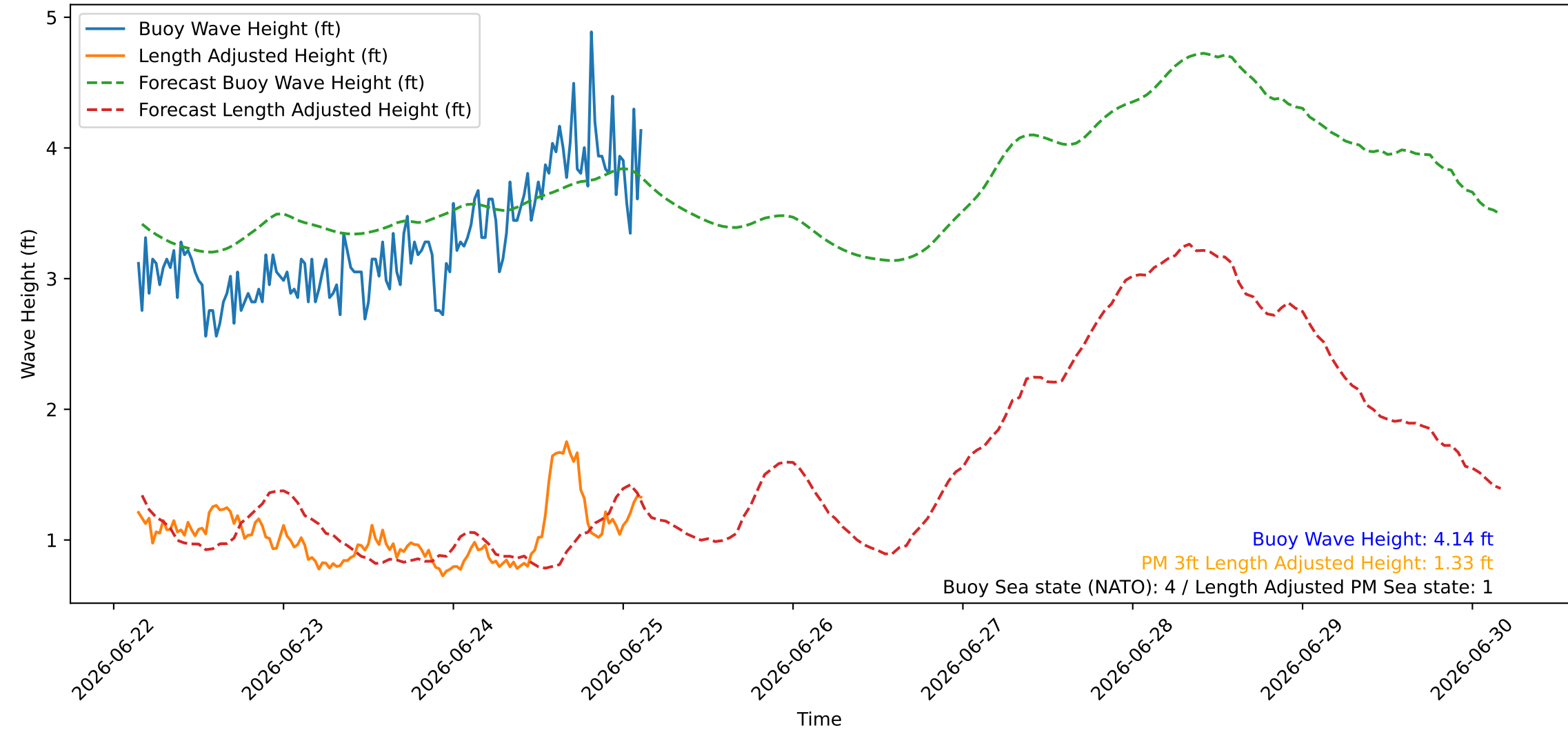
Wave Heights over Time for Oceanside Harbor at 2026-06-25 03:30:26
