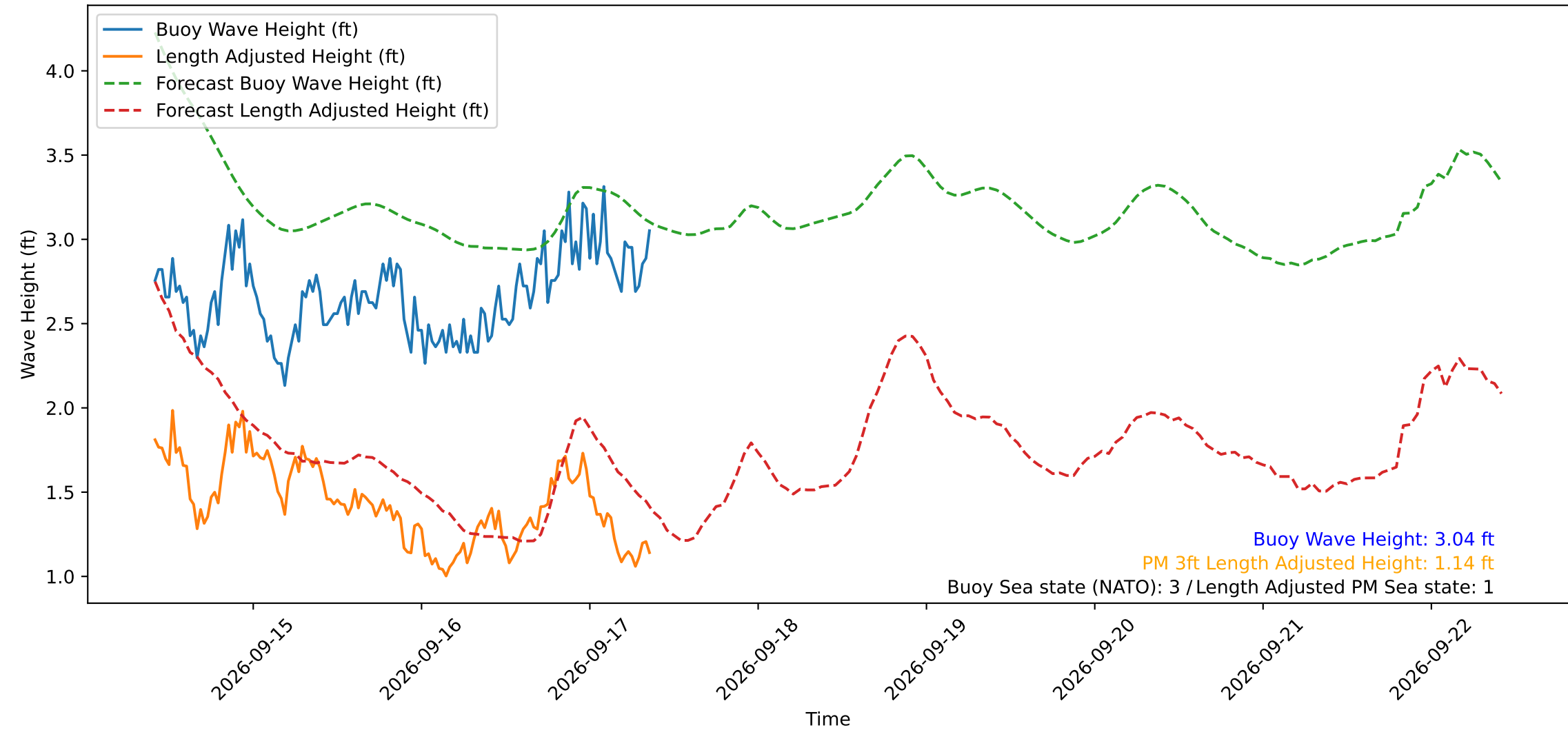
Wave Heights over Time for Green Beach at 2026-09-17 09:31:12
