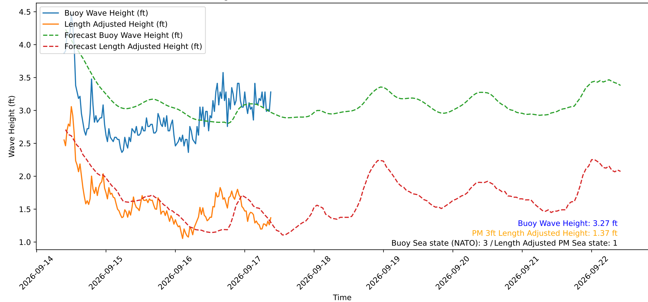
Wave Heights over Time for Oceanside Harbor at 2026-09-17 09:30:30
