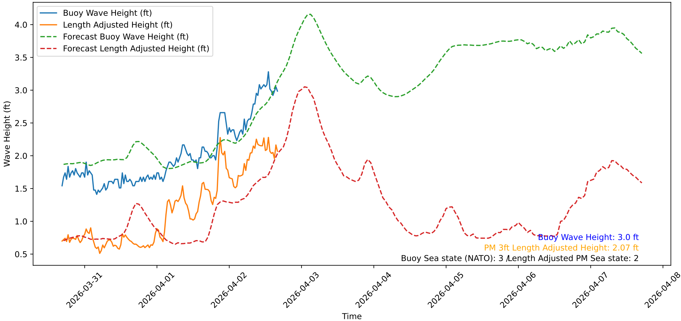
Wave Heights over Time for Green Beach at 2026-04-02 16:41:09
