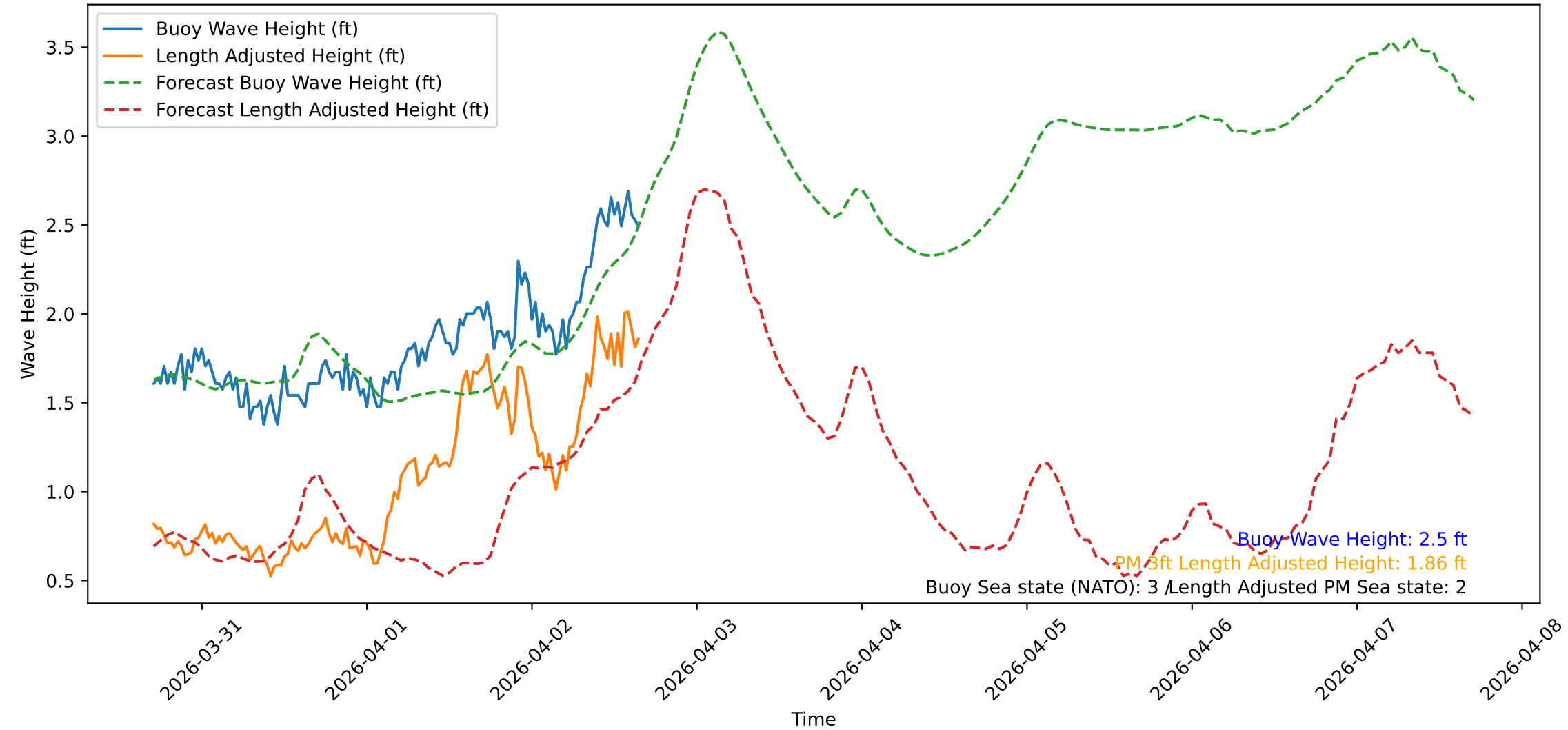
Wave Heights over Time for Red Beach at 2026-04-02 16:40:47
