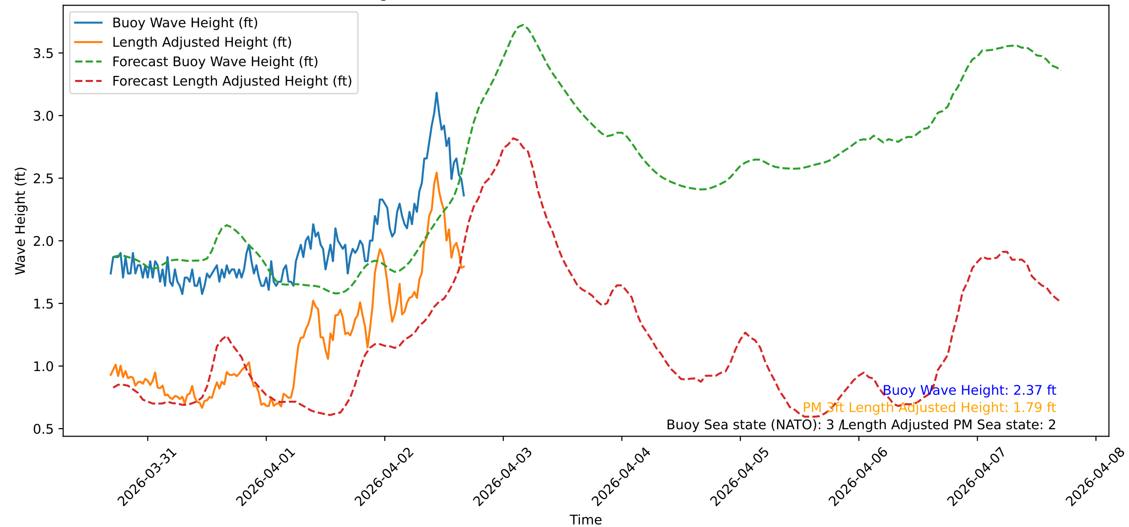
Wave Heights over Time for Oceanside Harbor at 2026-04-02 16:40:31
