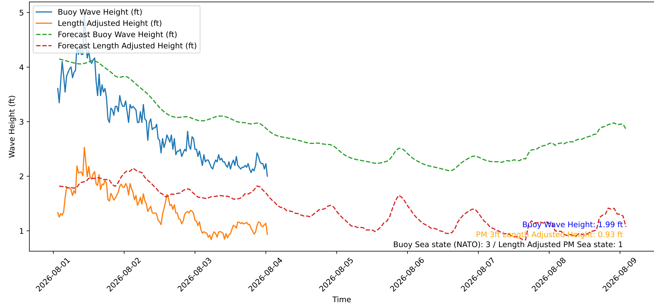
Wave Heights over Time for Green Beach at 2026-08-04 01:31:08
