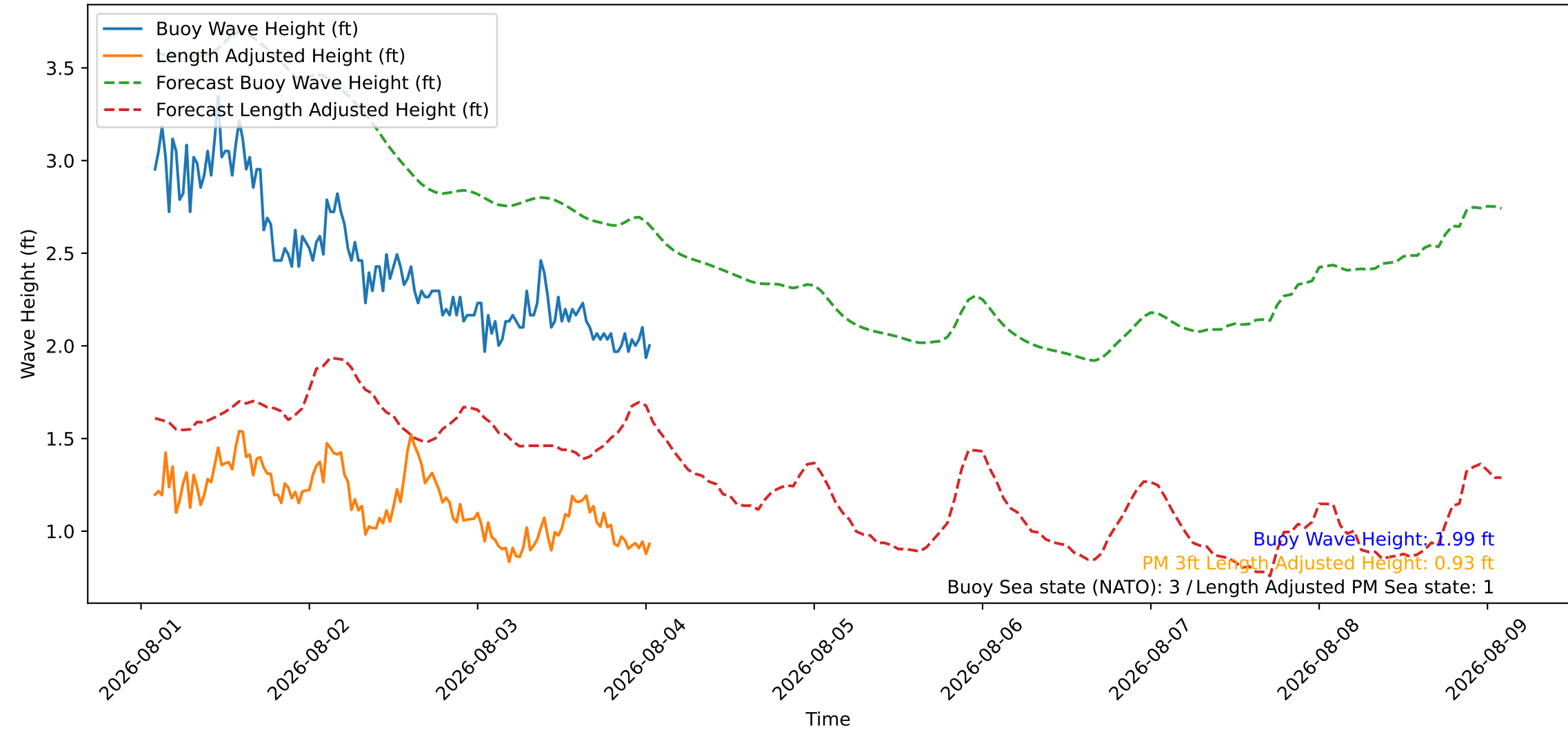
Wave Heights over Time for Red Beach at 2026-08-04 01:30:46
