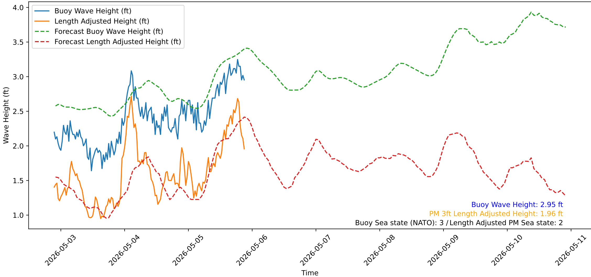
Wave Heights over Time for Oceanside Harbor at 2026-05-05 21:40:31
