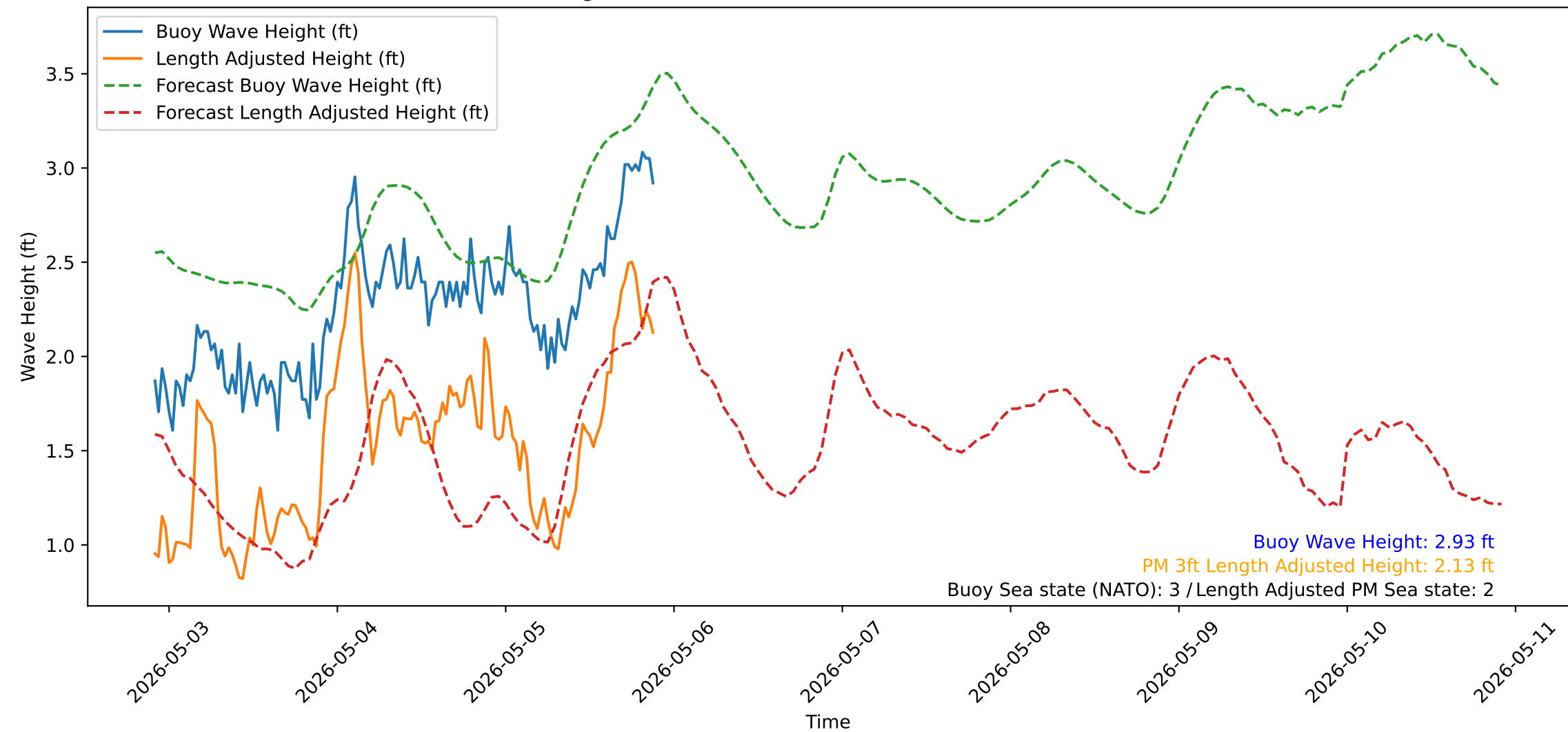
Wave Heights over Time for Red Beach at 2026-05-05 21:40:51
