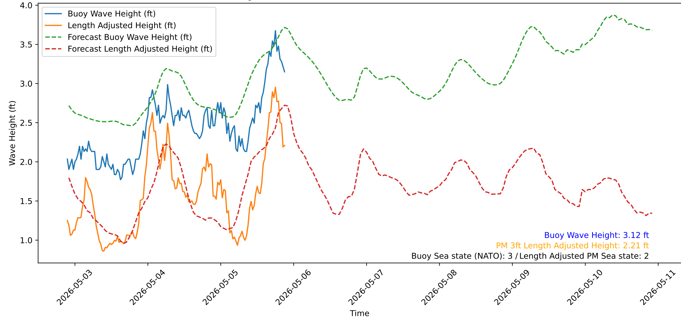
Wave Heights over Time for Green Beach at 2026-05-05 21:41:14
