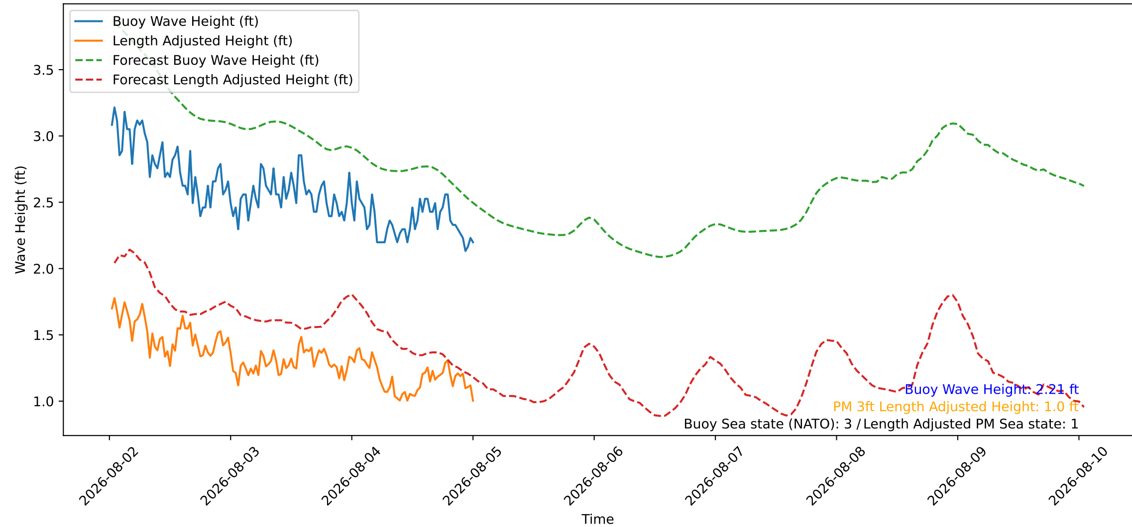
Wave Heights over Time for Oceanside Harbor at 2026-08-05 00:30:27
