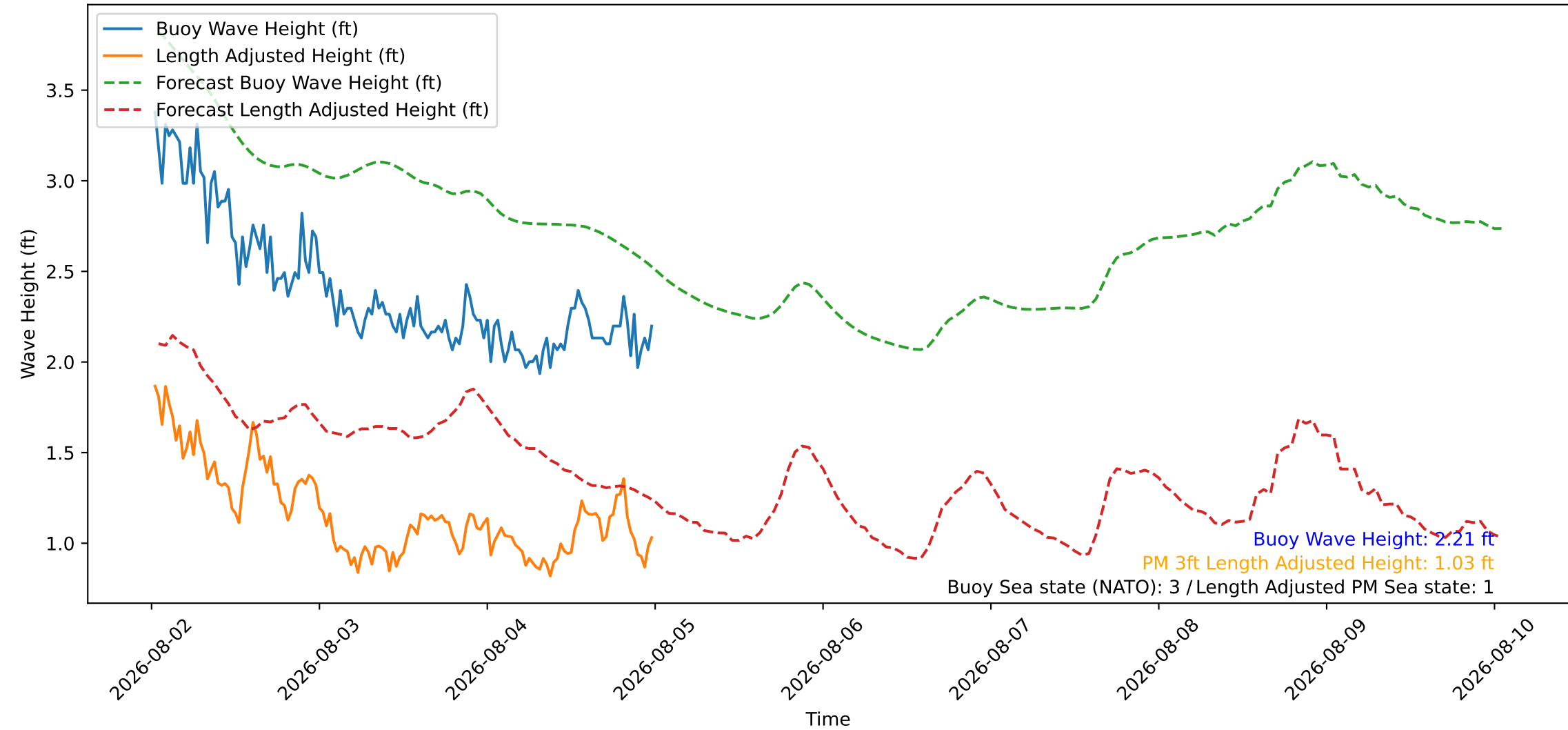
Wave Heights over Time for Green Beach at 2026-08-05 00:31:09
