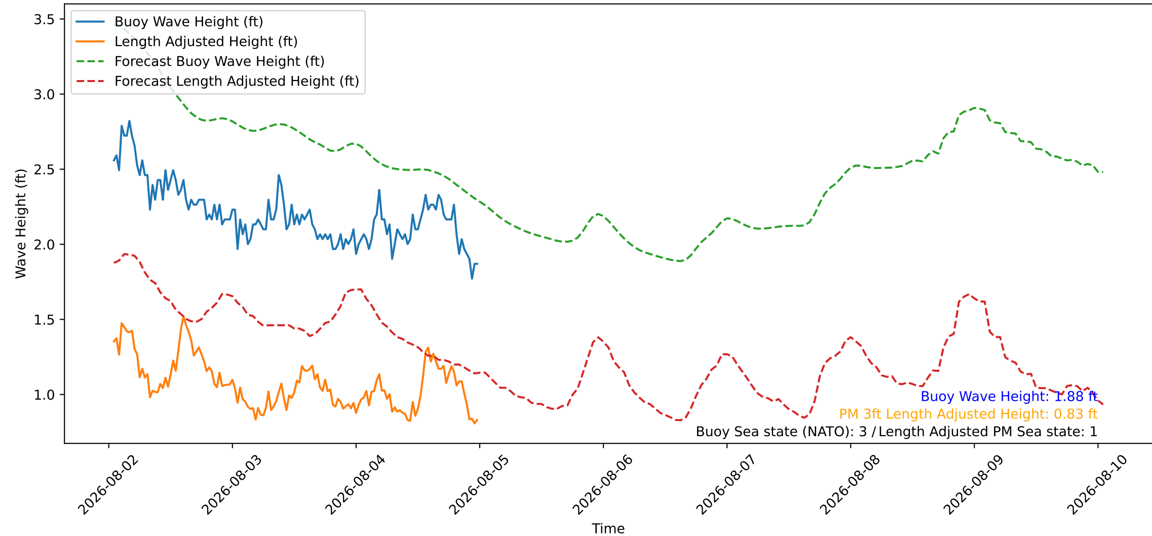
Wave Heights over Time for Red Beach at 2026-08-05 00:30:46
