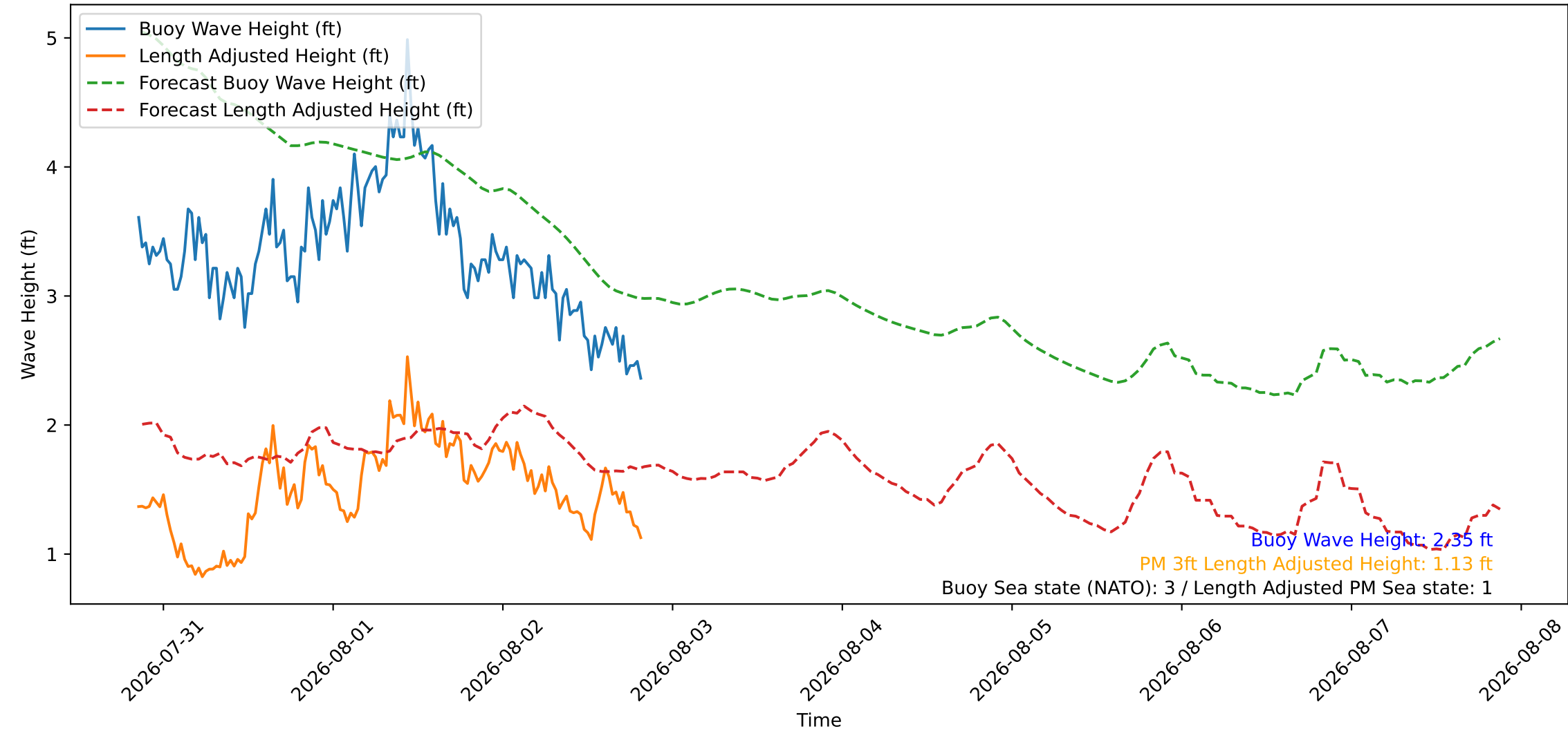
Wave Heights over Time for Green Beach at 2026-08-02 20:31:09
