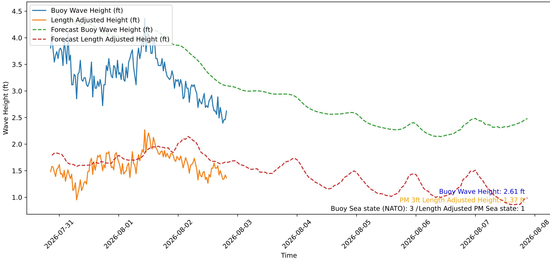
Wave Heights over Time for Oceanside Harbor at 2026-08-02 20:30:26
