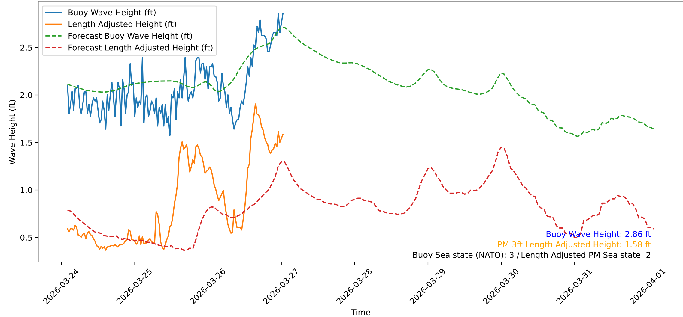
Wave Heights over Time for Red Beach at 2026-03-27 01:30:47
