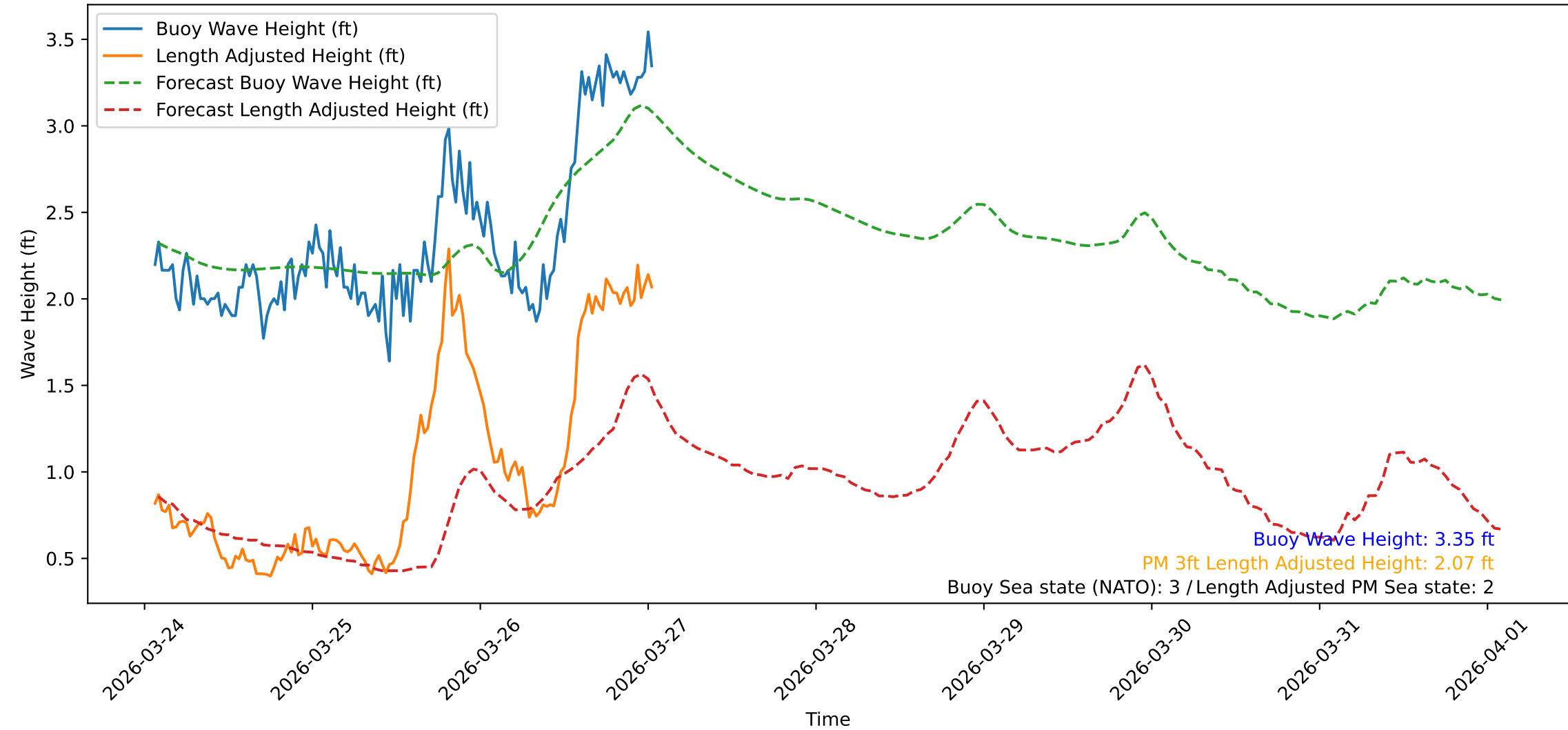
Wave Heights over Time for Green Beach at 2026-03-27 01:31:09
