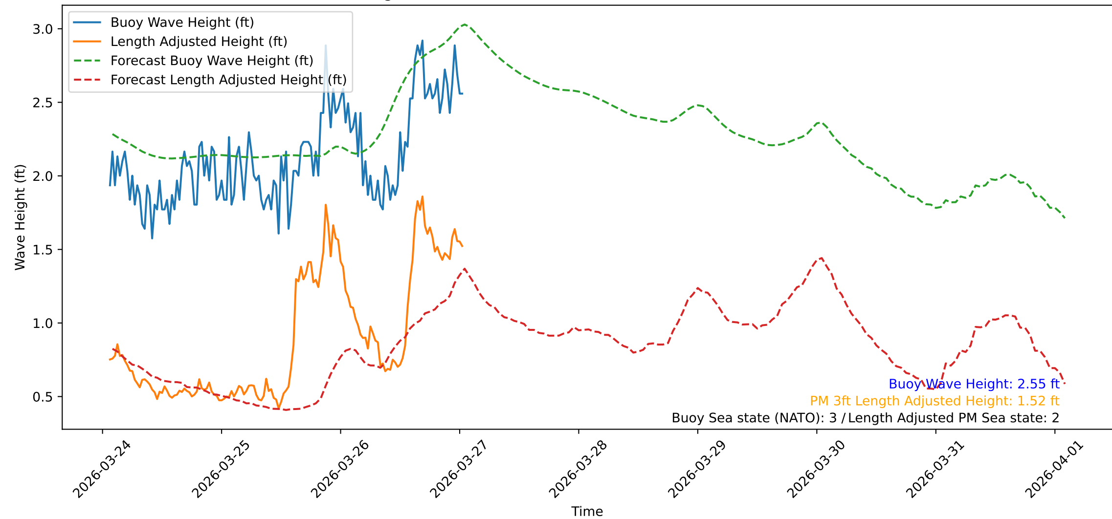
Wave Heights over Time for Oceanside Harbor at 2026-03-27 01:30:31
