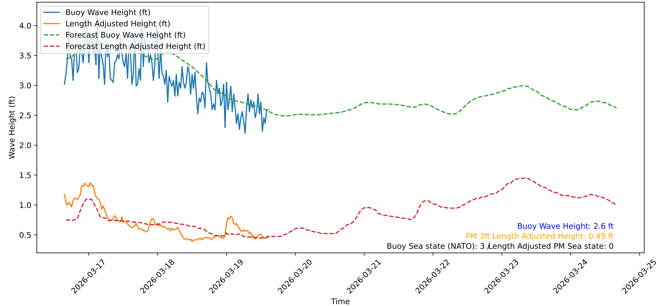
Wave Heights over Time for Green Beach at 2026-03-19 15:31:10
