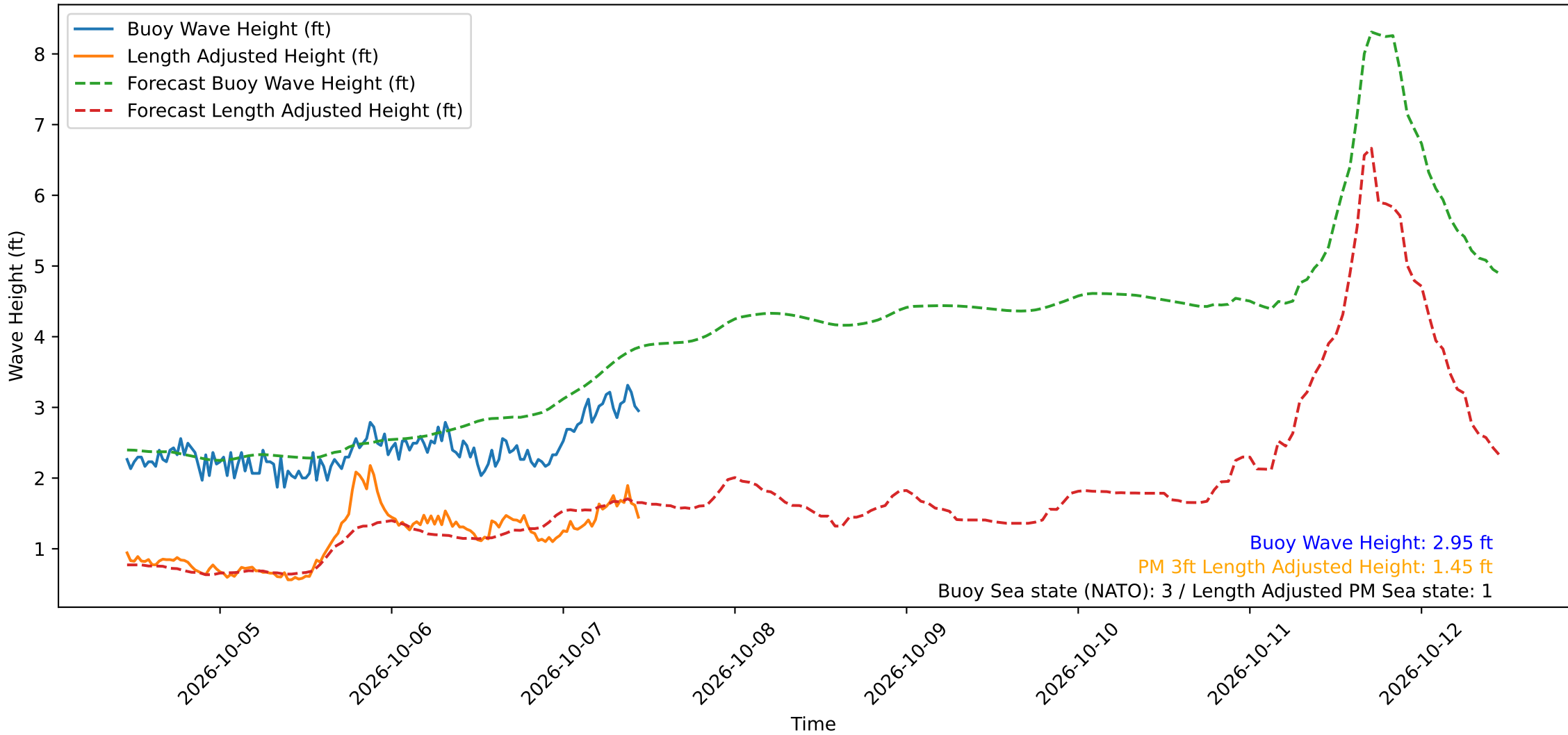
Wave Heights over Time for Oceanside Harbor at 2026-10-07 11:10:30
