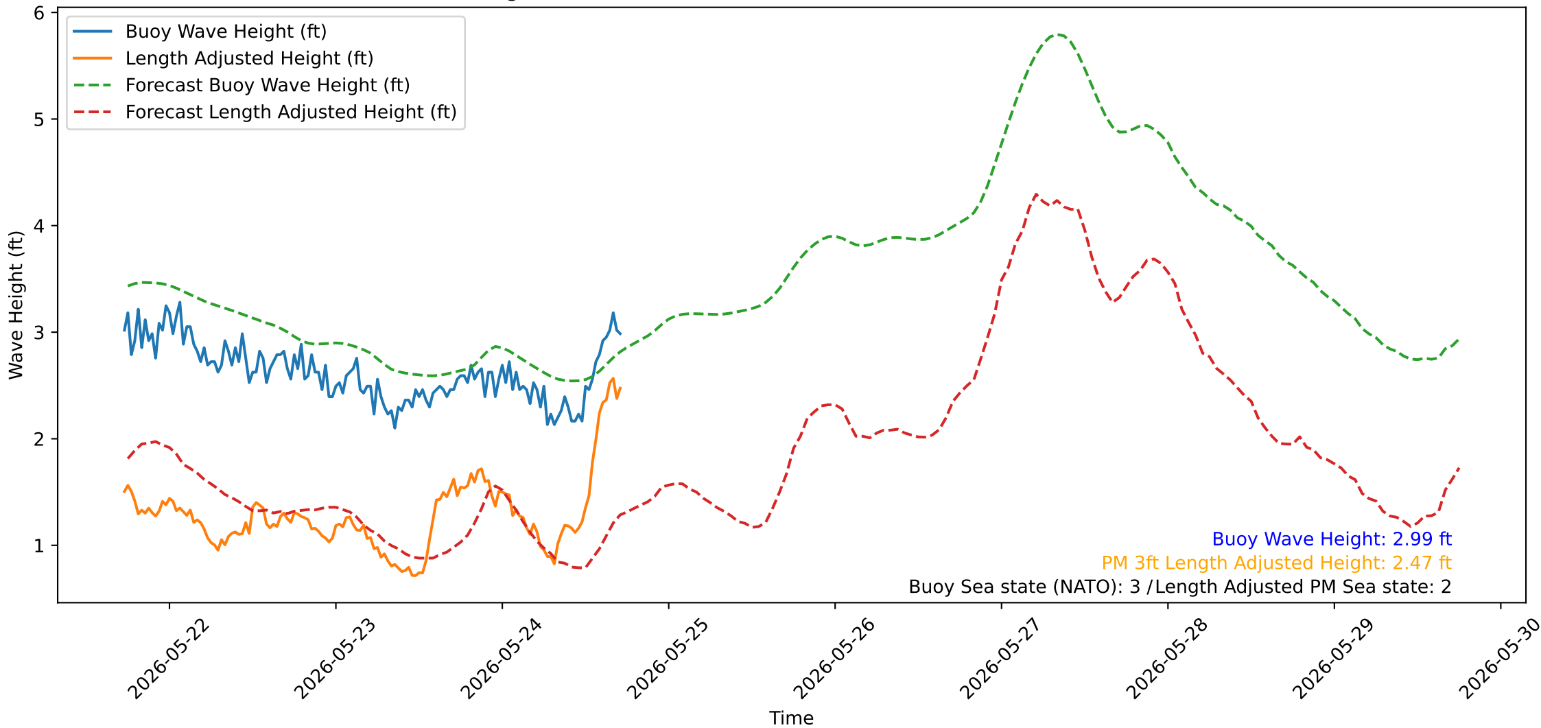
Wave Heights over Time for Oceanside Harbor at 2026-05-24 17:30:32
