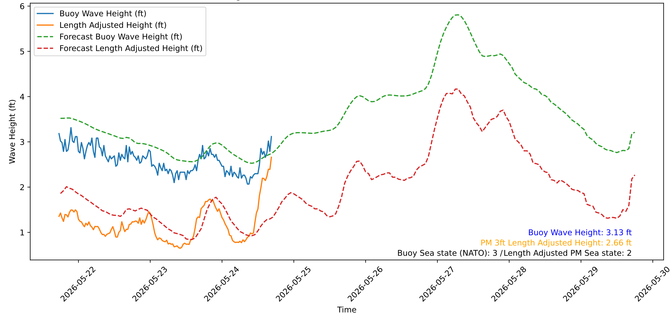
Wave Heights over Time for Green Beach at 2026-05-24 17:31:15
