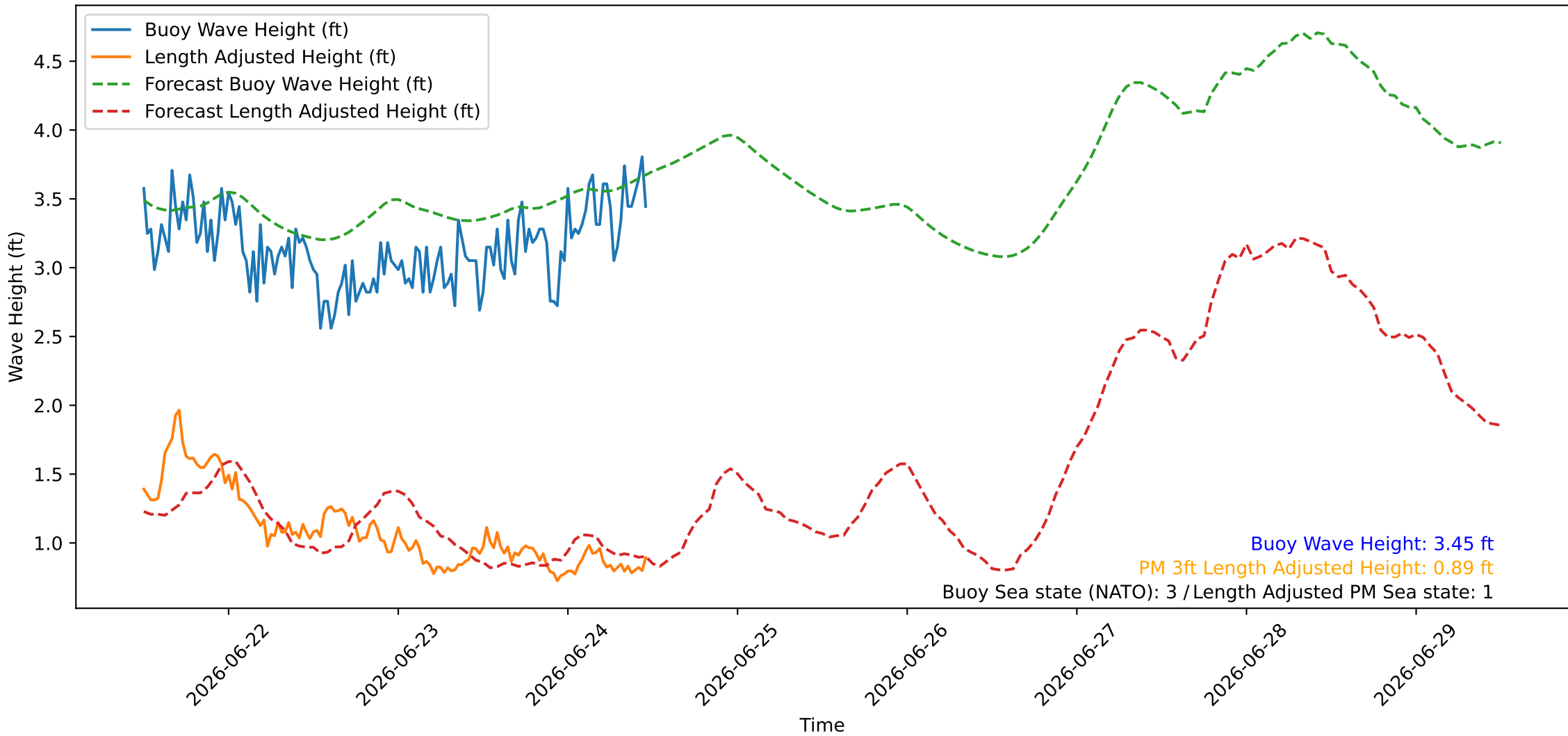
Wave Heights over Time for Oceanside Harbor at 2026-06-24 12:00:26
