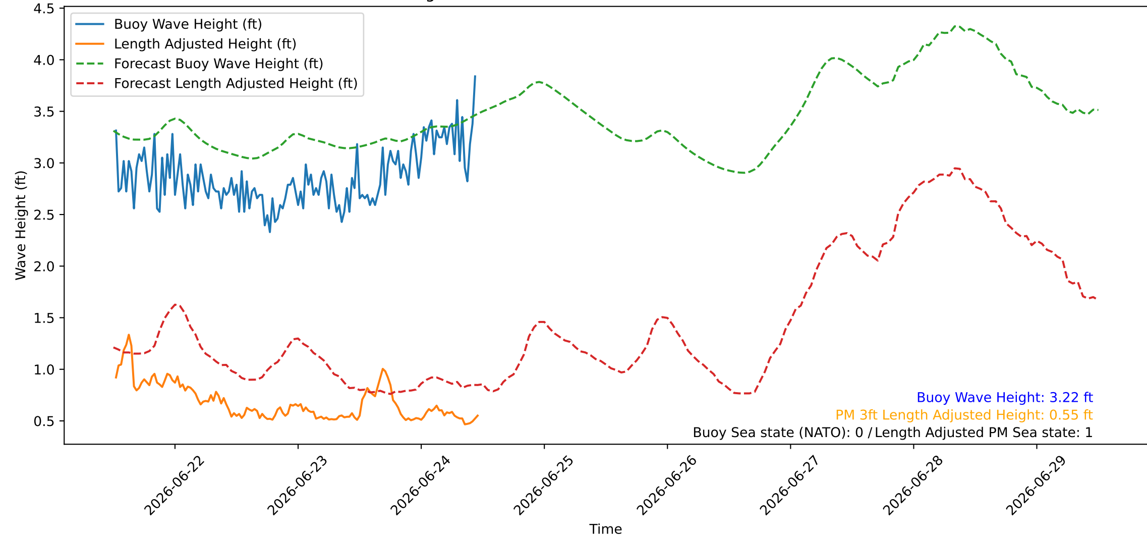
Wave Heights over Time for Red Beach at 2026-06-24 12:00:45
