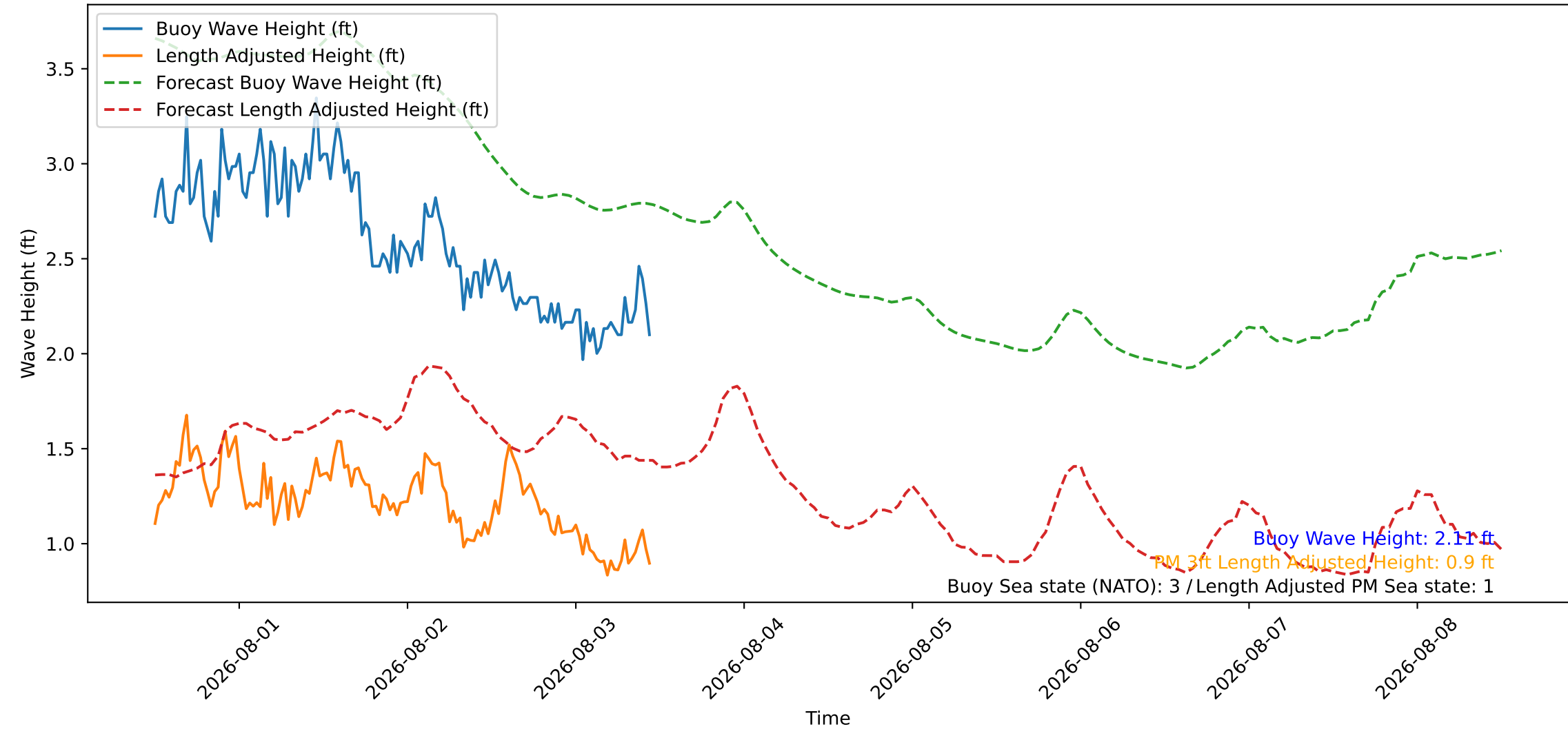
Wave Heights over Time for Red Beach at 2026-08-03 11:30:46
