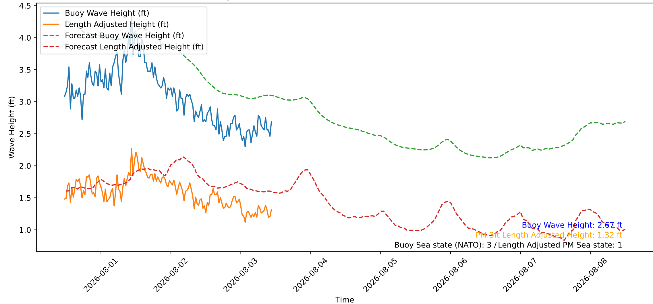
Wave Heights over Time for Oceanside Harbor at 2026-08-03 11:30:26
