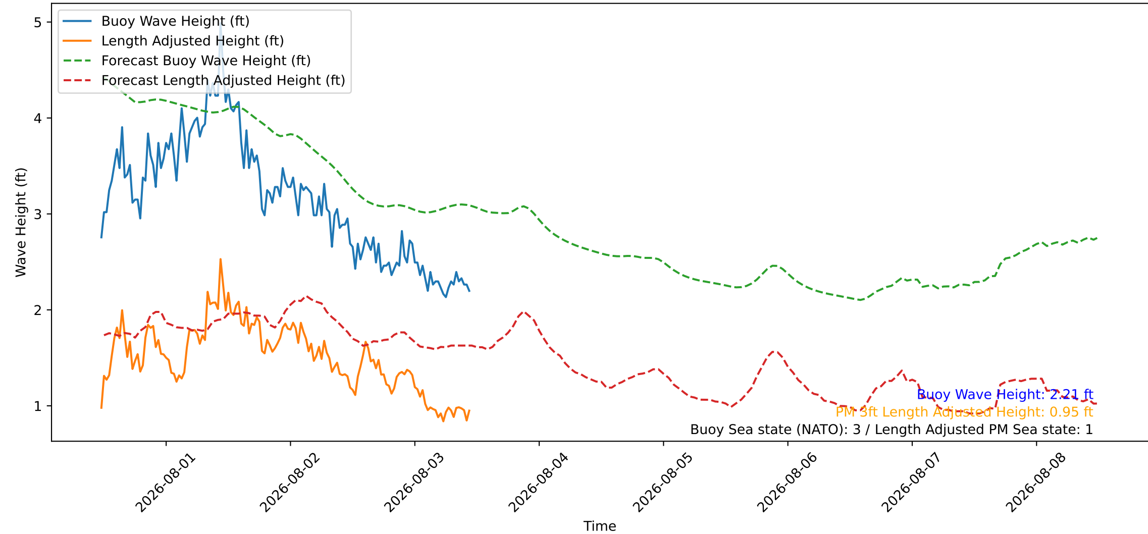
Wave Heights over Time for Green Beach at 2026-08-03 11:31:08
