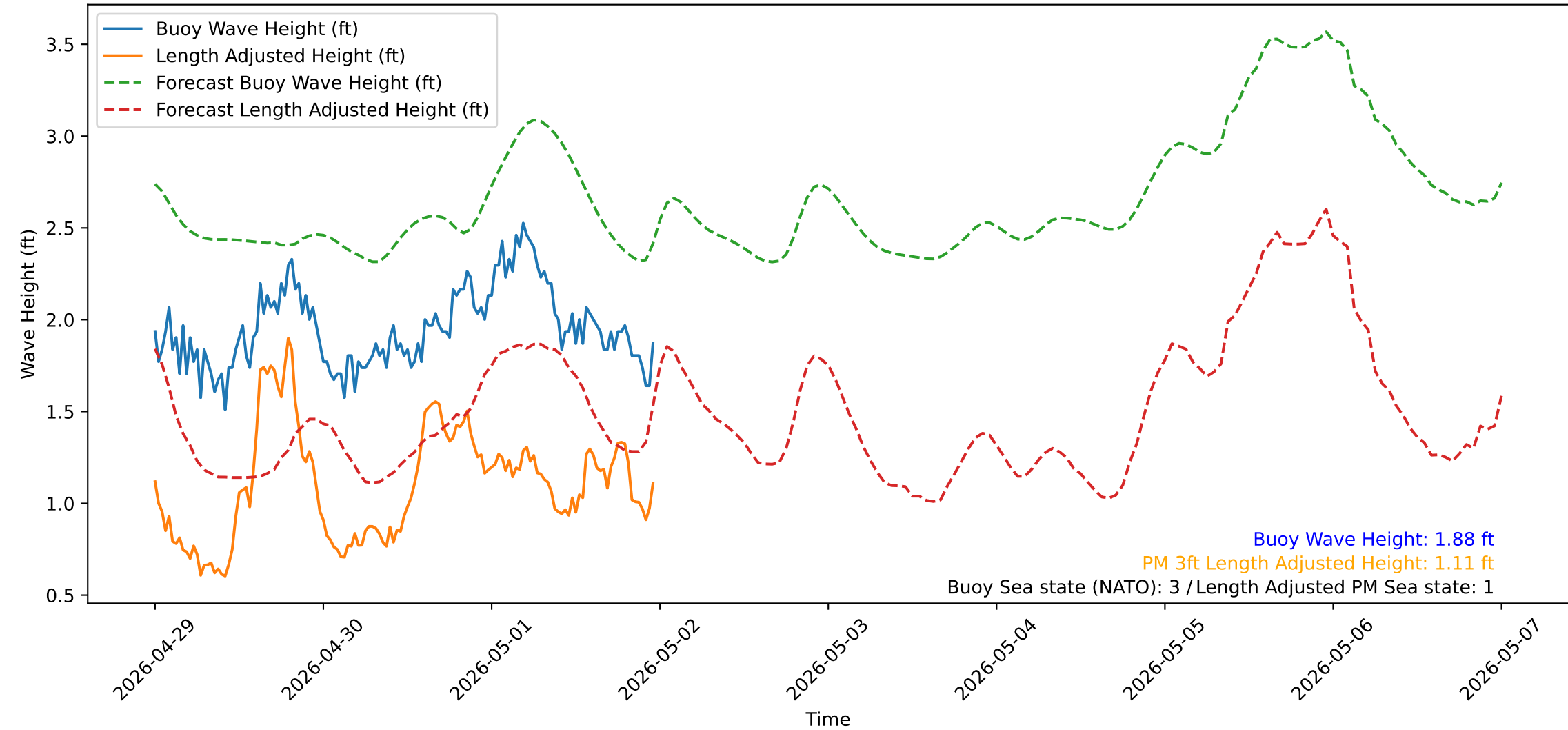
Wave Heights over Time for Red Beach at 2026-05-01 23:50:52
