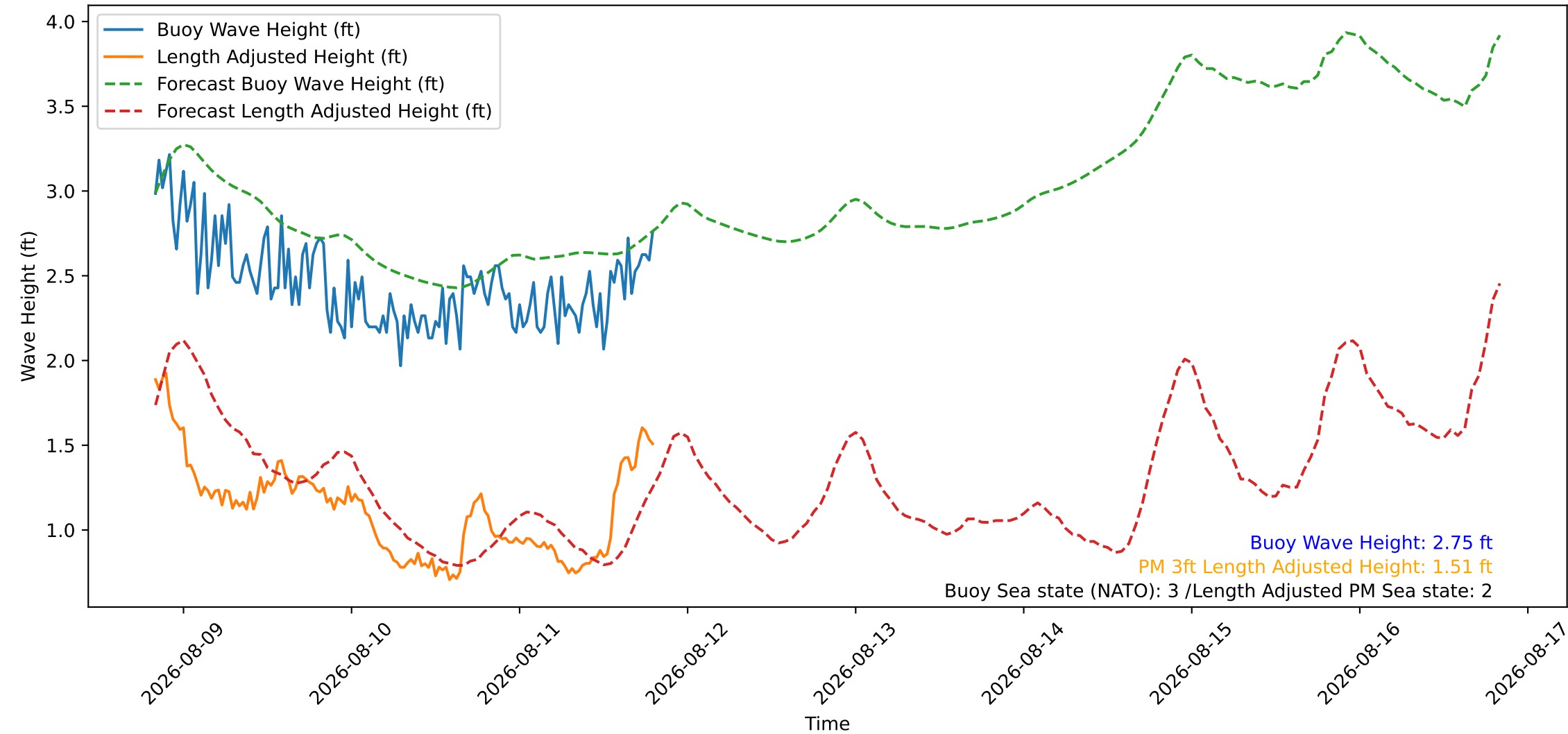
Wave Heights over Time for Oceanside Harbor at 2026-08-11 20:00:26
