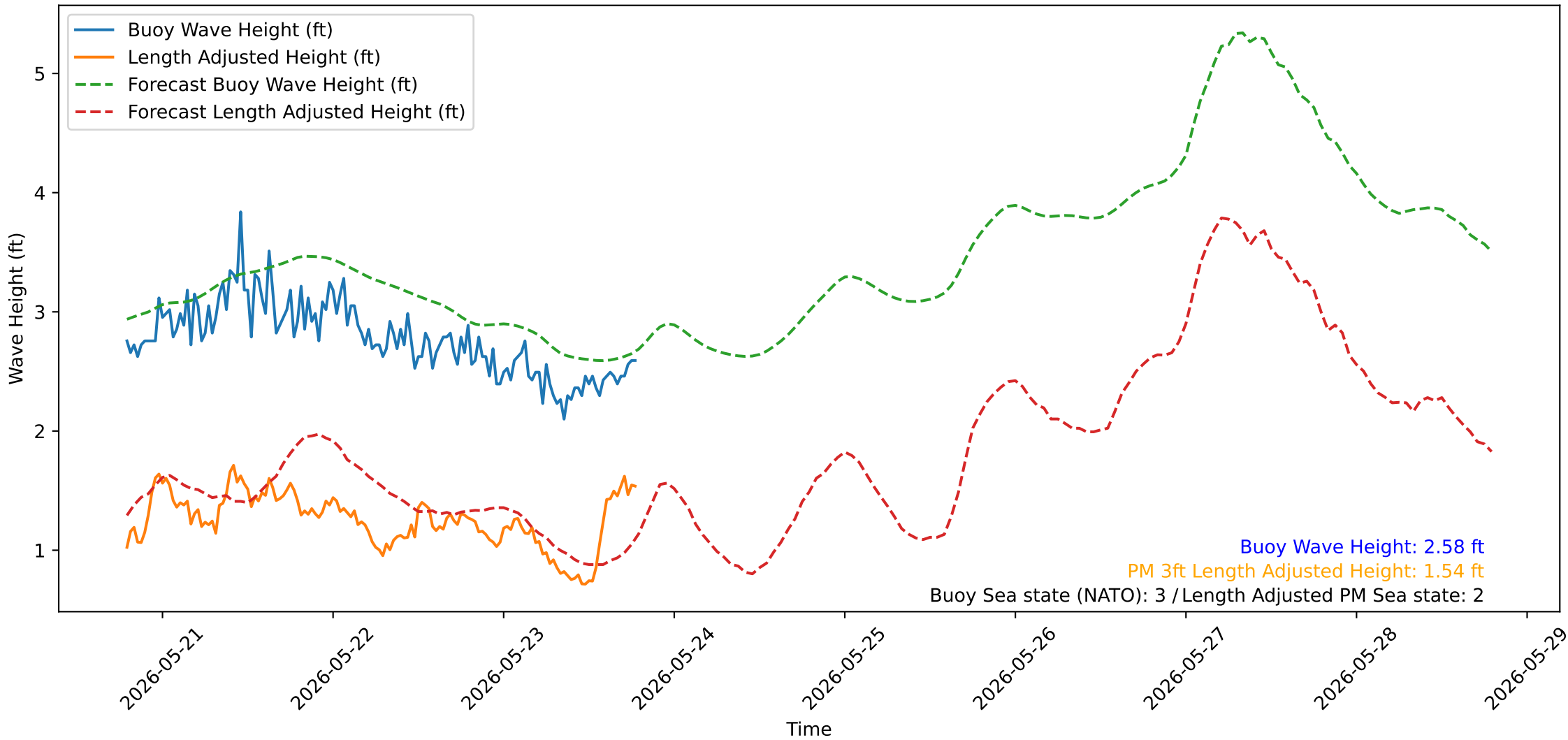
Wave Heights over Time for Oceanside Harbor at 2026-05-23 19:00:31
