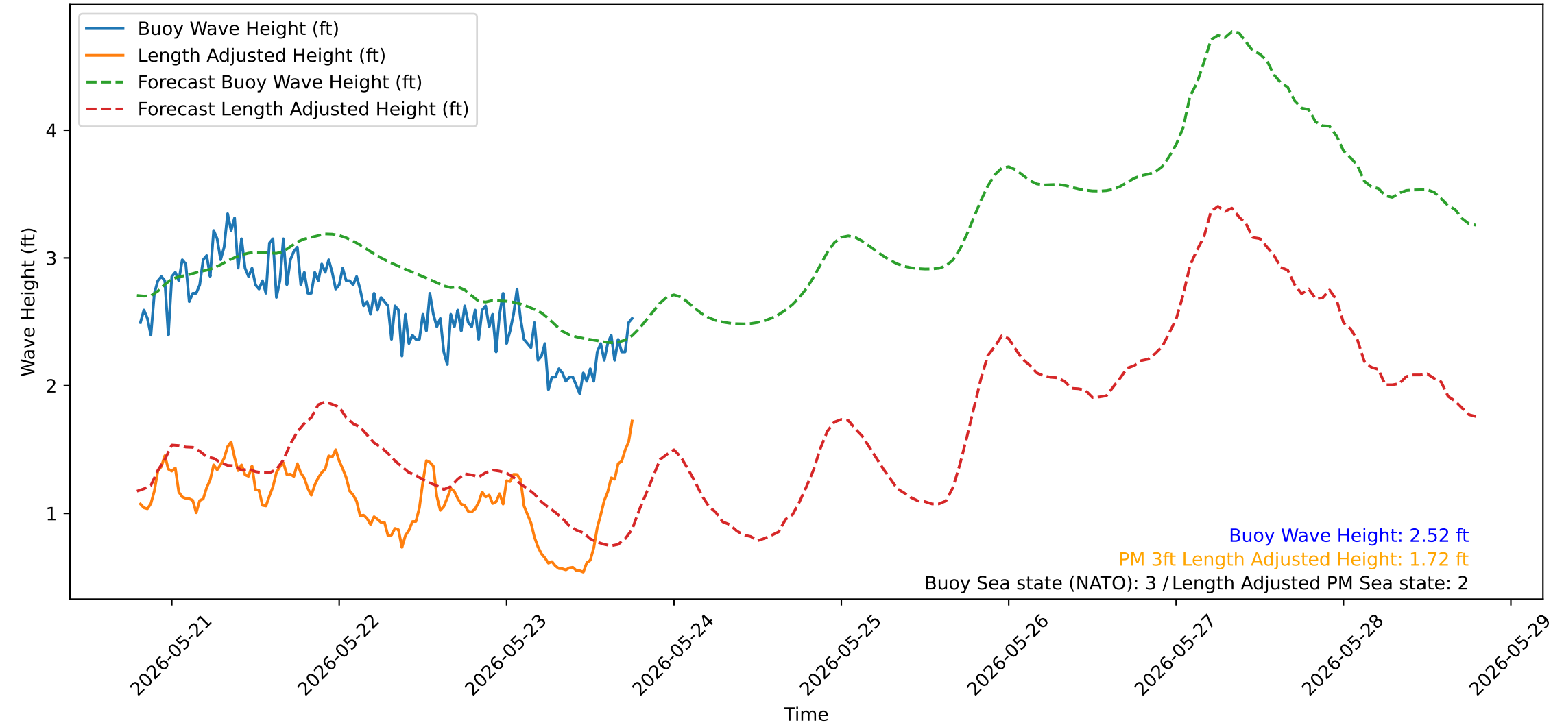
Wave Heights over Time for Red Beach at 2026-05-23 19:00:51
