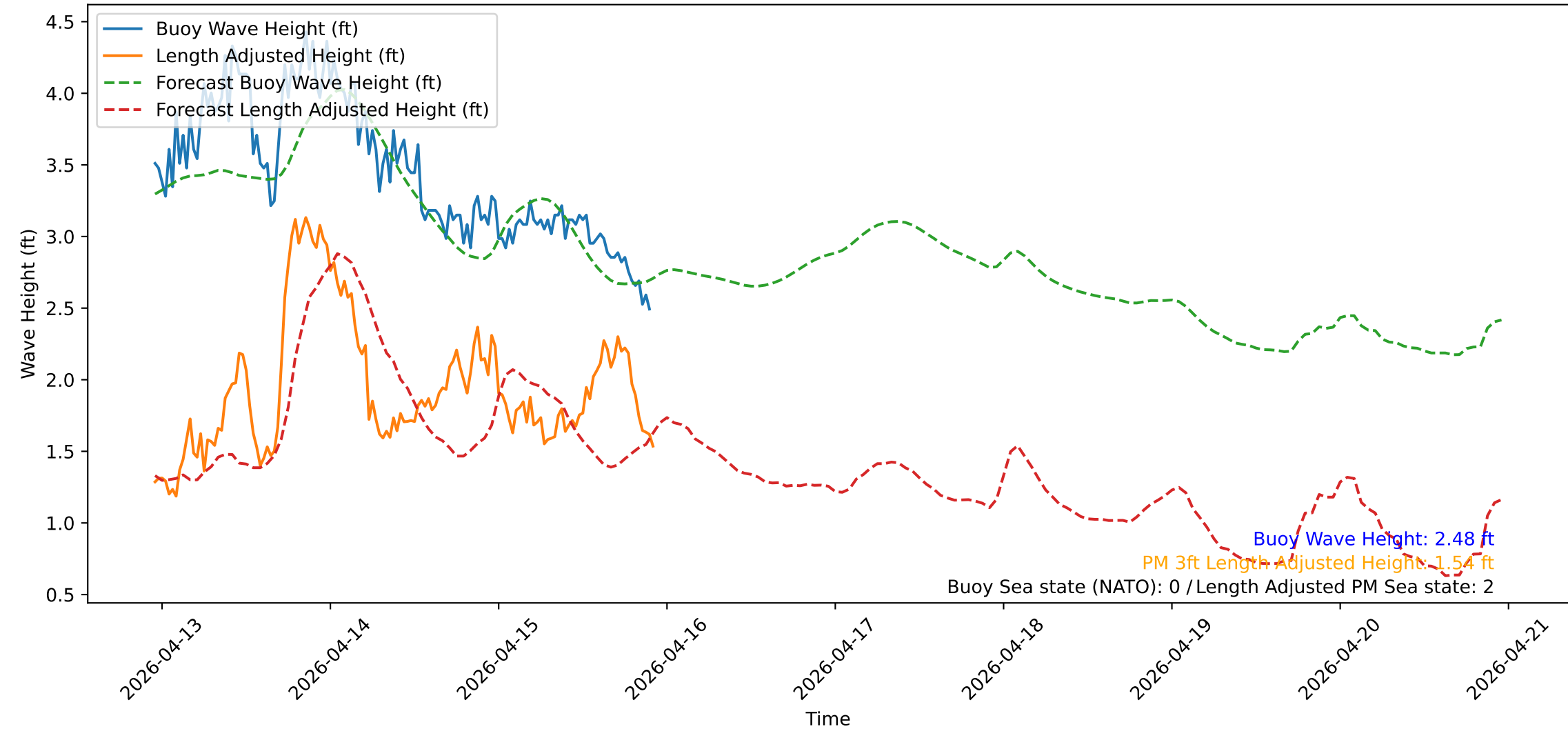
Wave Heights over Time for Red Beach at 2026-04-15 22:40:51
