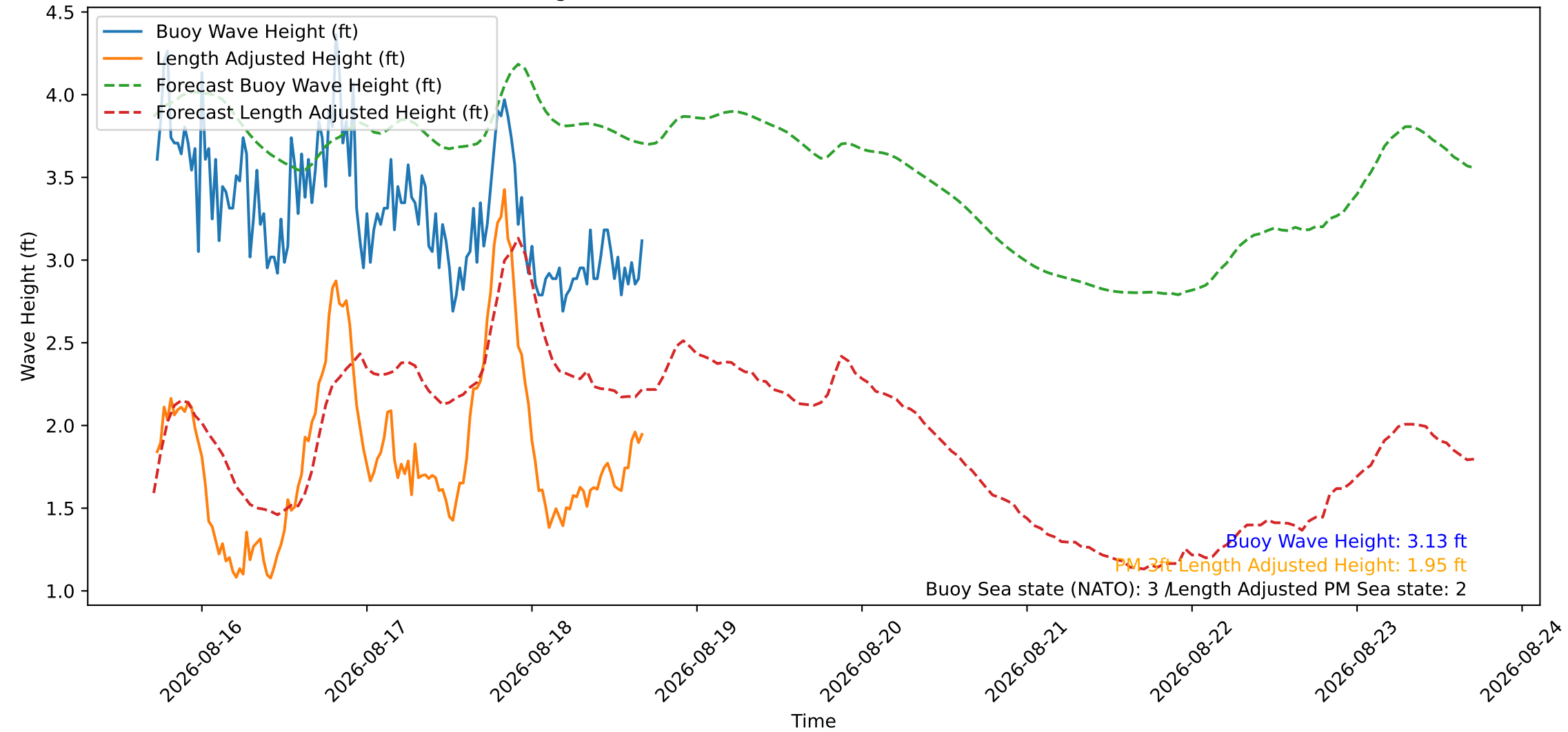
Wave Heights over Time for Green Beach at 2026-08-18 17:01:09
