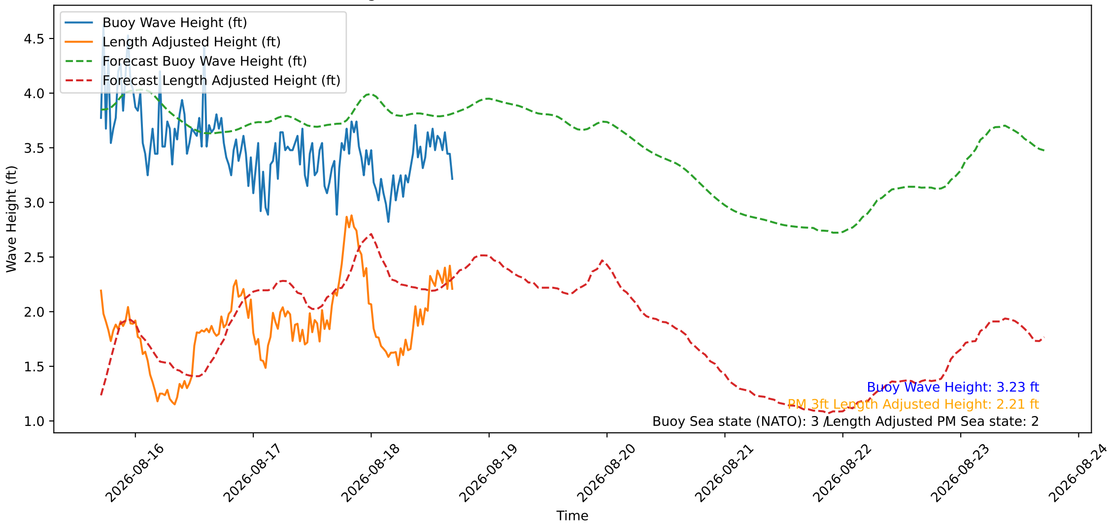
Wave Heights over Time for Oceanside Harbor at 2026-08-18 17:00:26
