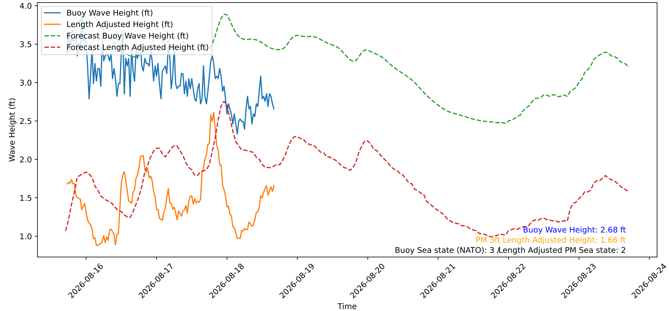
Wave Heights over Time for Red Beach at 2026-08-18 17:00:46
