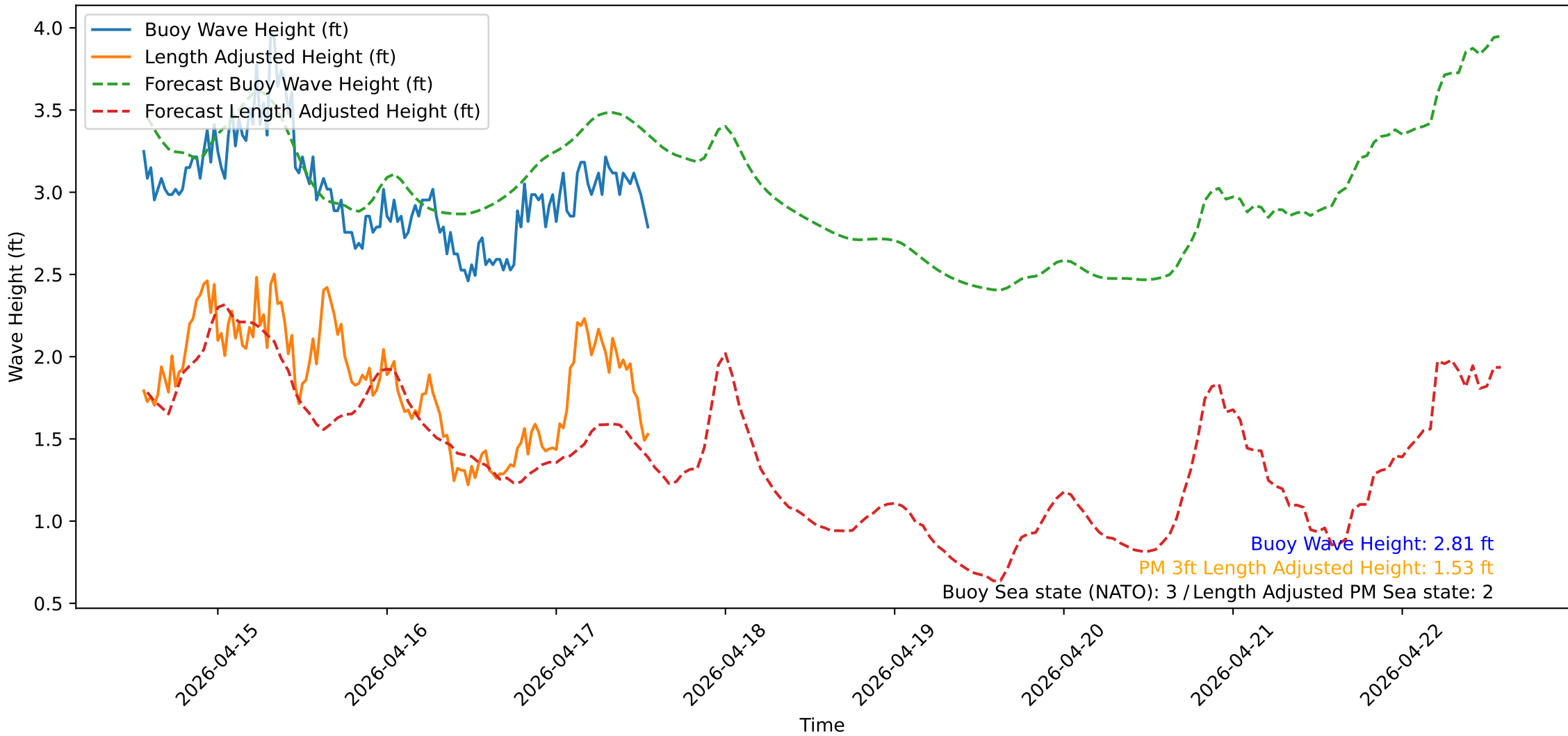
Wave Heights over Time for Green Beach at 2026-04-17 13:41:15
