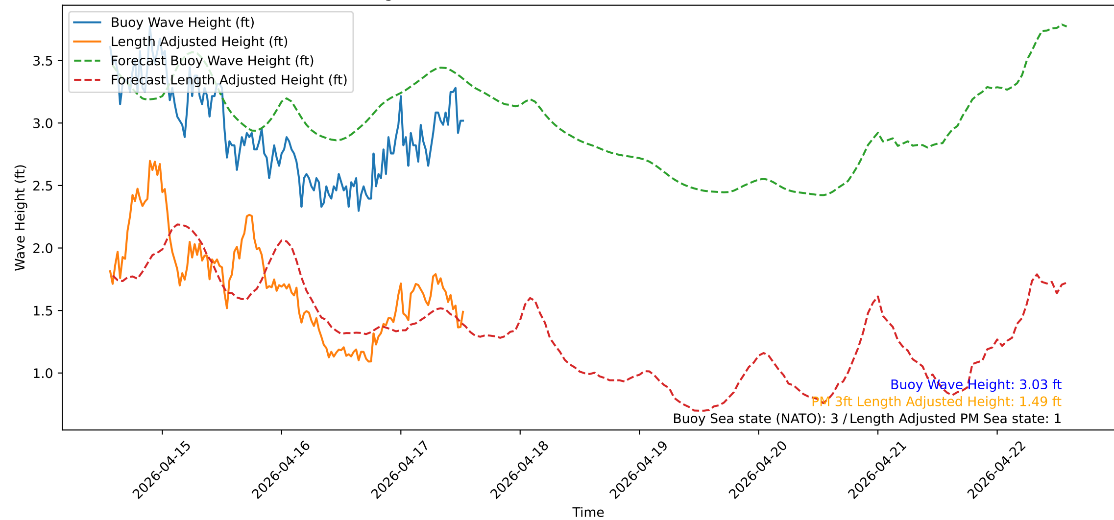
Wave Heights over Time for Oceanside Harbor at 2026-04-17 13:40:33
